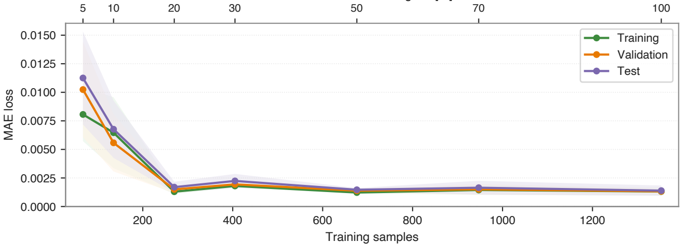
Learning curve for the inverse model
