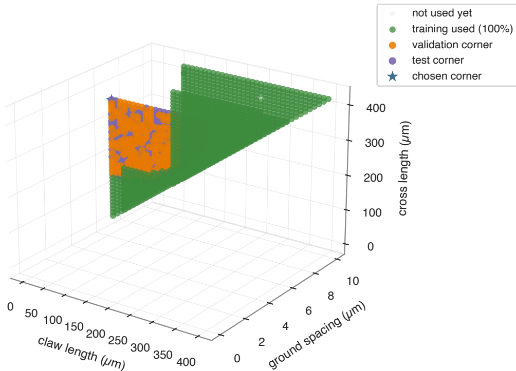
Geometry coverage at 100% training fraction
