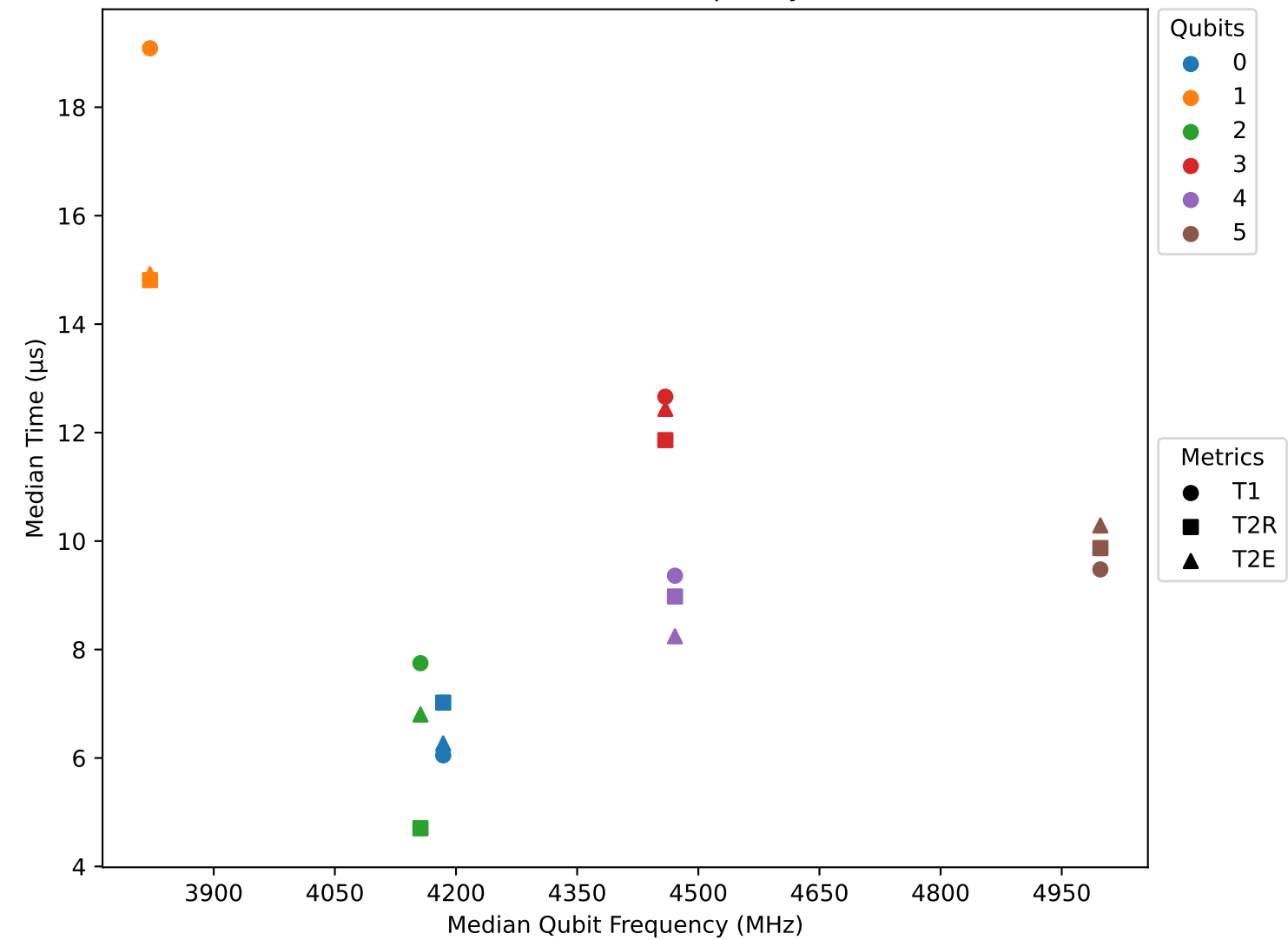
Decoherence vs. Qubit Frequency (Run 1)
