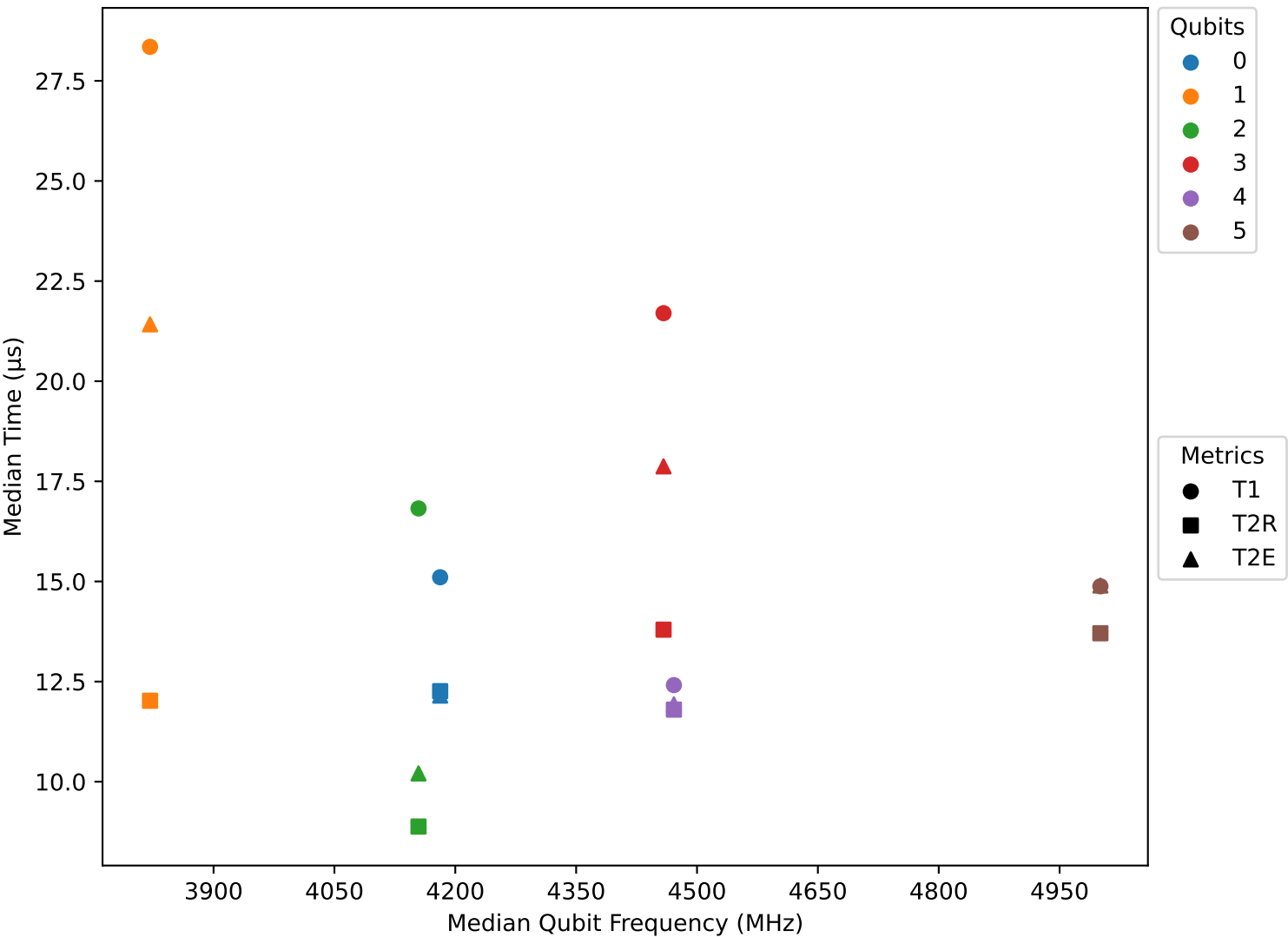
Decoherence vs. Qubit Frequency (Run 3)
