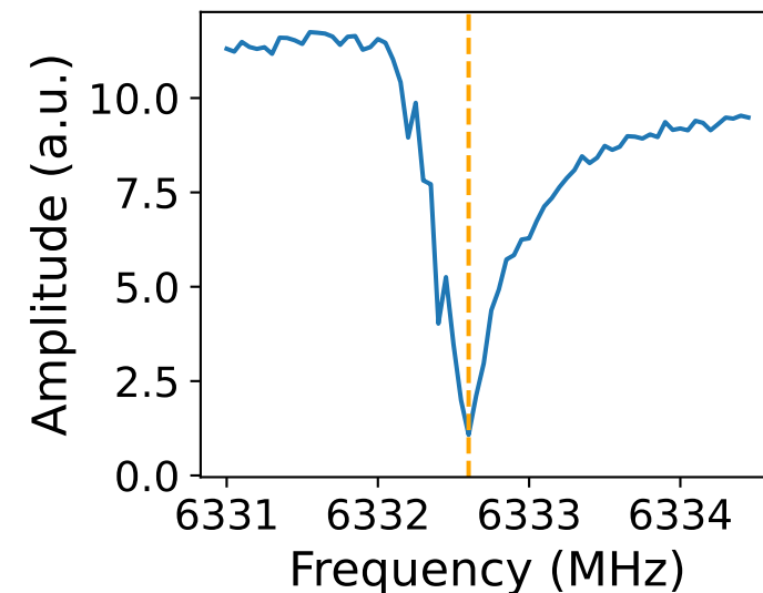
Resonator 3 6332.600 MHz
