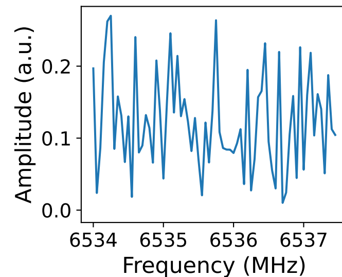
Resonator 6
