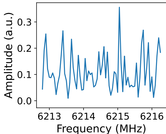
Resonator 1
