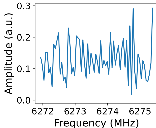
Resonator 2
