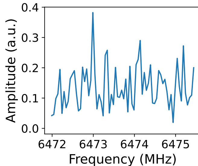
Resonator 5
