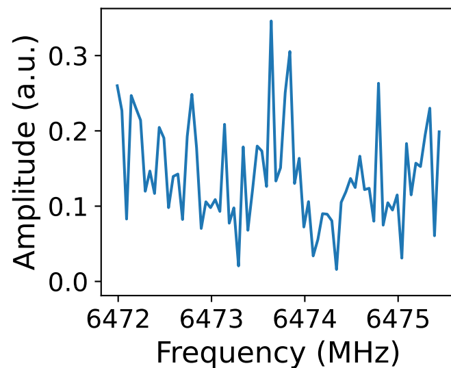
Resonator 5
