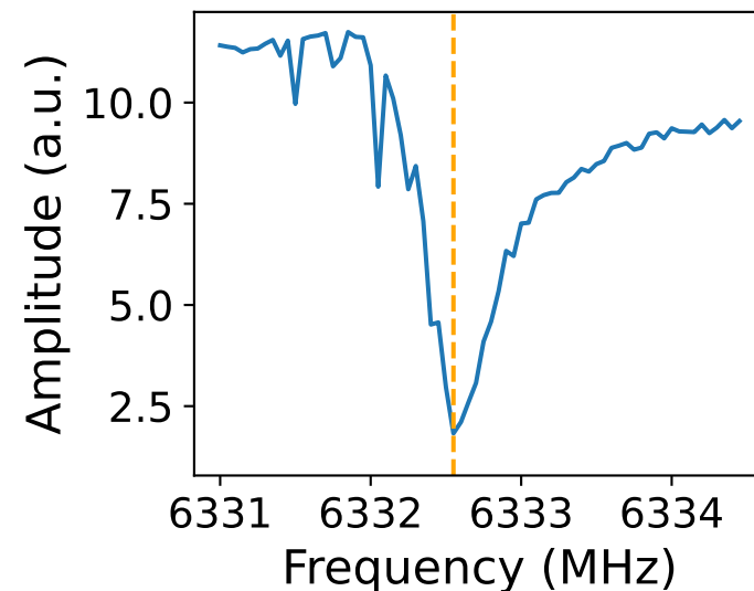
Resonator 3 6332.550 MHz
