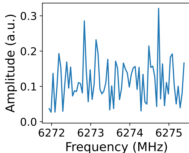
Resonator 2
