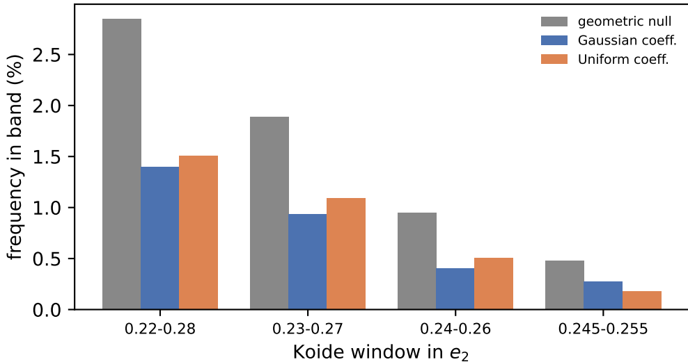
Koide is under-populated vs geometric null (all windows)
