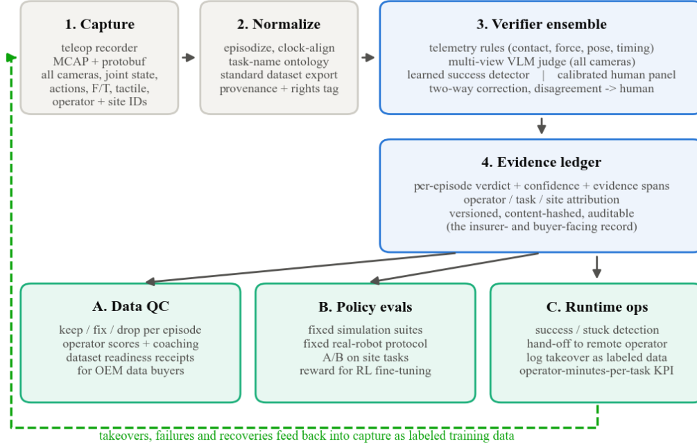
Figure 7: Architecture of the proposed evaluation layer: capture and normalization, a verifier ensemble, an evidence ledger, and three consumers. The dashed path returns takeovers, failures and recoveries to capture as labeled data.
