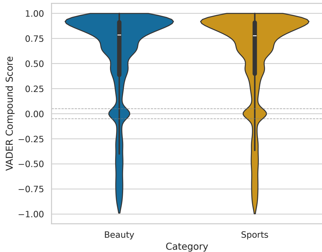
Sentiment Distribution (Violin + Box)
