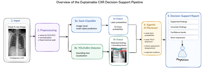
Fig. 1. Locked workflow used in the final repository: chest X-ray image, Swin classification, YOLO localization support, and agentic AI report generation.
