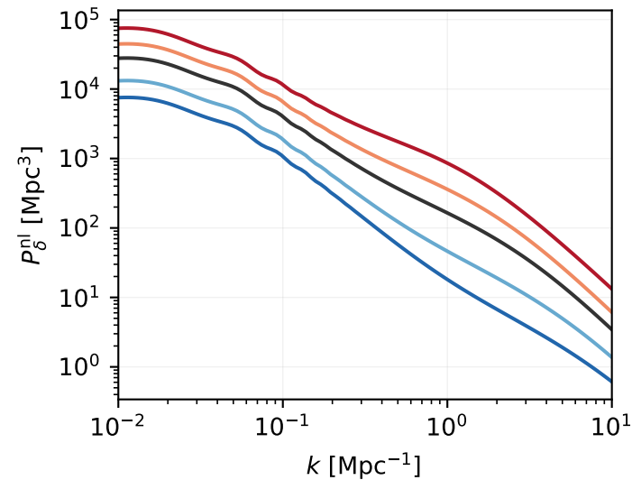
(a) Nonlinear matter
