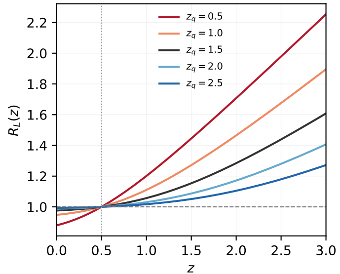
(c) Transition redshift z_q
