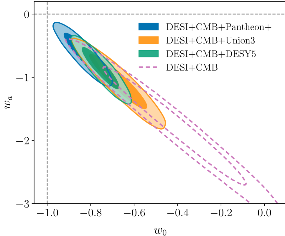
(b) Evolving-dark-energy constraints
