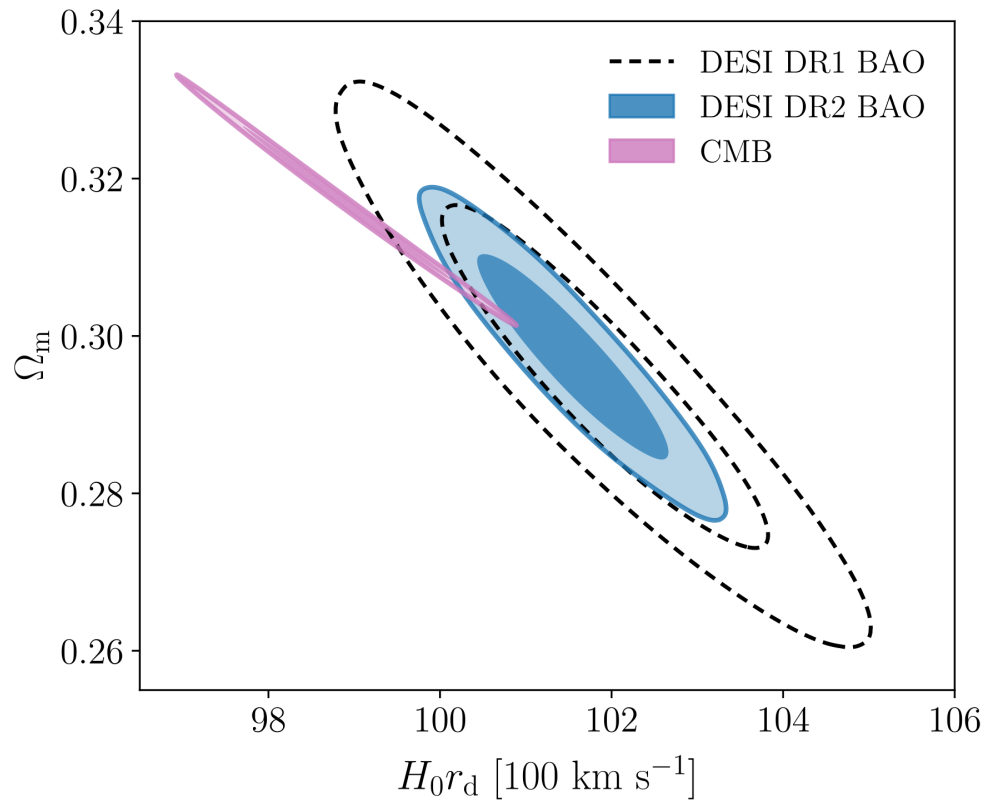
(a) \Lambda CDM constraints
