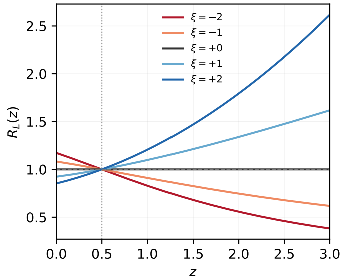
(b) Evolution index \xi
