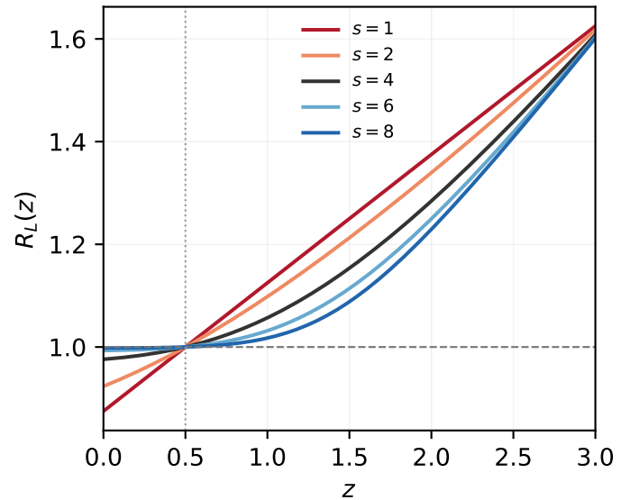
(c) Sharpness s
