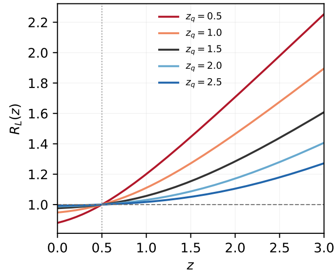
(a) Transition redshift z_q
