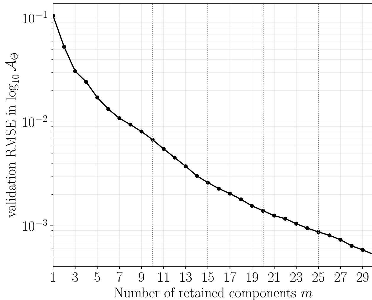
Validation reconstruction error versus PCA rank
