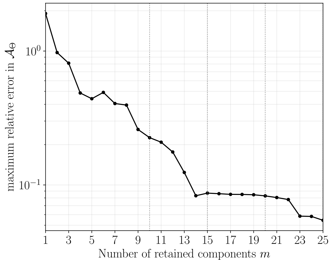
Validation reconstruction error versus PCA rank
