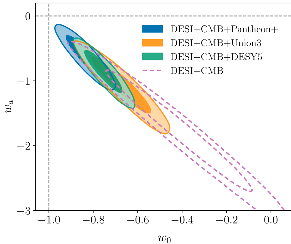
(b) Evolving-dark-energy constraints
