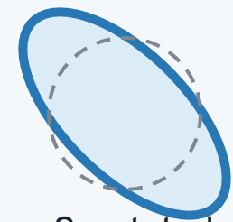
gamma2: rotated shear
