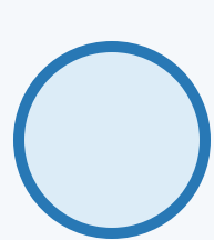
unlensed
