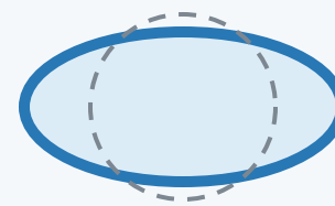
gamma1: horizontal shear
