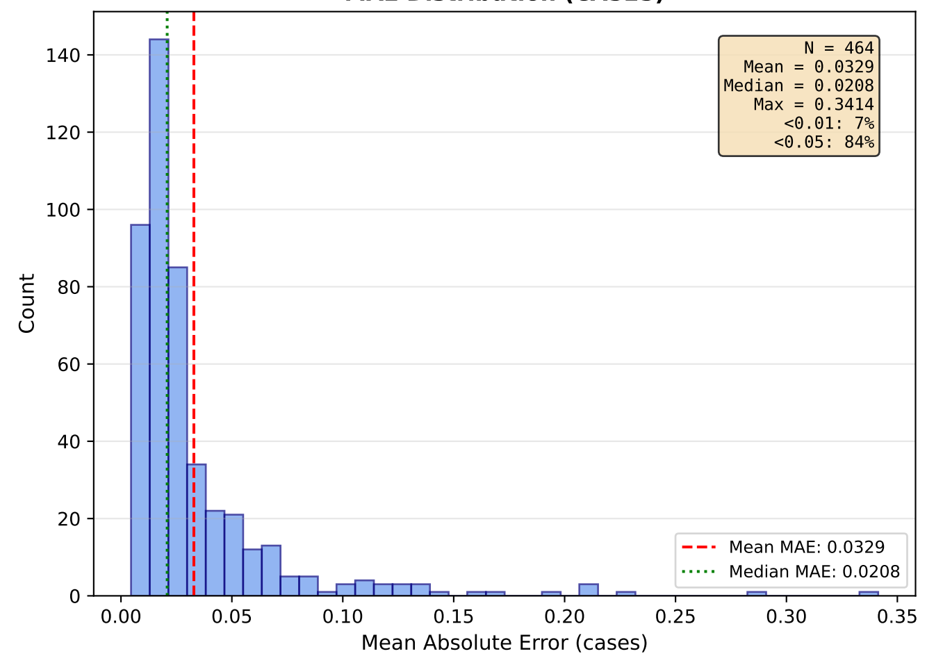
MAE Distribution (CASES)
