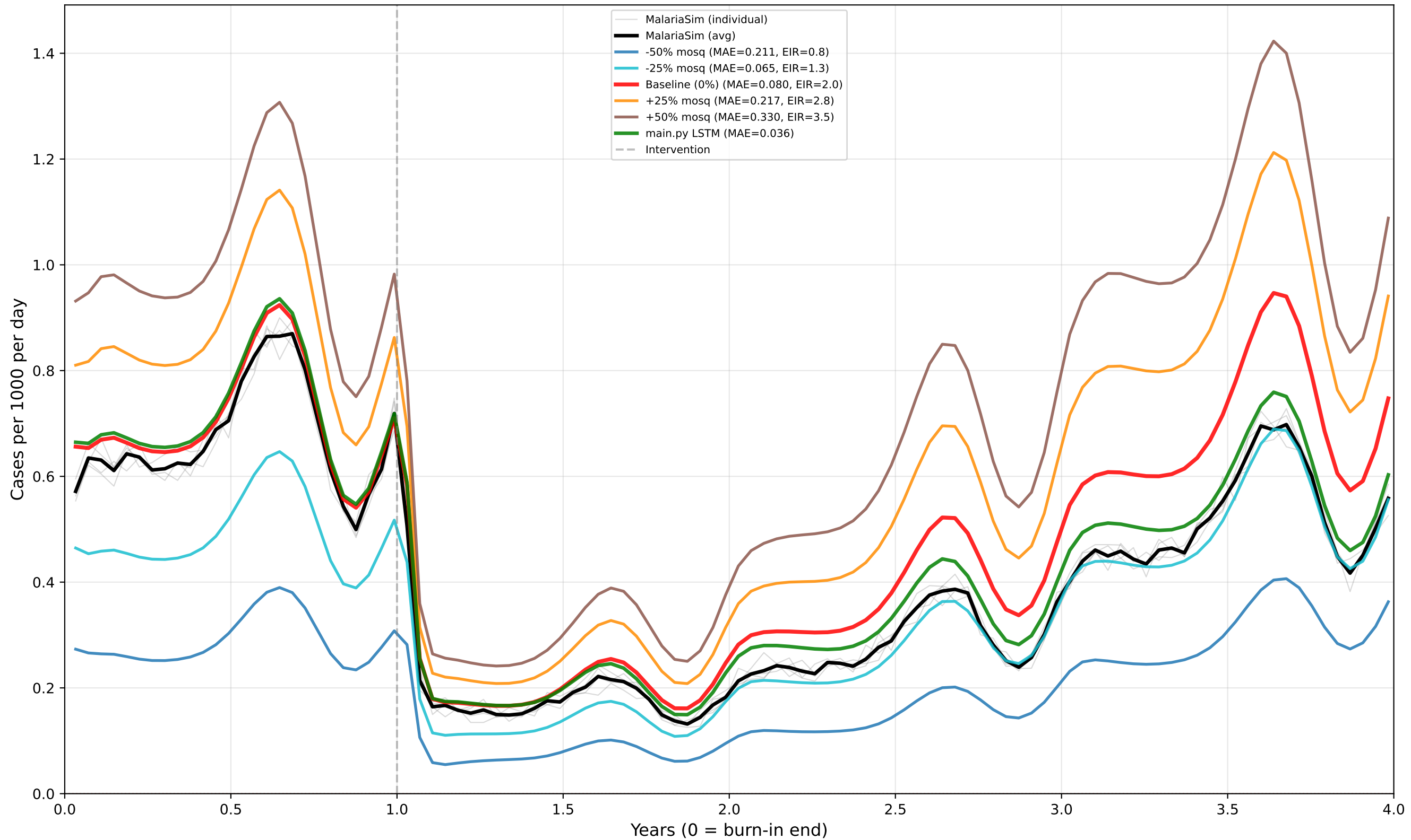
Case 10: Perennial - ITN Only - Low EIR - Mid dn0 Predictor: CASES | True EIR: 2.1 | Est EIR (0%): 2.0 prev_y9: 0.083 | [minte v1.4.0]
