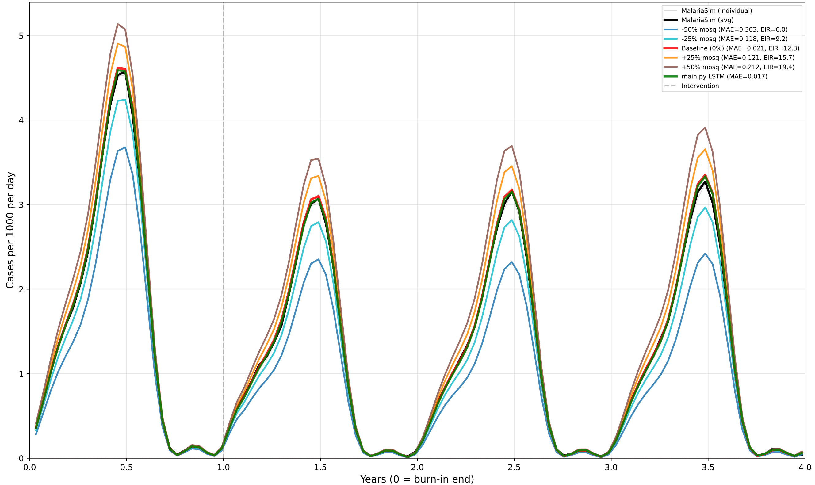
Case 26: Seasonal - LSM Only - Mid EIR Predictor: CASES | True EIR: 12.1 | Est EIR (0%): 12.3 prev_y9: 0.327 | [minte v1.4.0]
