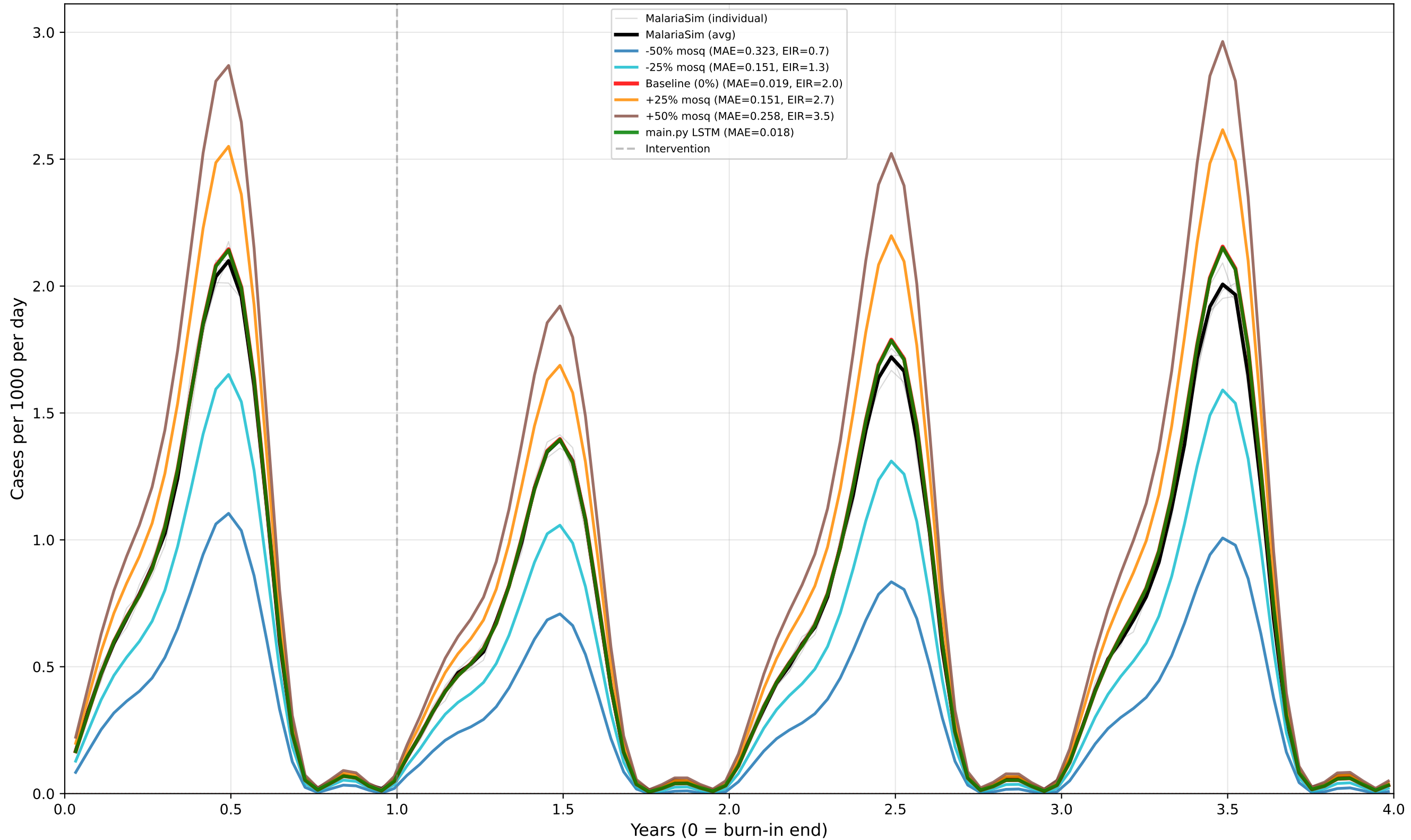
Case 16: Seasonal - ITN Only - Low EIR - Low dn0 Predictor: CASES | True EIR: 2.0 | Est EIR (0%): 2.0 prev_y9: 0.108 | [minte v1.4.0]
