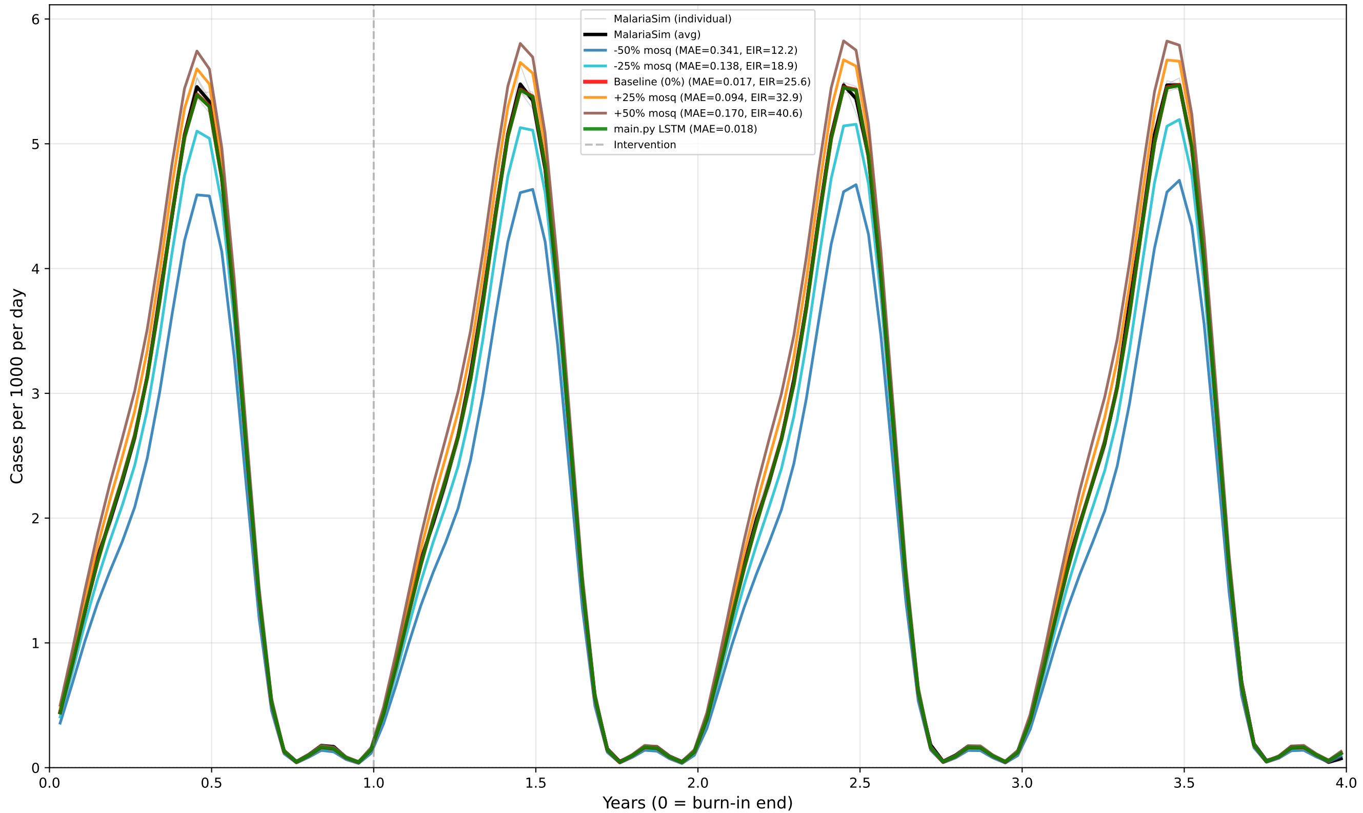
Case 6: Seasonal - No Intervention - High EIR Predictor: CASES | True EIR: 25.4 | Est EIR (0%): 25.6 prev_y9: 0.449 | [minte v1.4.0]
