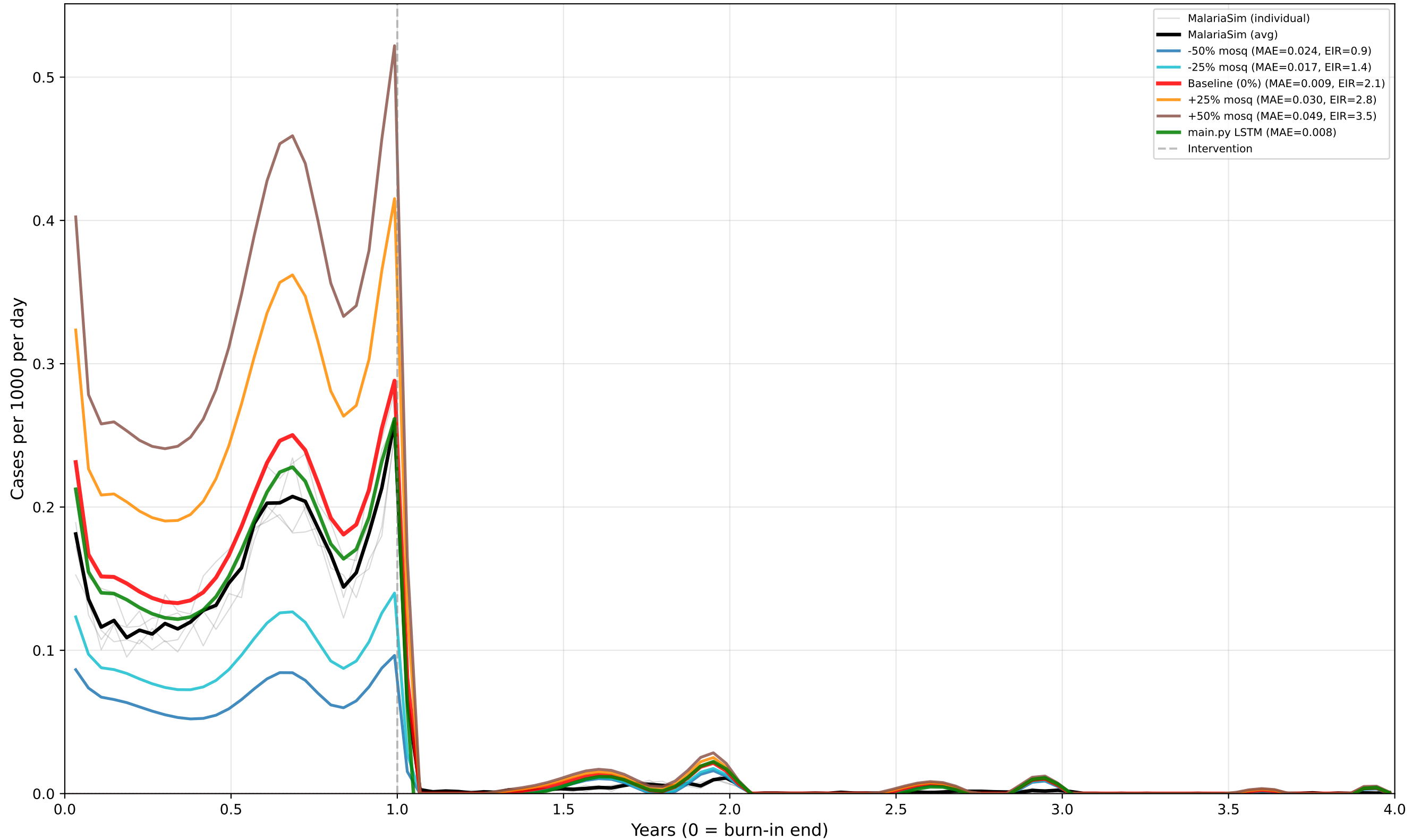
Case 35: Perennial - IRS+LSM - Low EIR Predictor: CASES | True EIR: 2.0 | Est EIR (0%): 2.1 prev_y9: 0.021 | [minte v1.4.0]
