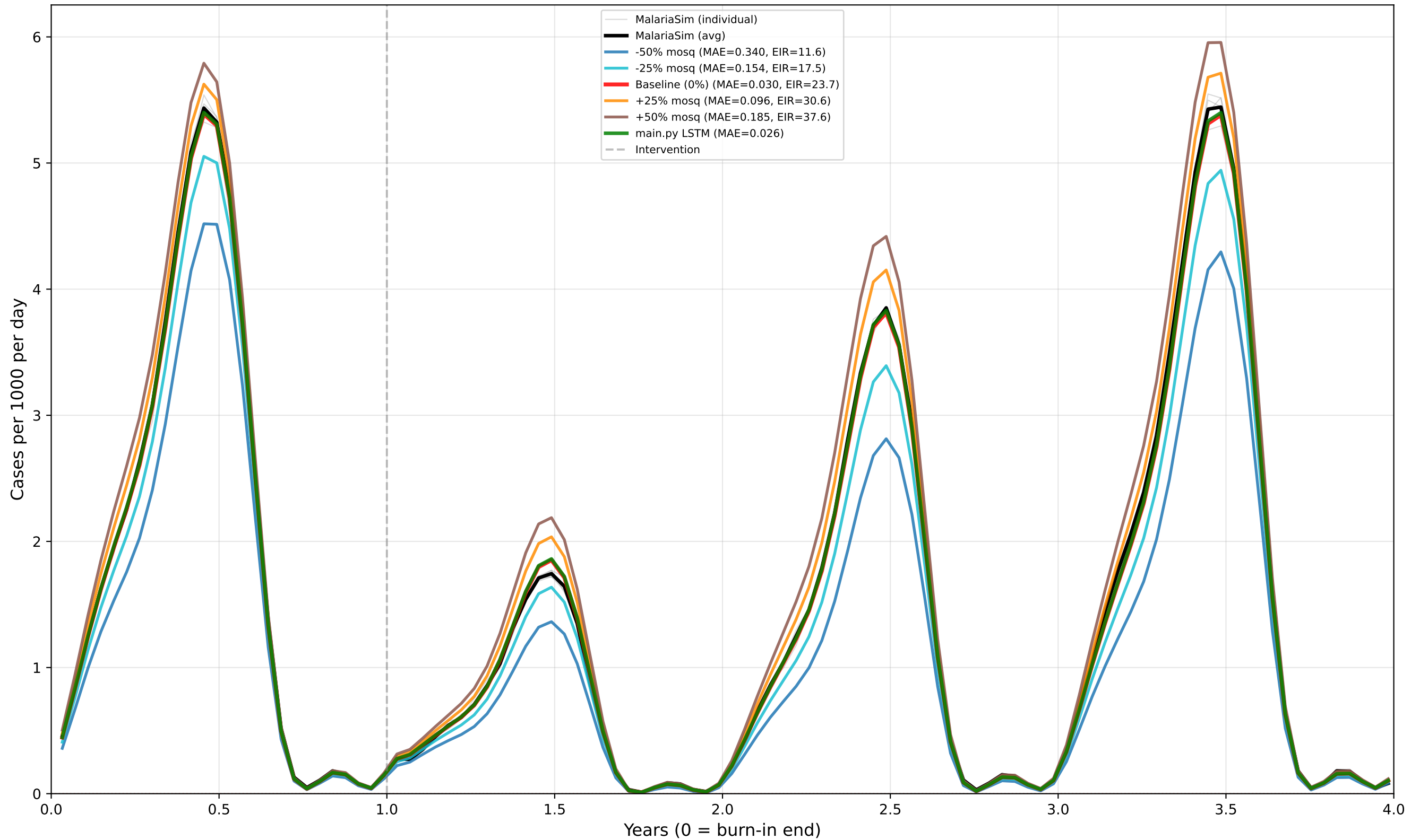
Case 18: Seasonal - ITN Only - High EIR - High dn0 Predictor: CASES | True EIR: 24.1 | Est EIR (0%): 23.7 prev_y9: 0.423 | [minte v1.4.0]
