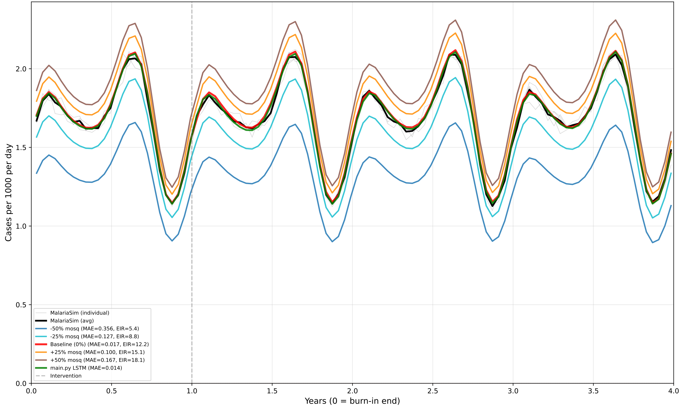
Case 2: Perennial - No Intervention - Mid EIR Predictor: CASES | True EIR: 12.0 | Est EIR (0%): 12.2 prev_y9: 0.362 | [minte v1.4.0]
