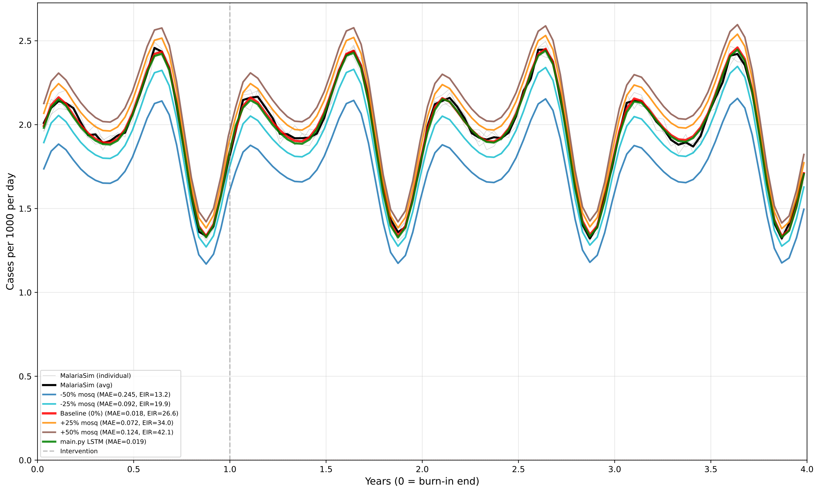
Case 3: Perennial - No Intervention - High EIR Predictor: CASES | True EIR: 25.7 | Est EIR (0%): 26.6 prev_y9: 0.498 | [minte v1.4.0]
