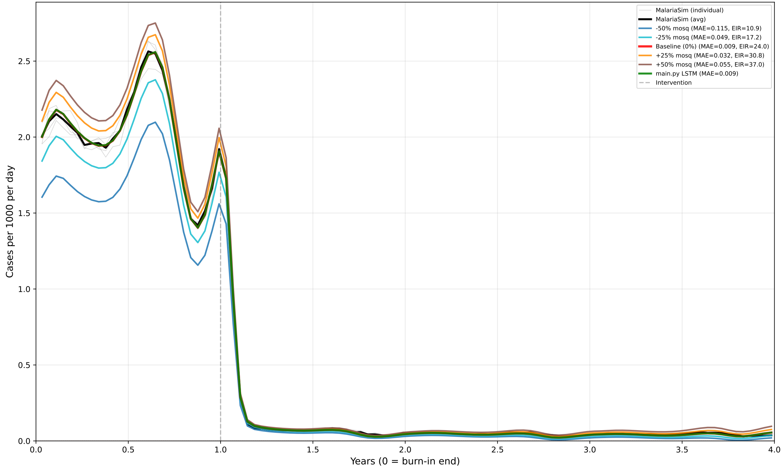
Case 33: Perennial - ITN+LSM - High EIR - High dn0 Predictor: CASES | True EIR: 24.1 | Est EIR (0%): 24.0 prev_y9: 0.440 | [minte v1.4.0]
