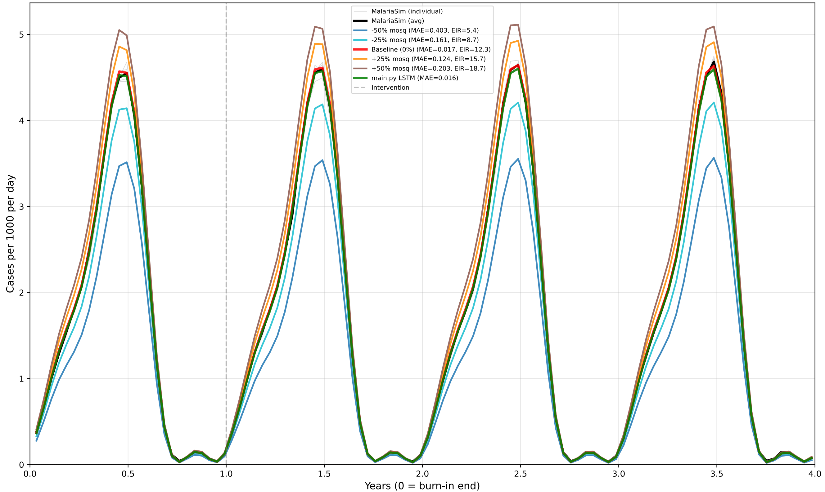
Case 5: Seasonal - No Intervention - Mid EIR Predictor: CASES | True EIR: 11.9 | Est EIR (0%): 12.3 prev_y9: 0.329 | [minte v1.4.0]
