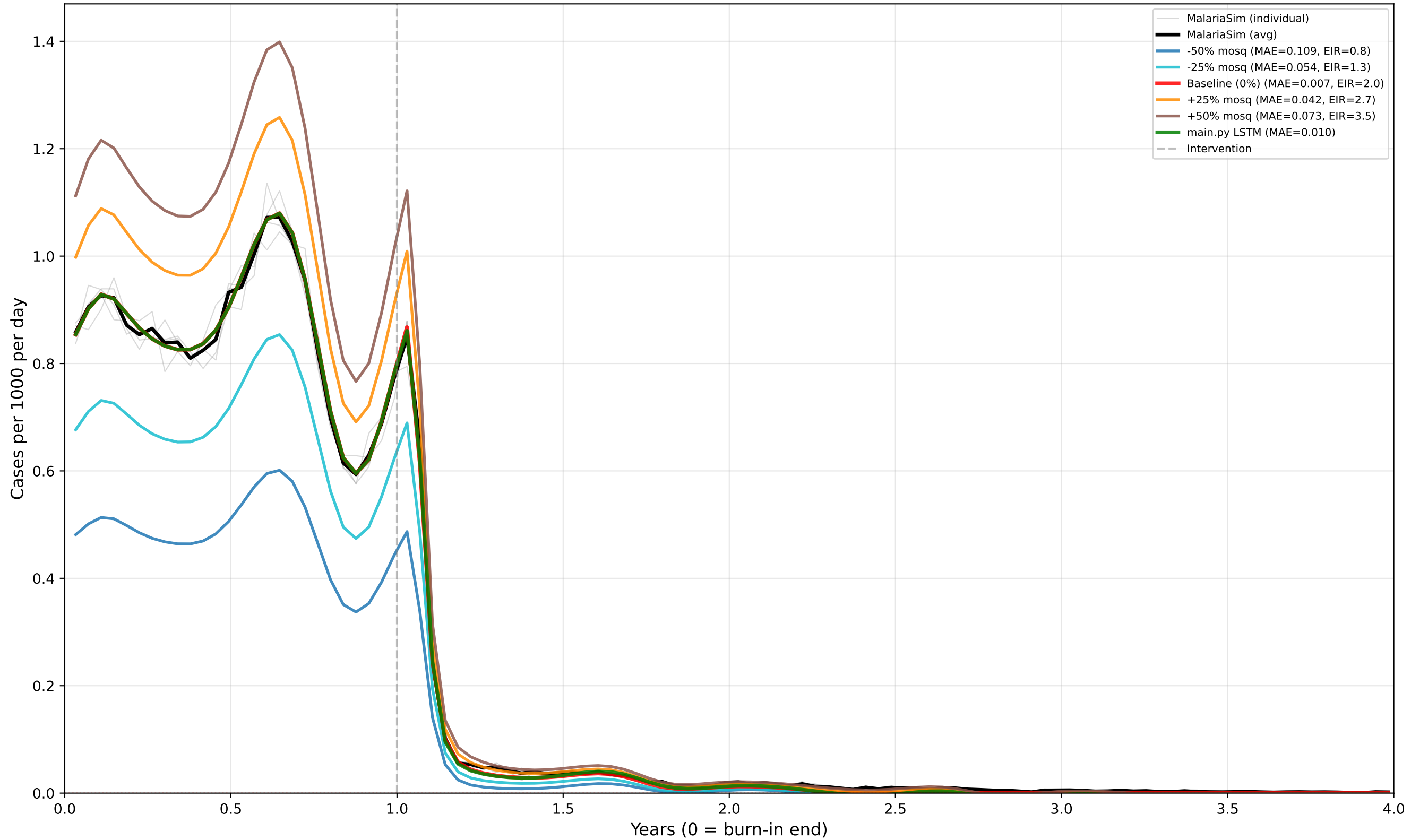
Case 23: Perennial - LSM Only - Low EIR Predictor: CASES | True EIR: 2.0 | Est EIR (0%): 2.0 prev_y9: 0.124 | [minte v1.4.0]
