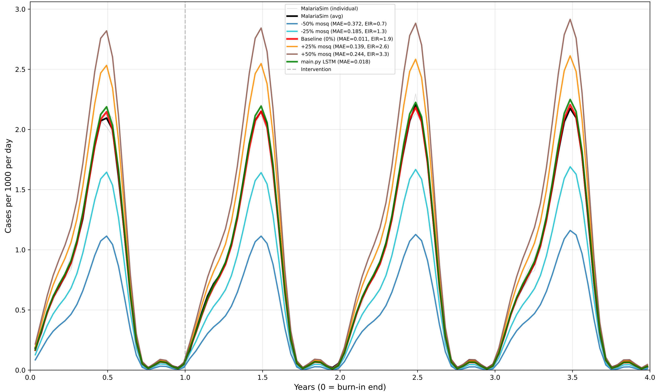
Case 4: Seasonal - No Intervention - Low EIR Predictor: CASES | True EIR: 2.0 | Est EIR (0%): 1.9 prev_y9: 0.107 | [minte v1.4.0]
