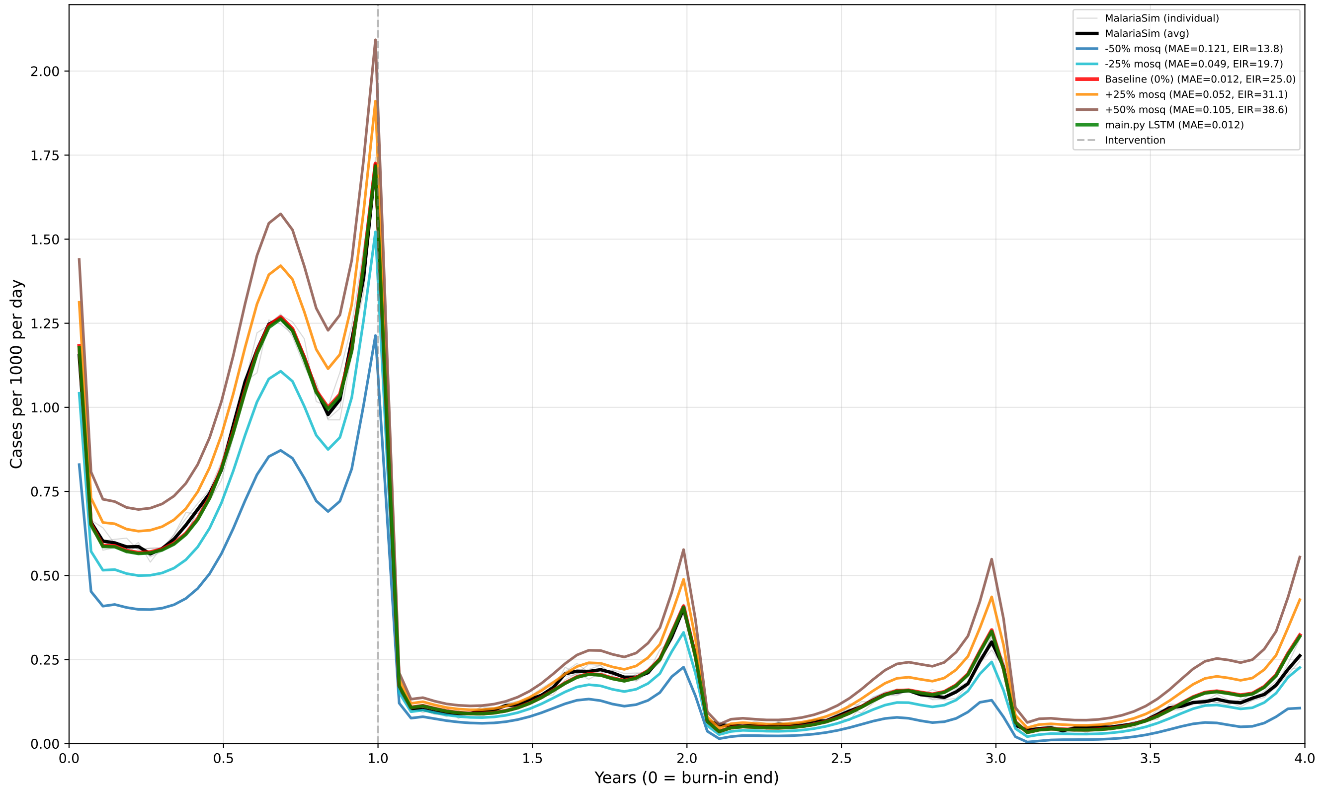
Case 37: Perennial - IRS+LSM - High EIR Predictor: CASES | True EIR: 24.8 | Est EIR (0%): 25.0 prev_y9: 0.226 | [minte v1.4.0]
