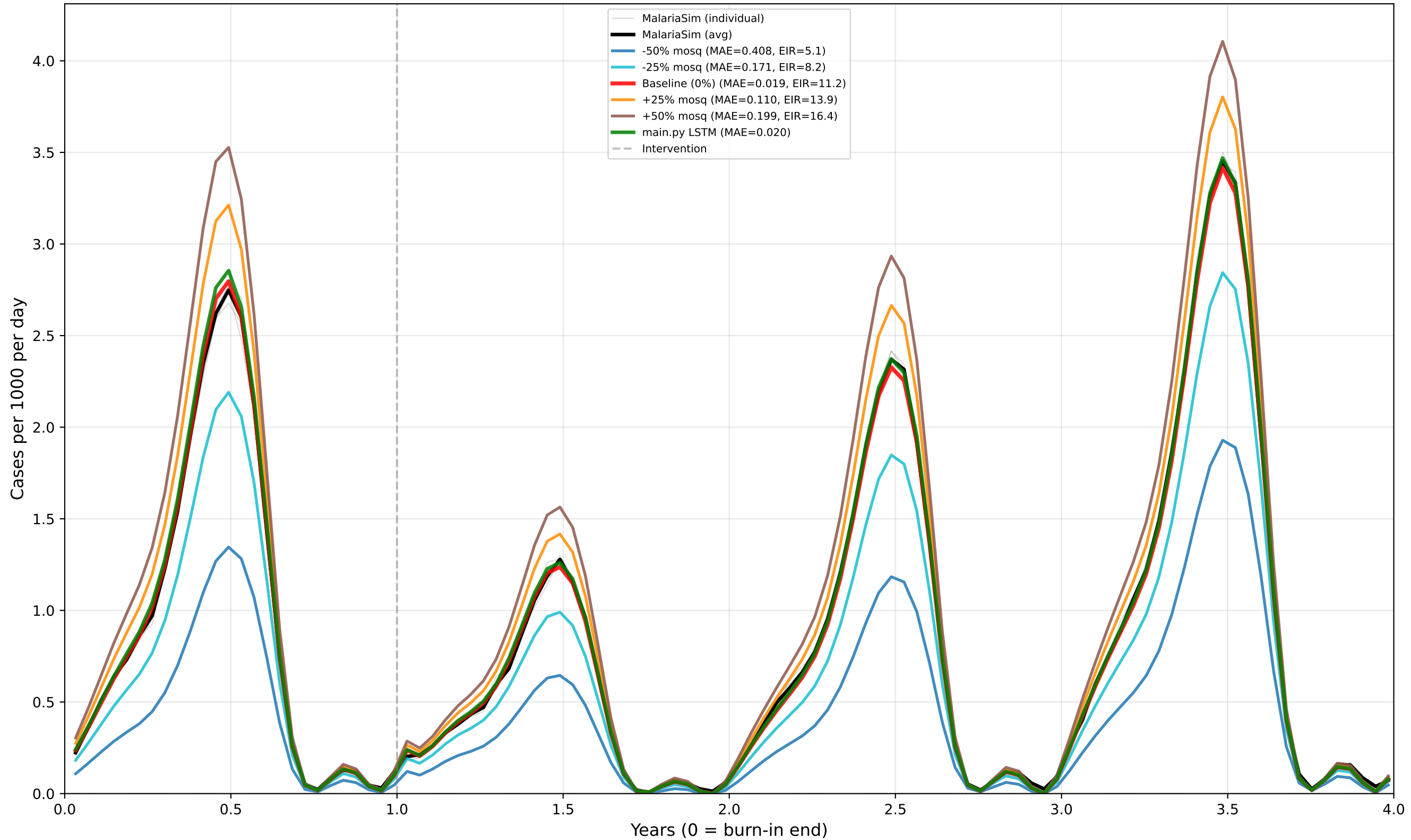
Case 30: Seasonal - ITN+IRS - Mid EIR - Mid dn0 Predictor: CASES | True EIR: 11.5 | Est EIR (0%): 11.2 prev_y9: 0.153 | [minte v1.4.0]
