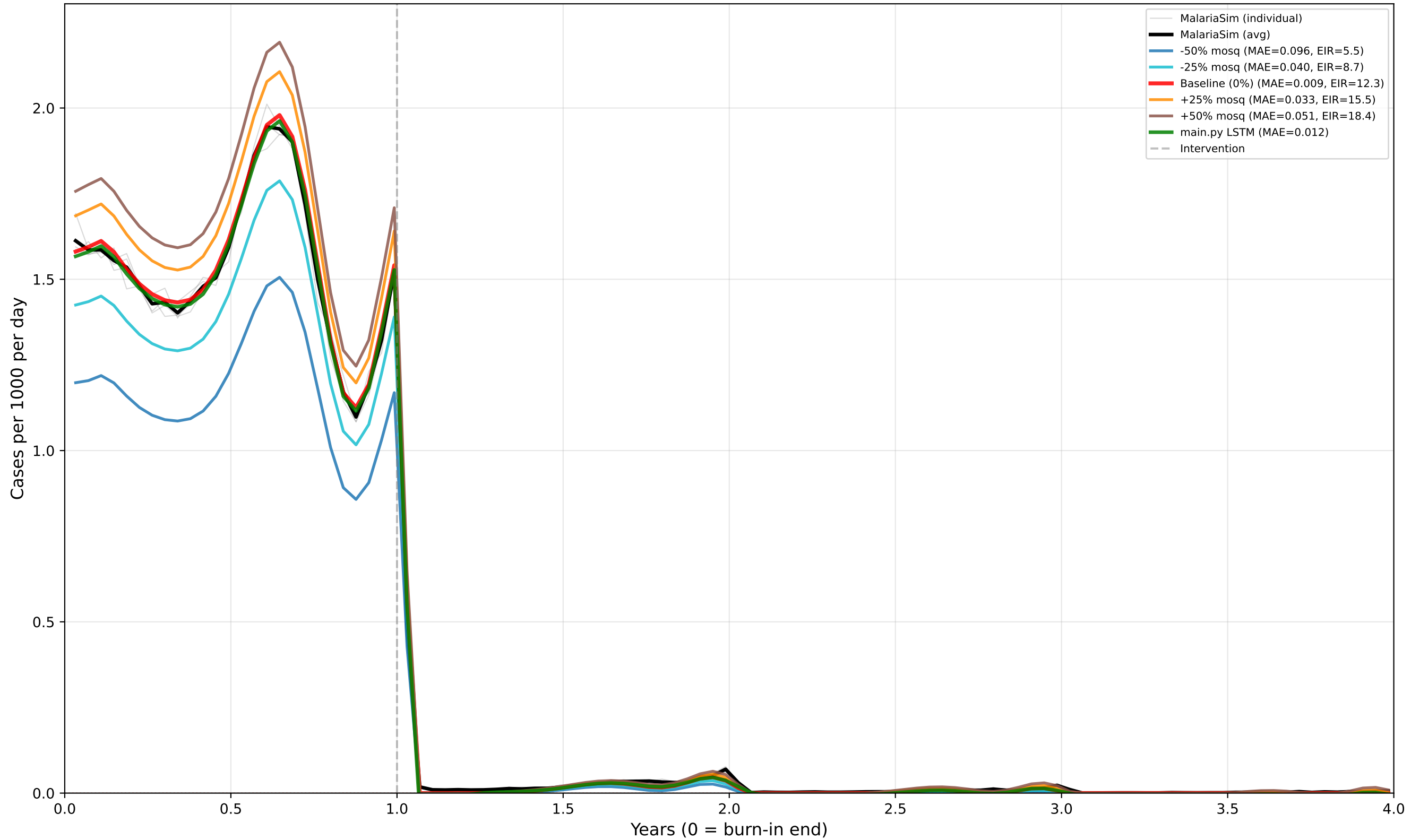
Case 36: Perennial - IRS+LSM - Mid EIR Predictor: CASES | True EIR: 11.9 | Est EIR (0%): 12.3 prev_y9: 0.328 | [minte v1.4.0]
