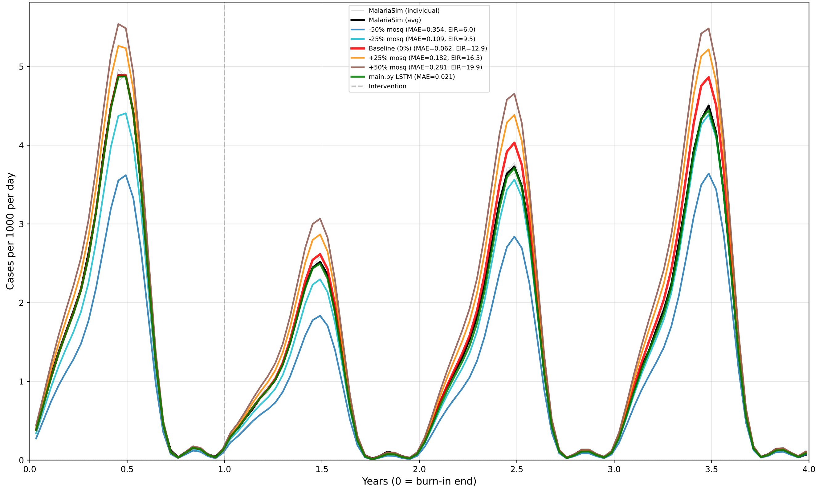
Case 34: Seasonal - ITN+LSM - Mid EIR - Mid dn0 Predictor: CASES | True EIR: 12.8 | Est EIR (0%): 12.9 prev_y9: 0.308 | [minte v1.4.0]
