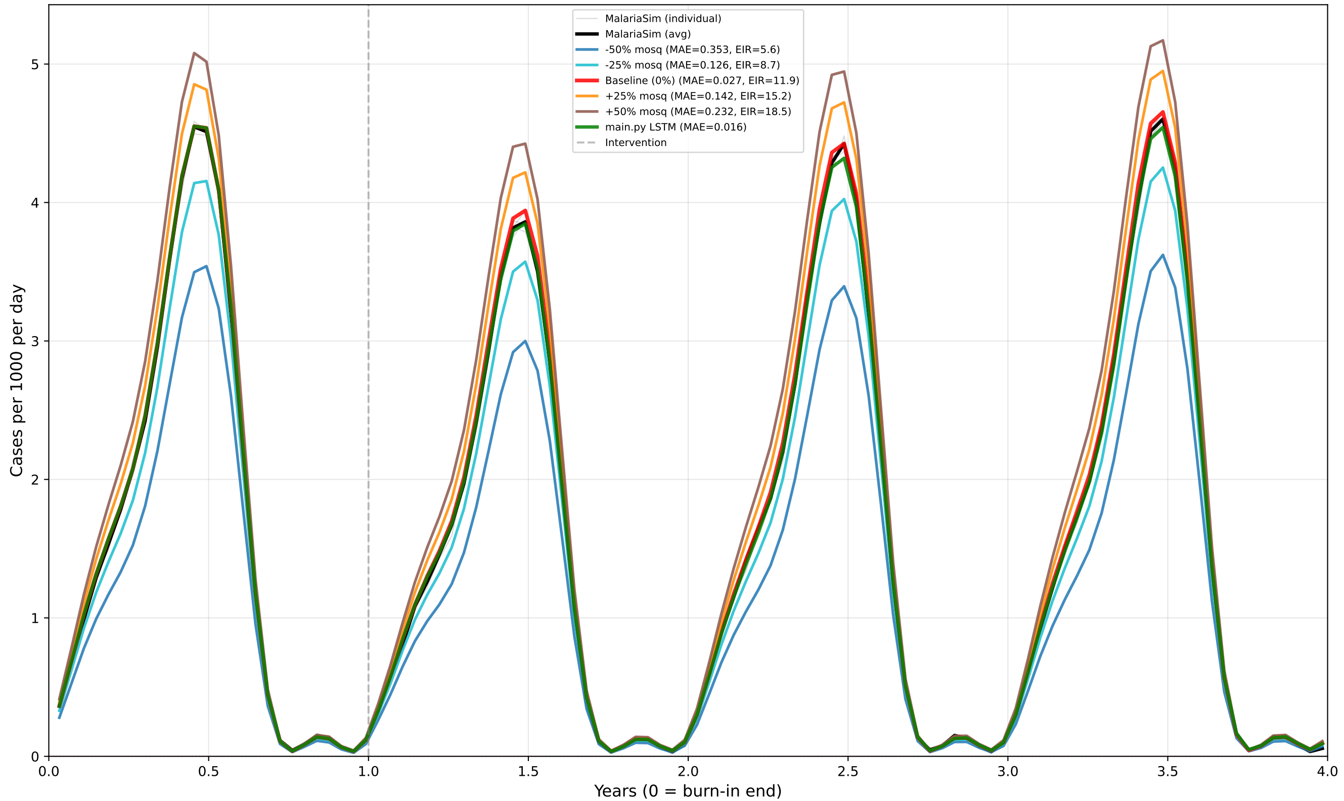
Case 17: Seasonal - ITN Only - Mid EIR - Mid dn0 Predictor: CASES | True EIR: 11.9 | Est EIR (0%): 11.9 prev_y9: 0.321 | [minte v1.4.0]
