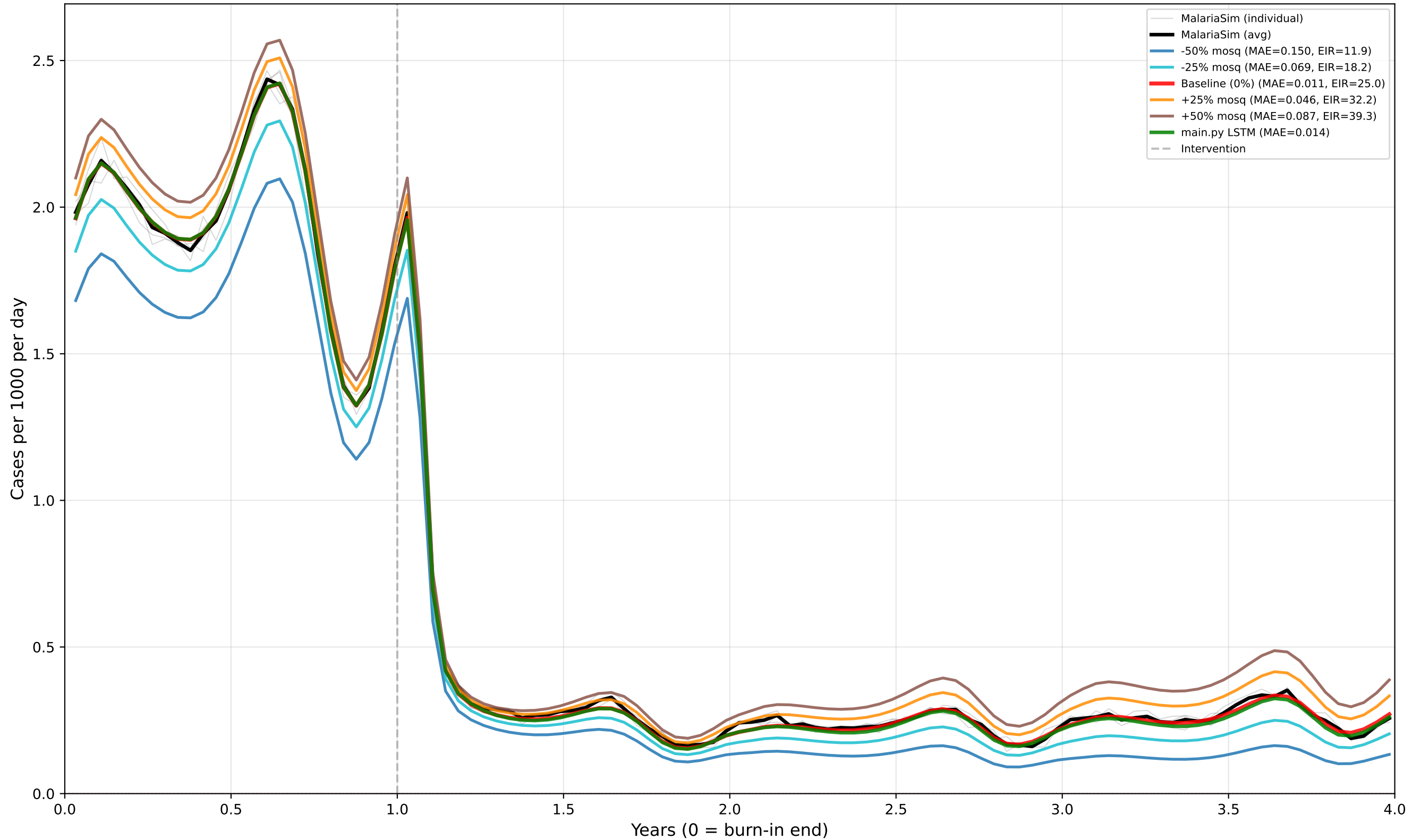
Case 25: Perennial - LSM Only - High EIR Predictor: CASES | True EIR: 25.0 | Est EIR (0%): 25.0 prev_y9: 0.491 | [minte v1.4.0]
