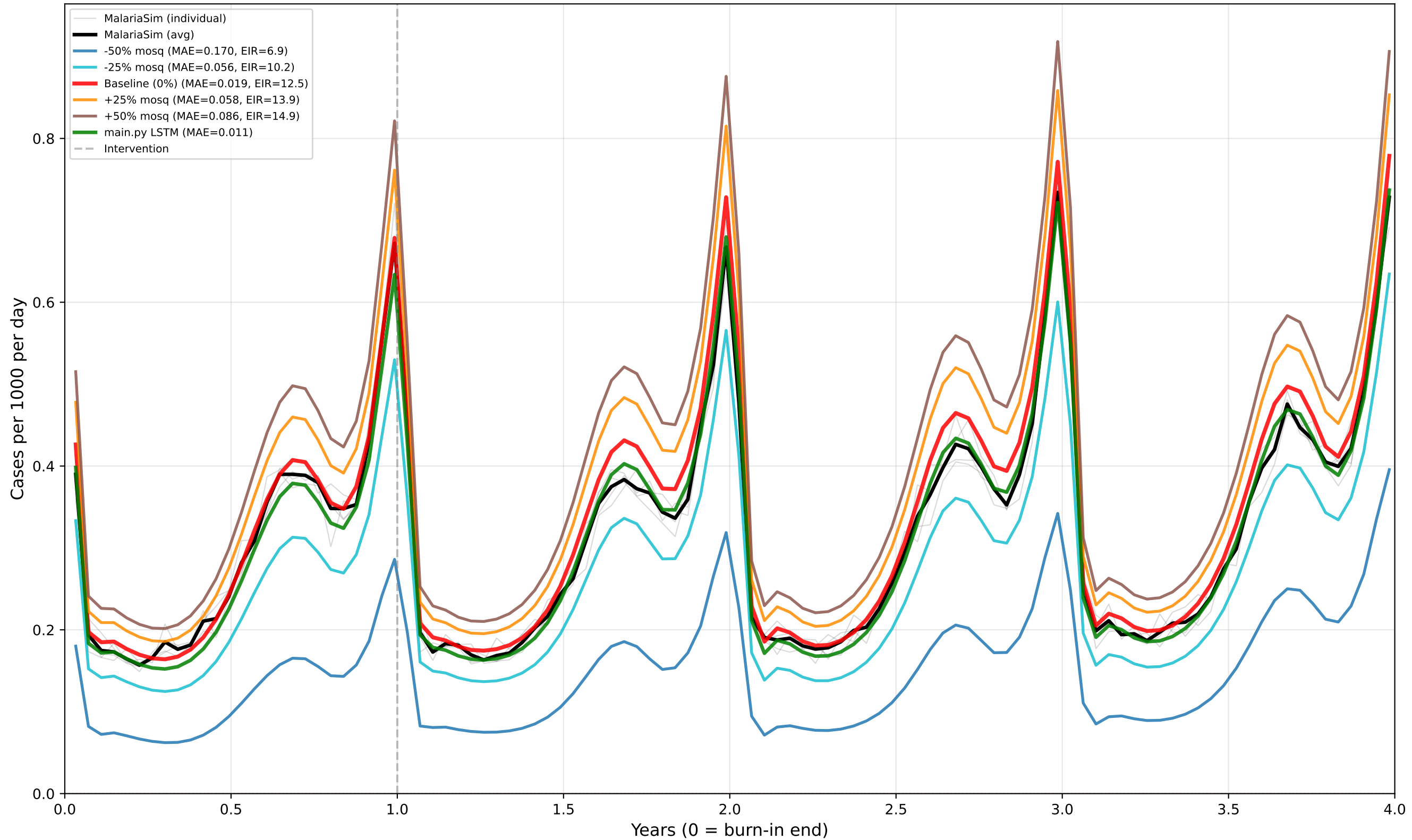
Case 20: Perennial - IRS Only - Mid EIR Predictor: CASES | True EIR: 11.8 | Est EIR (0%): 12.5 prev_y9: 0.067 | [minte v1.4.0]
