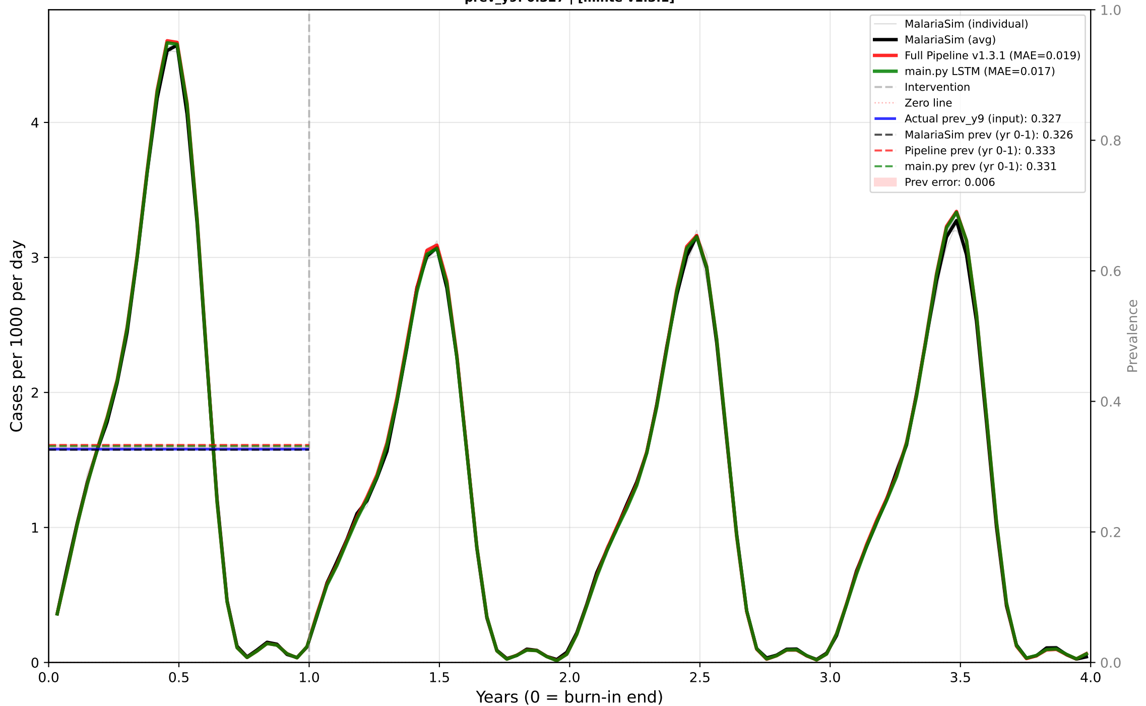
Case 26: Seasonal - LSM Only - Mid EIR Predictor: CASES | True EIR: 12.1 | Est EIR: 12.2 prev_y9: 0.327 | [minte v1.3.1]
