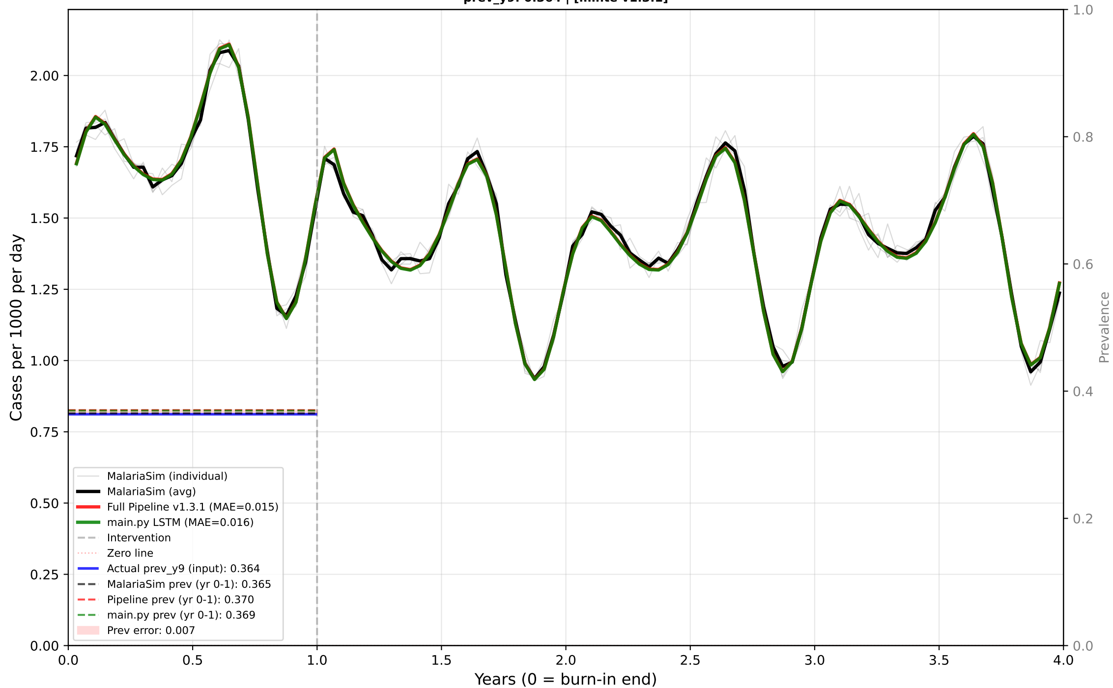
Case 24: Perennial - LSM Only - Mid EIR Predictor: CASES | True EIR: 12.2 | Est EIR: 12.2 prev_y9: 0.364 | [minte v1.3.1]
