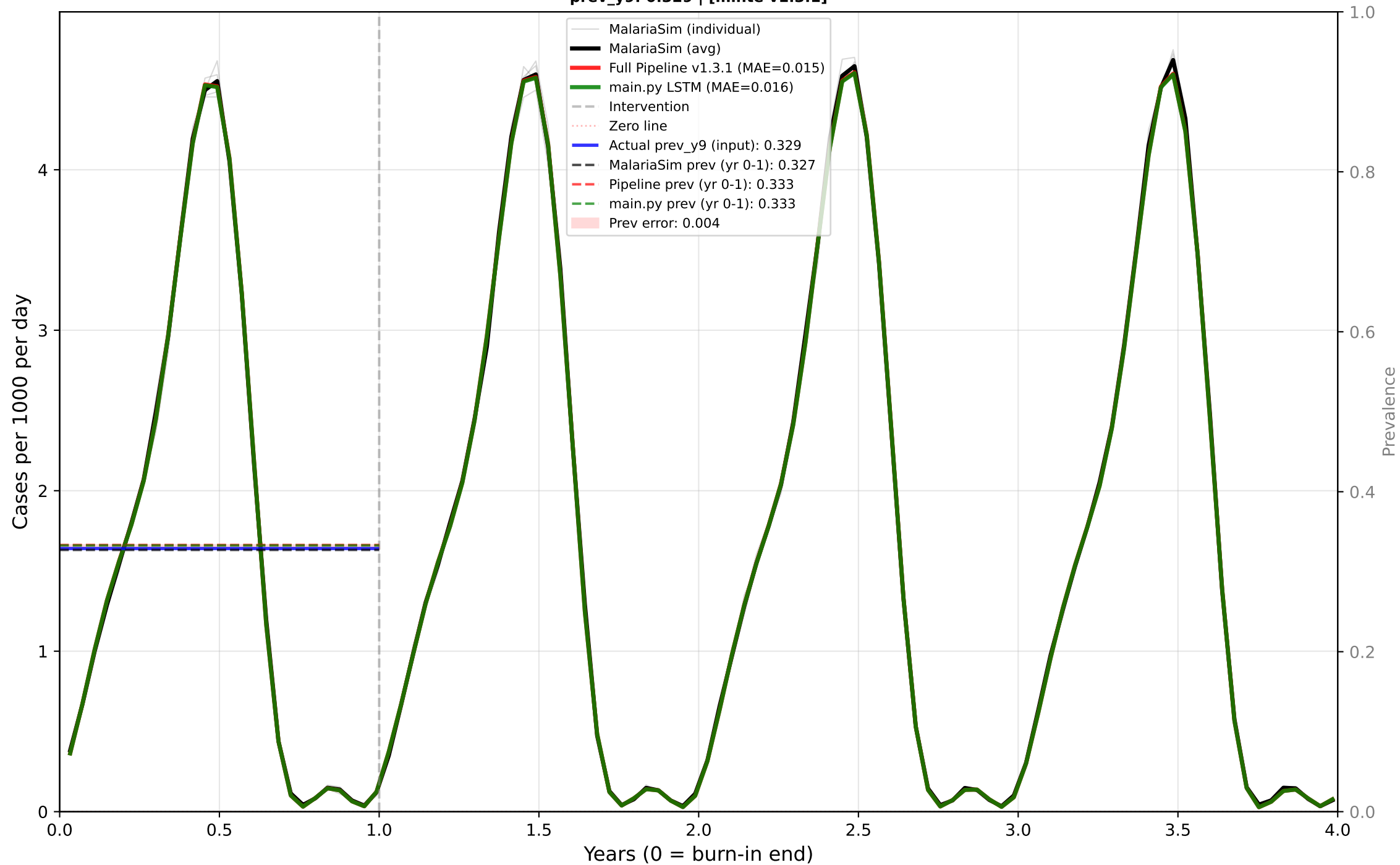
Case 5: Seasonal - No Intervention - Mid EIR Predictor: CASES | True EIR: 11.9 | Est EIR: 11.9 prev_y9: 0.329 | [minte v1.3.1]
