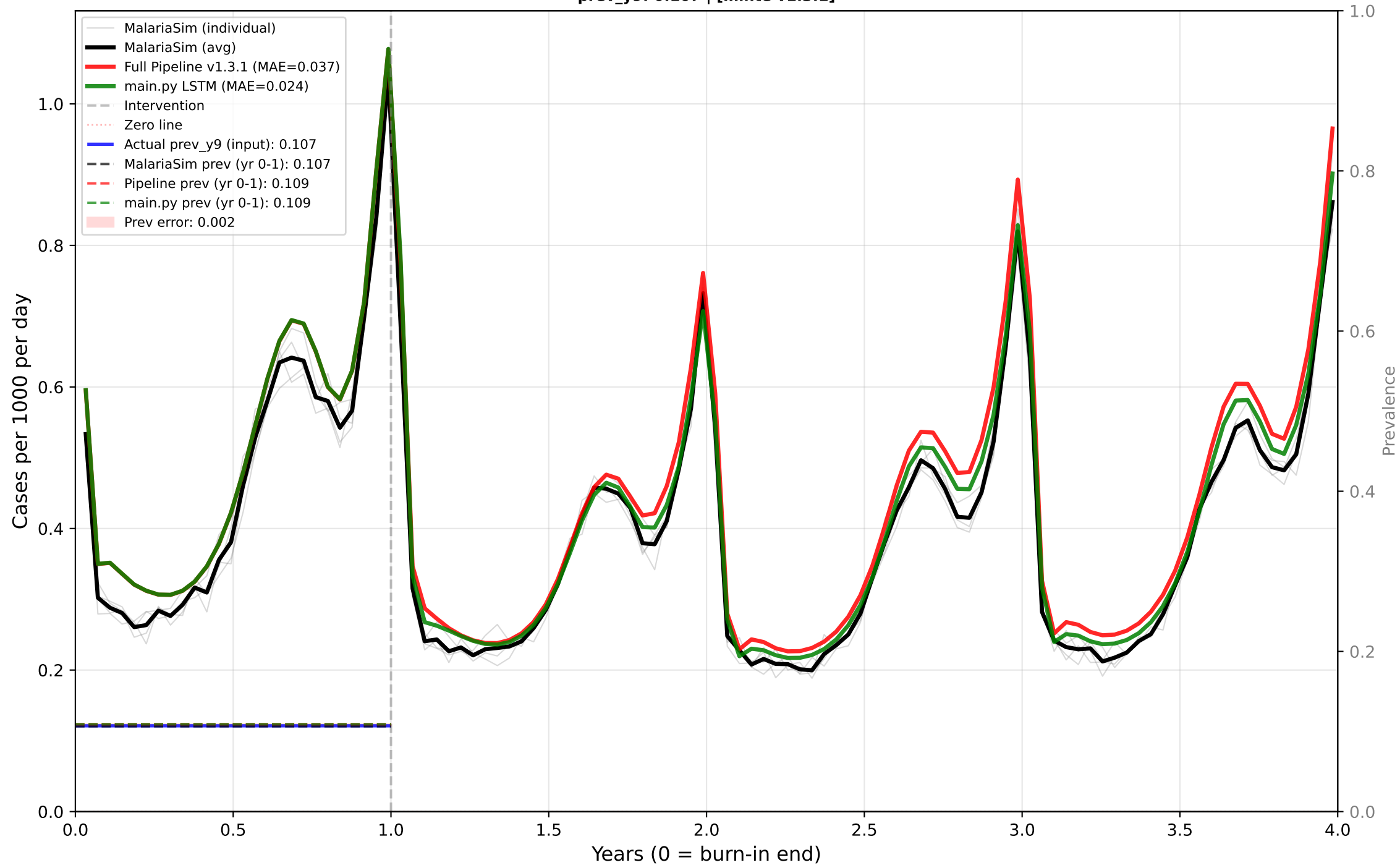
Case 41: Perennial - All Three - High EIR - High dn0 Predictor: CASES | True EIR: 24.2 | Est EIR: 24.2 prev_y9: 0.107 | [minte v1.3.1]
