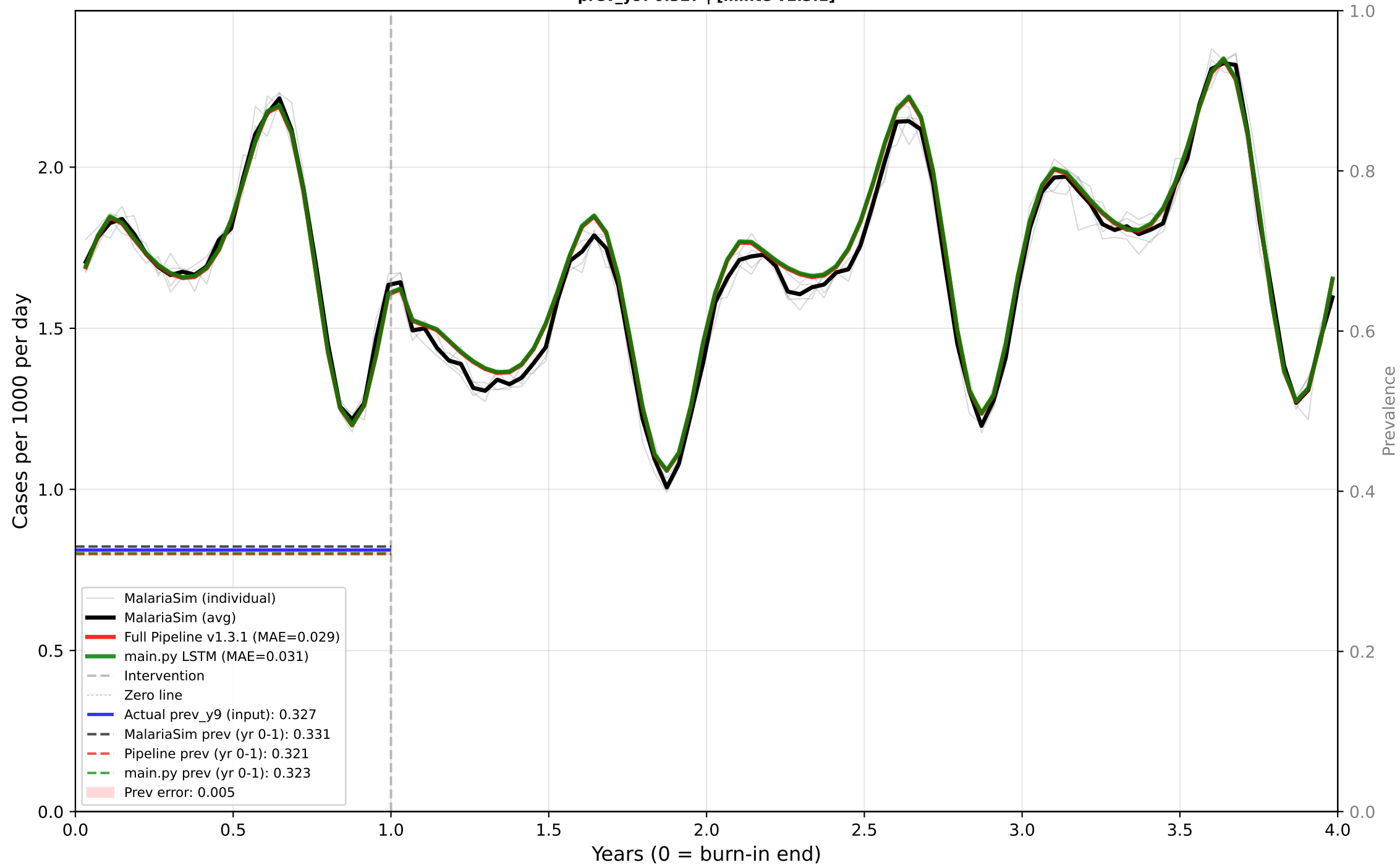
Case 8: Perennial - ITN Only - Mid EIR - Low dn0 Predictor: CASES | True EIR: 12.1 | Est EIR: 12.0 prev_y9: 0.327 | [minte v1.3.1]
