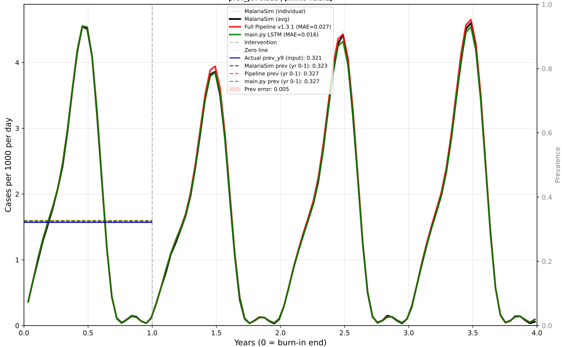
Case 17: Seasonal - ITN Only - Mid EIR - Mid dn0 Predictor: CASES | True EIR: 11.9 | Est EIR: 11.9 prev_y9: 0.321 | [minte v1.3.1]
