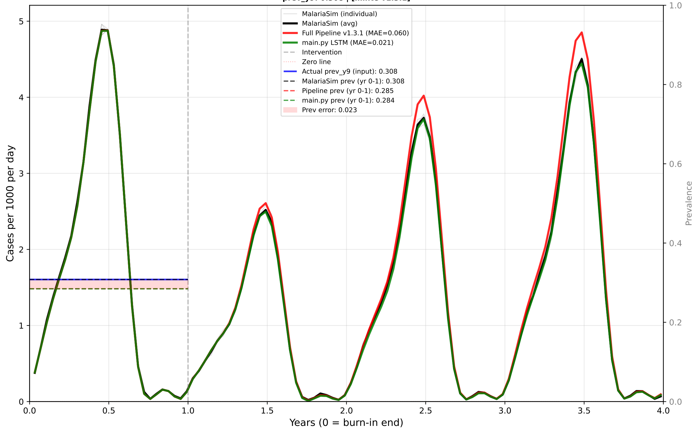
Case 34: Seasonal - ITN+LSM - Mid EIR - Mid dn0 Predictor: CASES | True EIR: 12.8 | Est EIR: 12.8 prev_y9: 0.308 | [minte v1.3.1]
