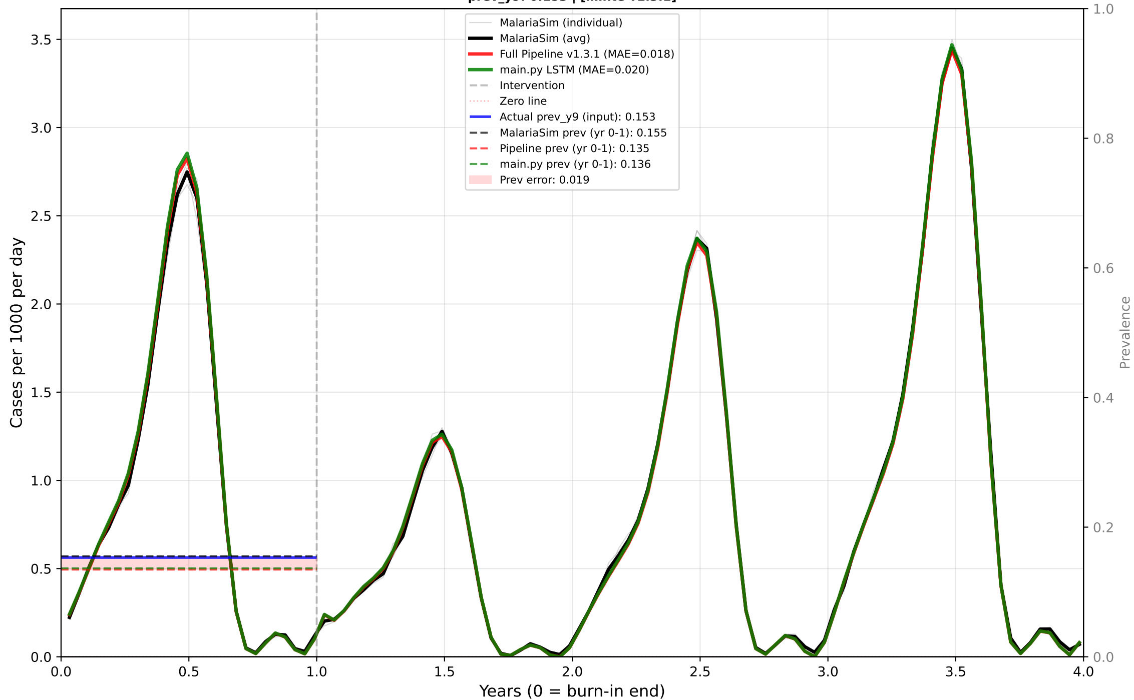
Case 30: Seasonal - ITN+IRS - Mid EIR - Mid dn0 Predictor: CASES | True EIR: 11.5 | Est EIR: 11.4 prev_y9: 0.153 | [minite v1.3.1]
