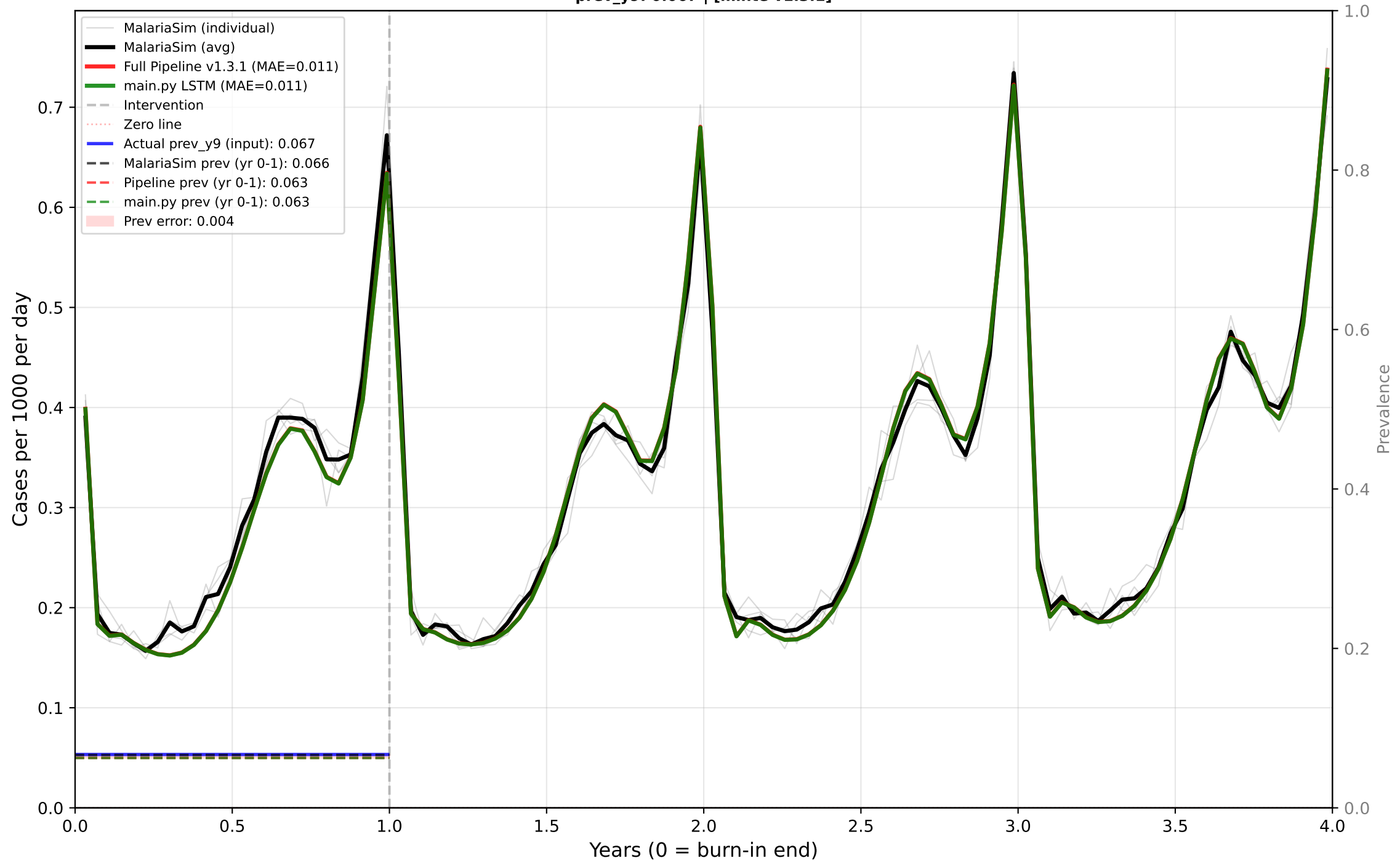
Case 20: Perennial - IRS Only - Mid EIR Predictor: CASES | True EIR: 11.8 | Est EIR: 11.8 prev_y9: 0.067 | [minte v1.3.1]
