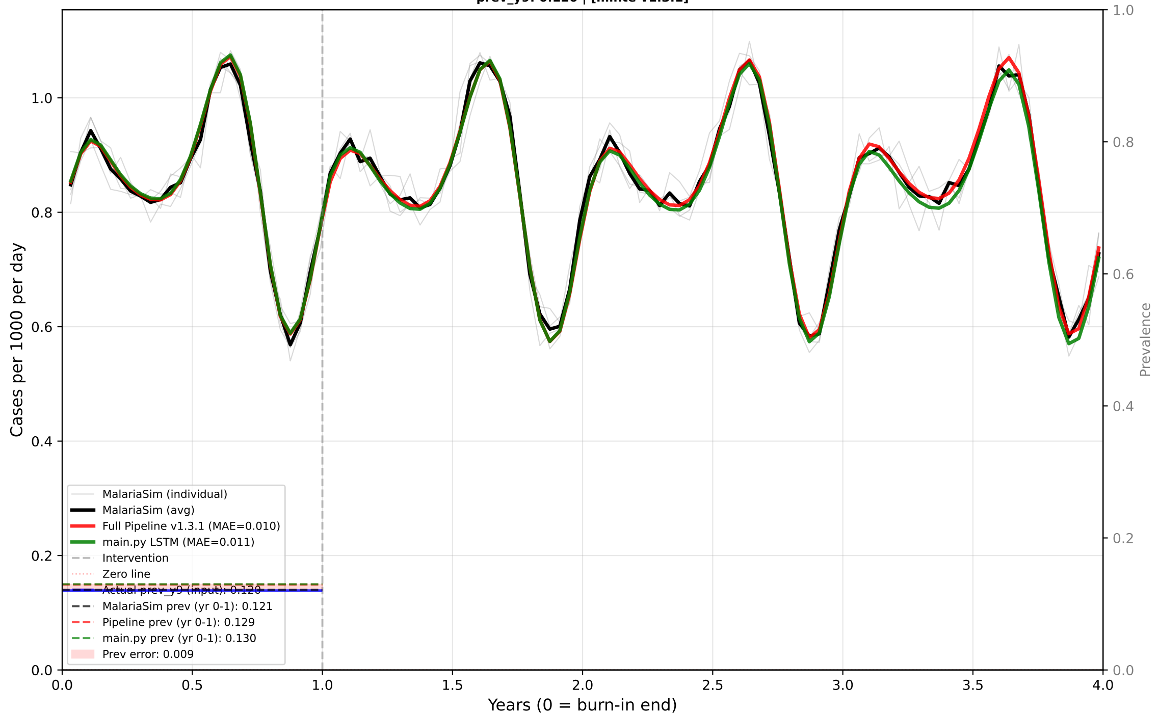
Case 1: Perennial - No Intervention - Low EIR Predictor: CASES | True EIR: 2.0 | Est EIR: 2.0 prev_y9: 0.120 | [minte v1.3.1]
