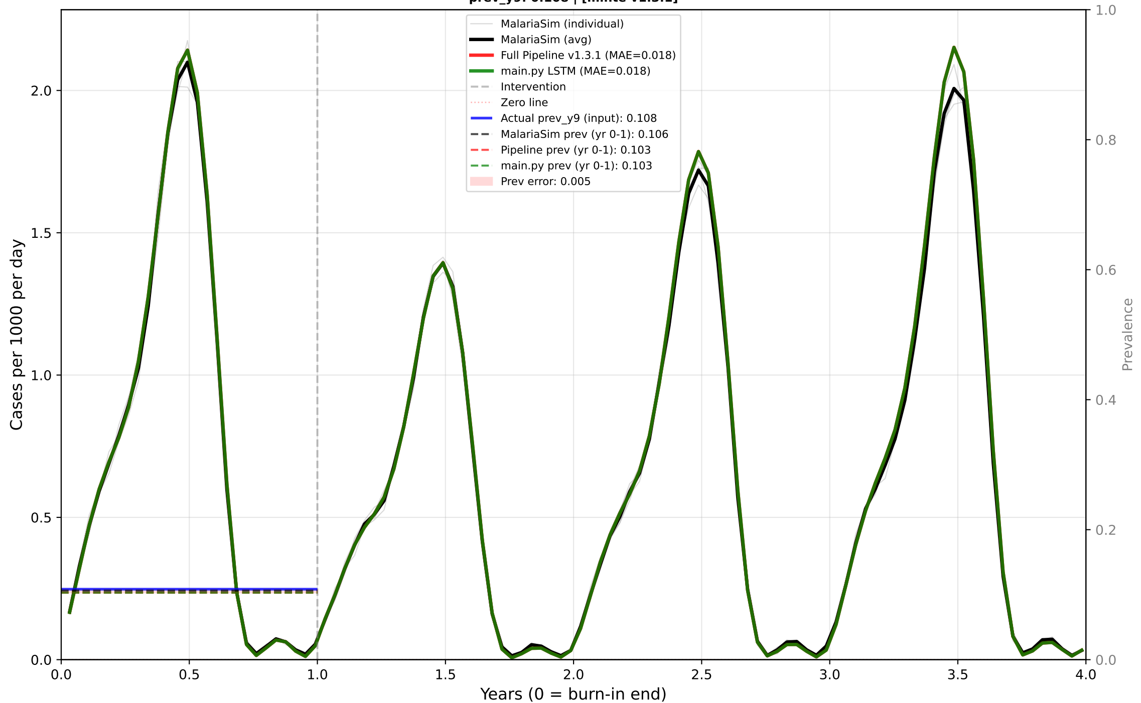
Case 16: Seasonal - ITN Only - Low EIR - Low dn0 Predictor: CASES | True EIR: 2.0 | Est EIR: 2.0 prev_y9: 0.108 | [minte v1.3.1]
