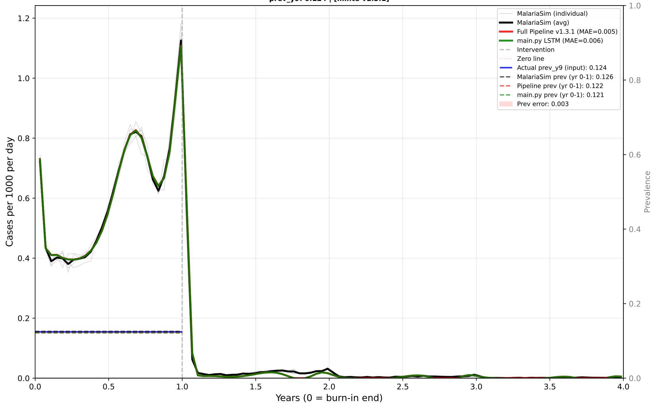
Case 40: Perennial - All Three - Mid EIR - Mid dn0 Predictor: CASES | True EIR: 13.0 | Est EIR: 13.0 prev_y9: 0.124 | [minte v1.3.1]
