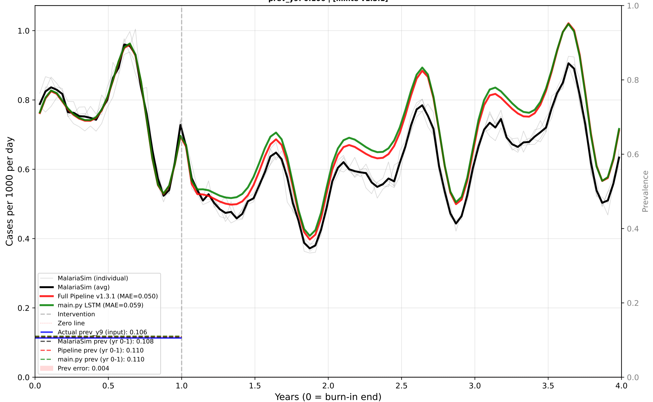
Case 7: Perennial - ITN Only - Low EIR - Low dn0 Predictor: CASES | True EIR: 1.7 | Est EIR: 1.6 prev_y9: 0.106 | [minte v1.3.1]
