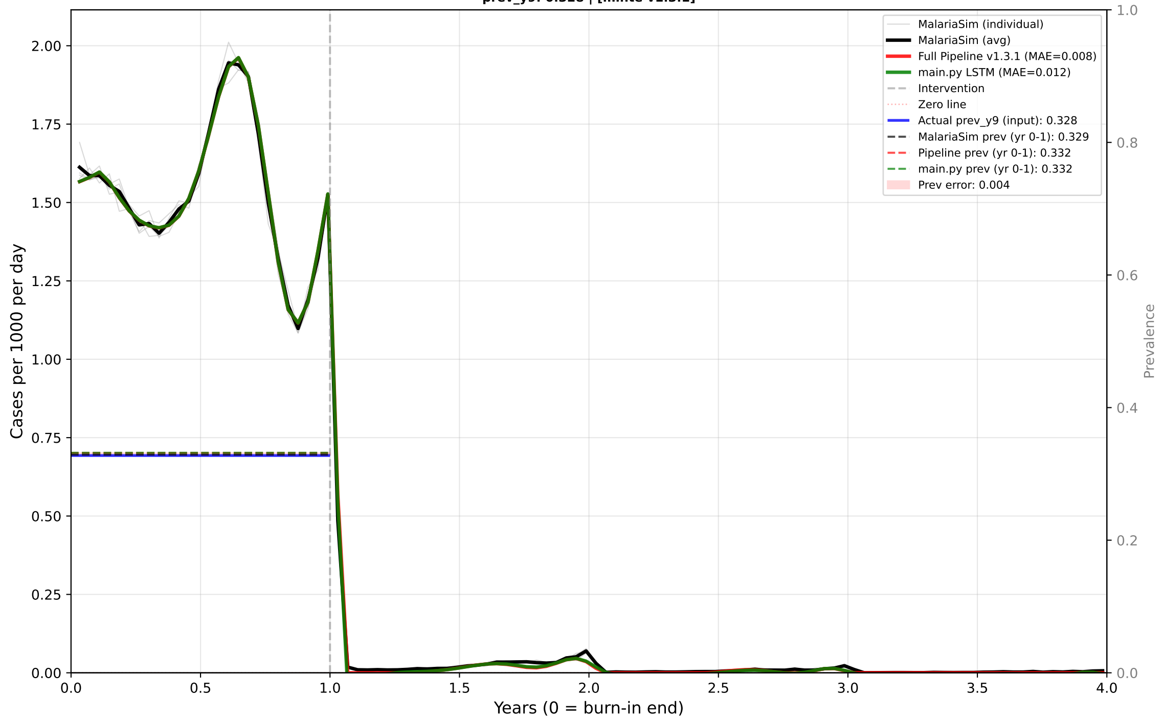
Case 36: Perennial - IRS+LSM - Mid EIR Predictor: CASES | True EIR: 11.9 | Est EIR: 11.9 prev_y9: 0.328 | [minte v1.3.1]
