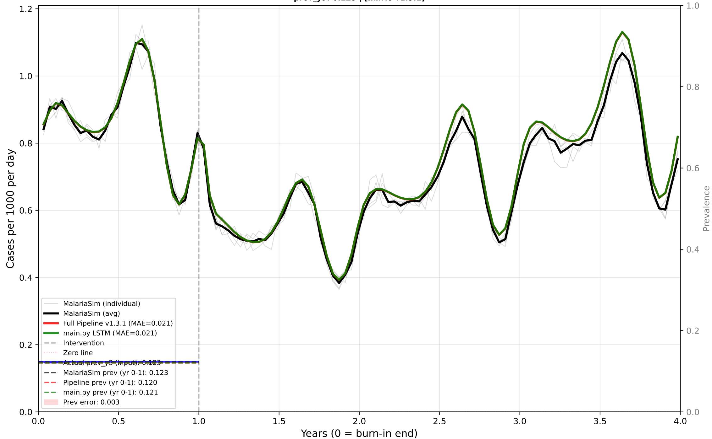
Case 13: Perennial - ITN Only - Low EIR - High dn0 Predictor: CASES | True EIR: 2.2 | Est EIR: 2.2 prev_y9: 0.123 | [minte v1.3.1]
