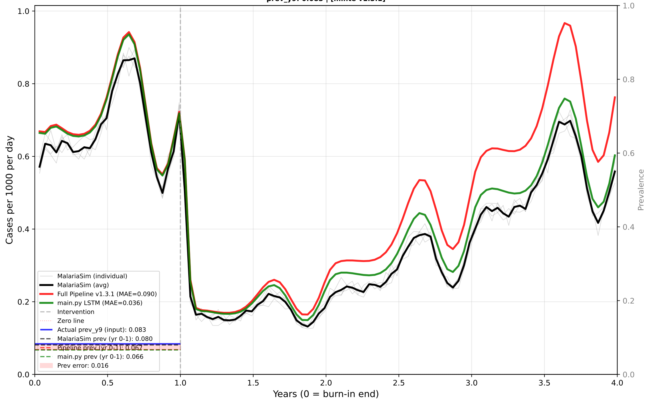
Case 10: Perennial - ITN Only - Low EIR - Mid dn0 Predictor: CASES | True EIR: 2.1 | Est EIR: 2.1 prev_y9: 0.083 | [minte v1.3.1]
