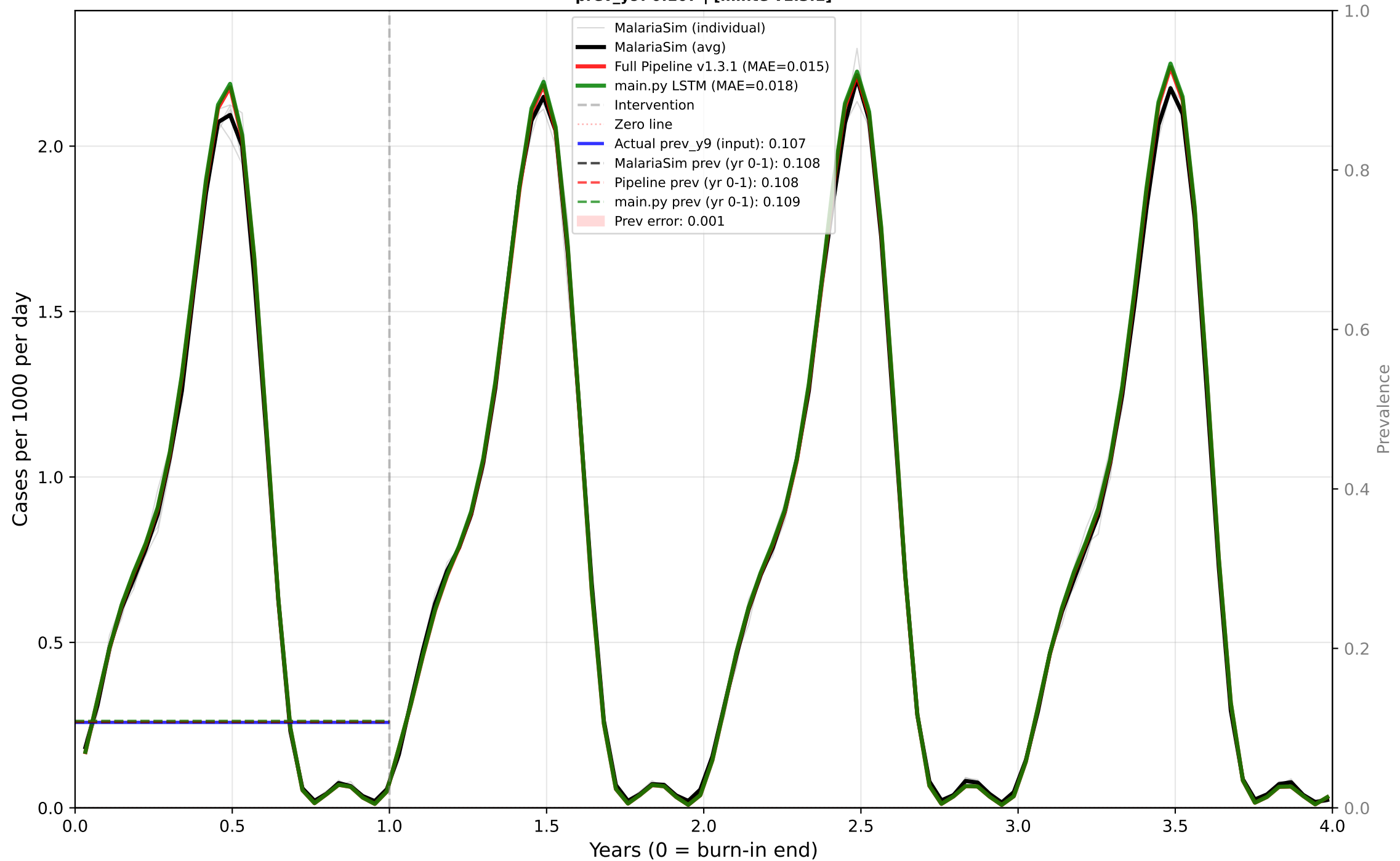
Case 4: Seasonal - No Intervention - Low EIR Predictor: CASES | True EIR: 2.0 | Est EIR: 2.0 prev_y9: 0.107 | [minte v1.3.1]
