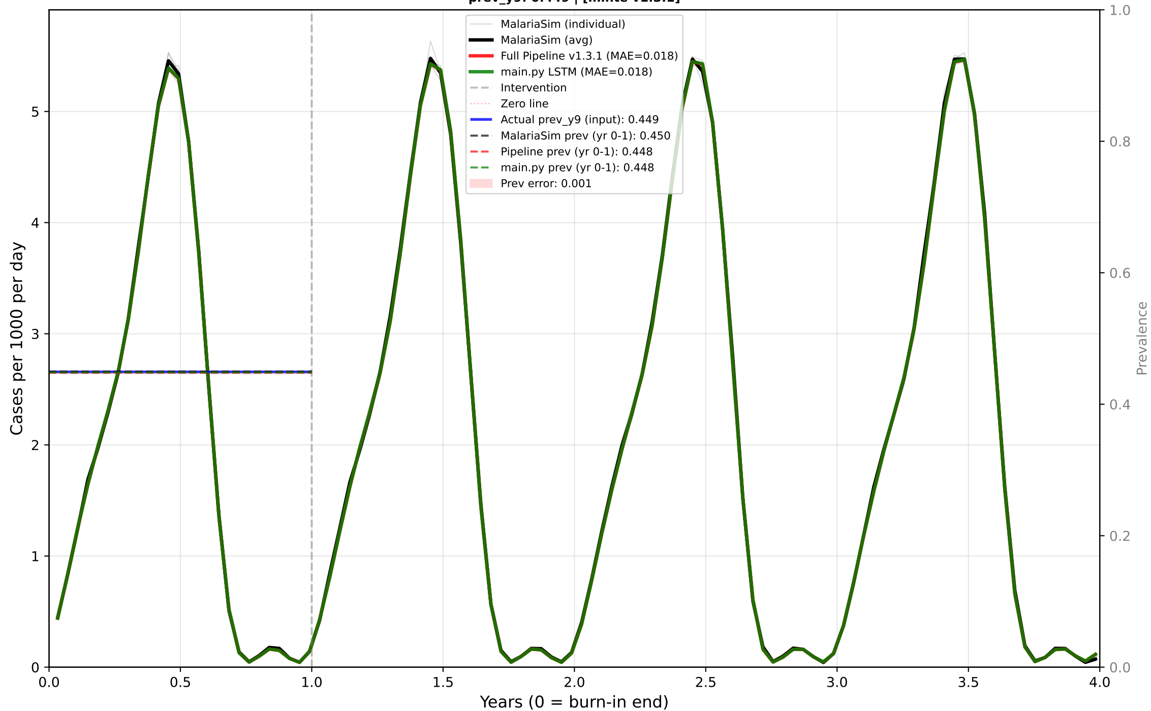
Case 6: Seasonal - No Intervention - High EIR Predictor: CASES | True EIR: 25.4 | Est EIR: 25.3 prev_y9: 0.449 | [minte v1.3.1]
