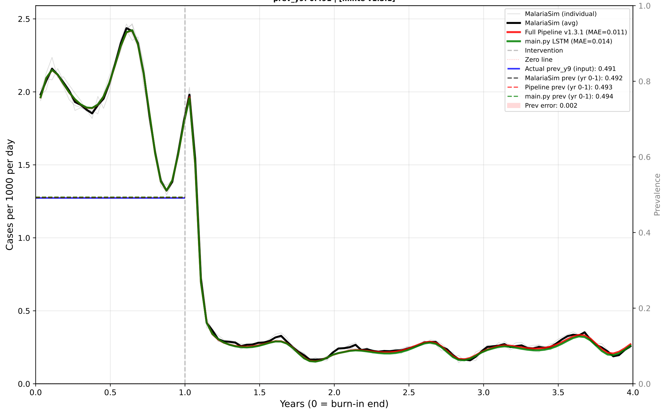
Case 25: Perennial - LSM Only - High EIR Predictor: CASES | True EIR: 25.0 | Est EIR: 25.0 prev_y9: 0.491 | [minte v1.3.1]
