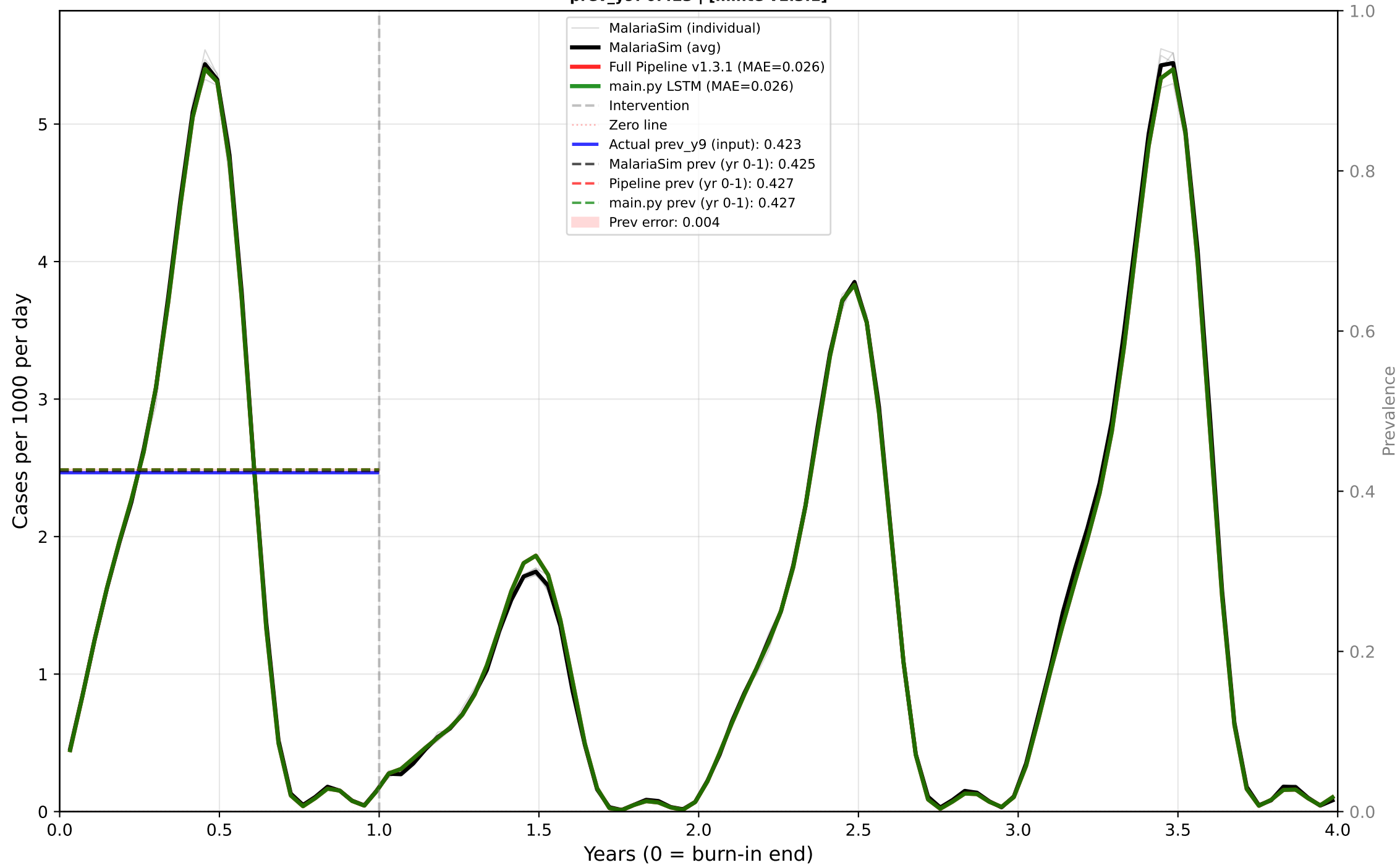
Case 18: Seasonal - ITN Only - High EIR - High dn0 Predictor: CASES | True EIR: 24.1 | Est EIR: 24.1 prev_y9: 0.423 | [minte v1.3.1]
