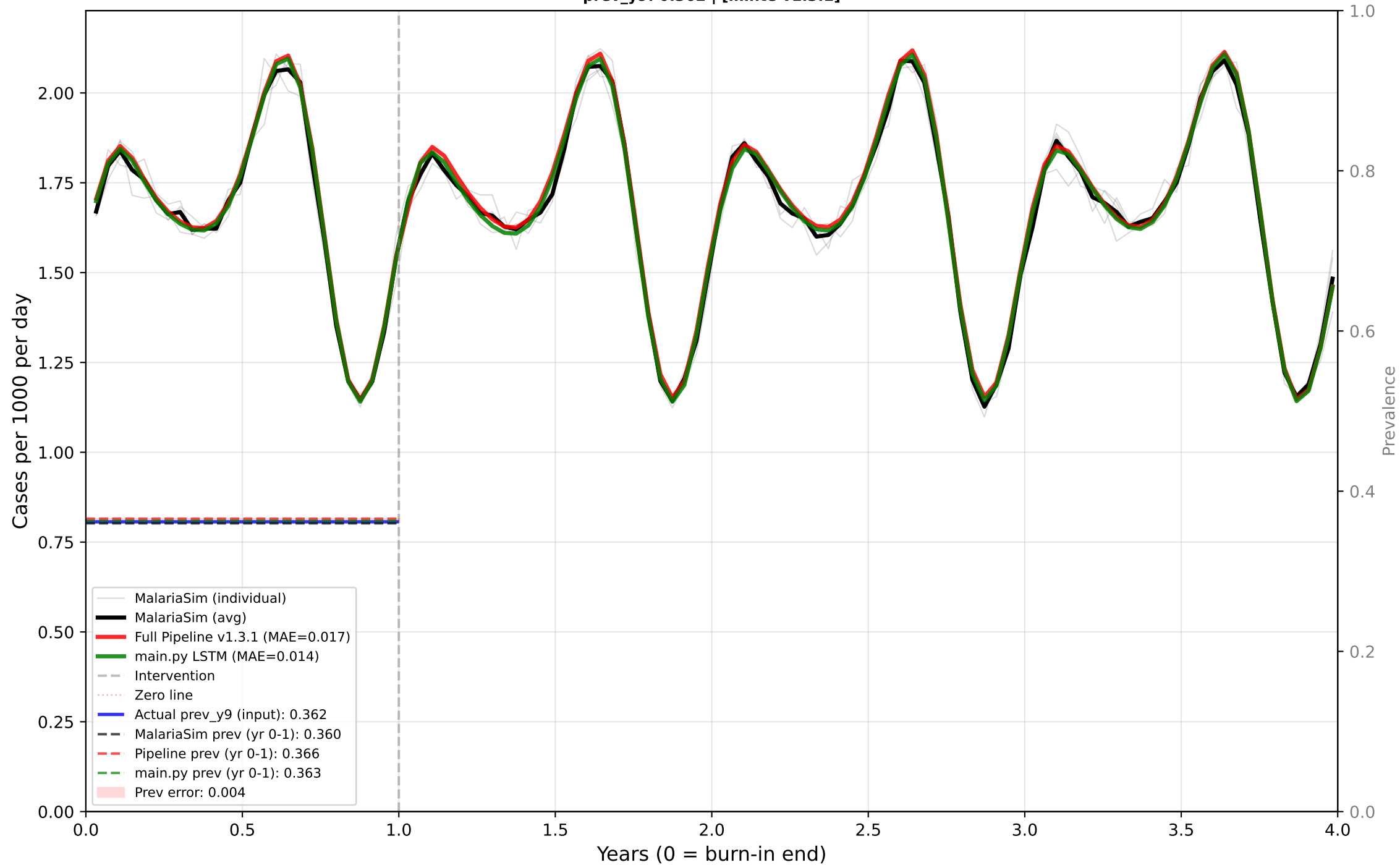
Case 2: Perennial - No Intervention - Mid EIR Predictor: CASES | True EIR: 12.0 | Est EIR: 12.2 prev_y9: 0.362 | [minte v1.3.1]
