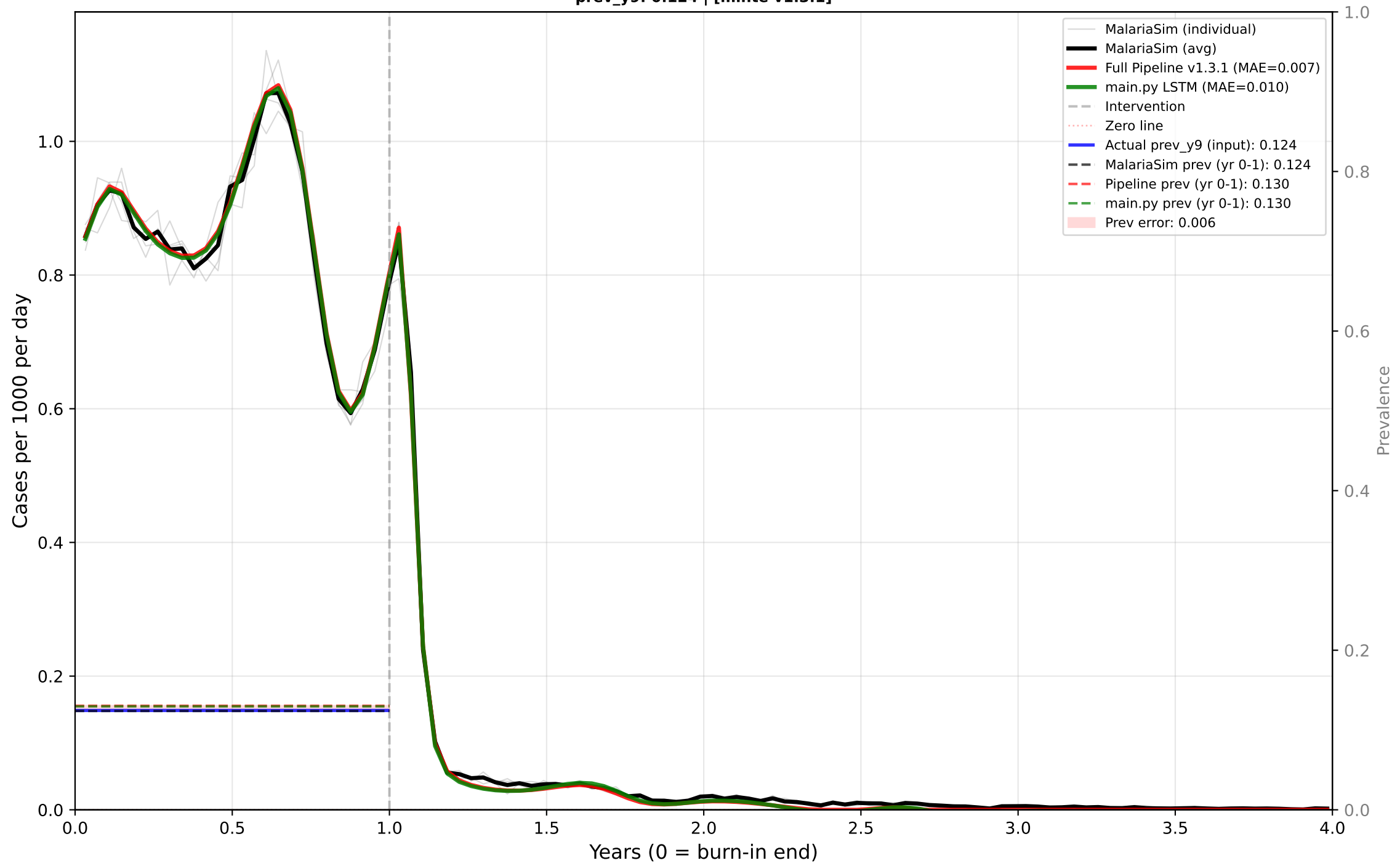
Case 23: Perennial - LSM Only - Low EIR Predictor: CASES | True EIR: 2.0 | Est EIR: 2.0 prev_y9: 0.124 | [minte v1.3.1]
