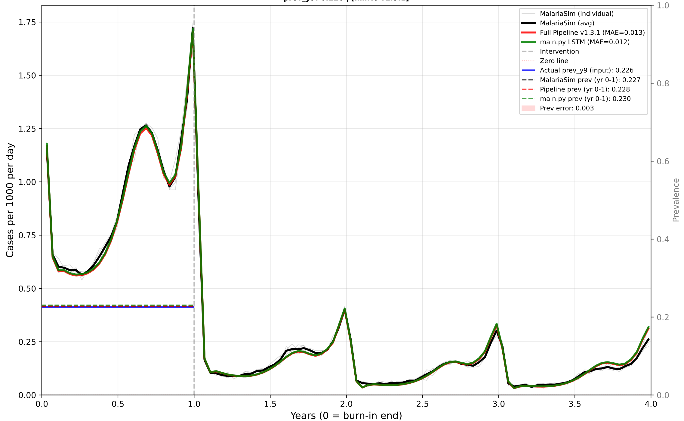
Case 37: Perennial - IRS+LSM - High EIR Predictor: CASES | True EIR: 24.8 | Est EIR: 24.4 prev_y9: 0.226 | [minte v1.3.1]
