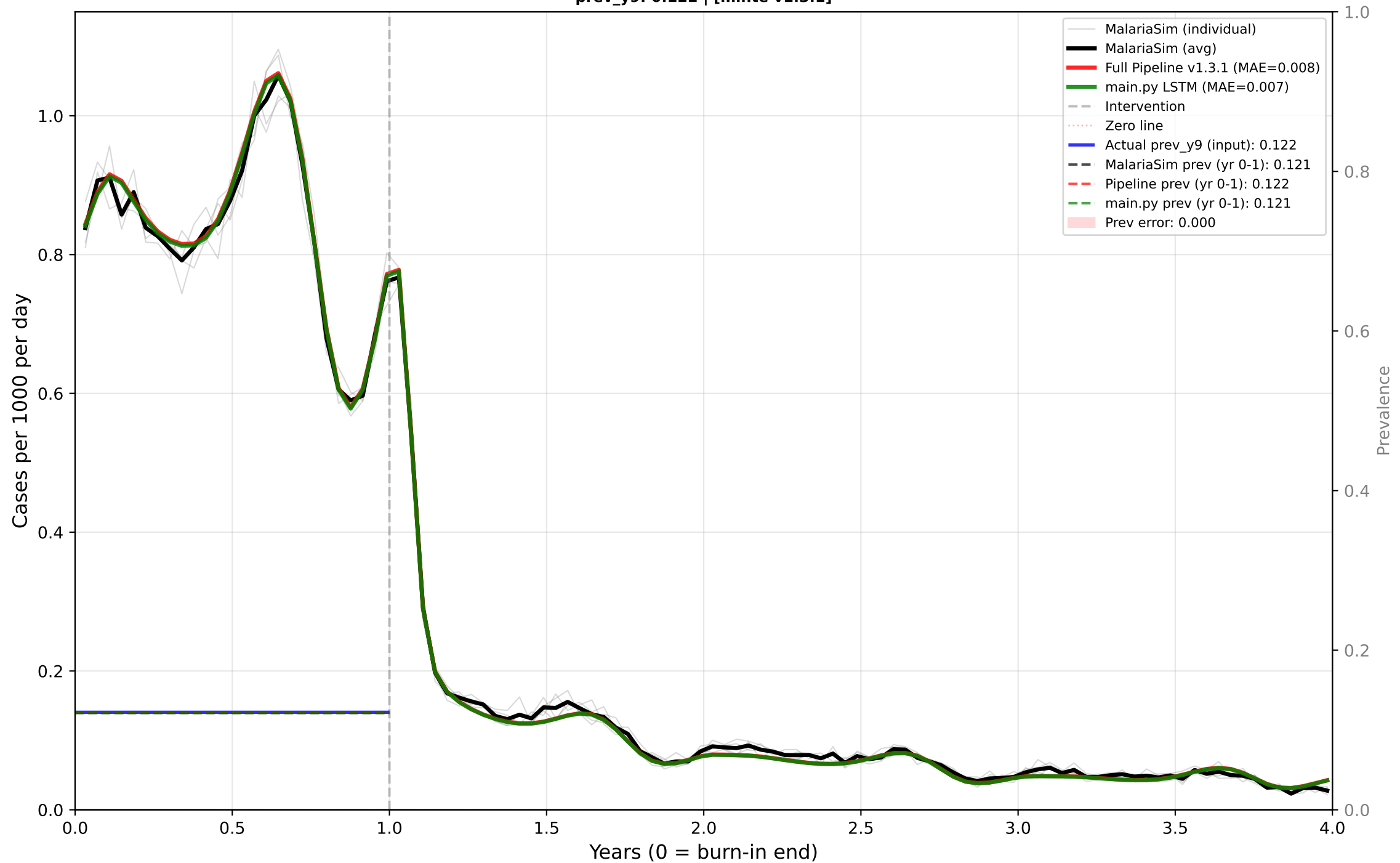
Case 31: Perennial - ITN+LSM - Low EIR - Low dn0 Predictor: CASES | True EIR: 2.0 | Est EIR: 2.0 prev_y9: 0.122 | [minte v1.3.1]
