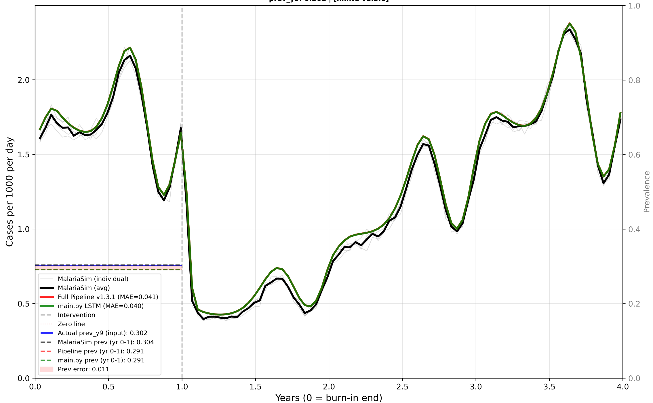
Case 14: Perennial - ITN Only - Mid EIR - High dn0 Predictor: CASES | True EIR: 11.9 | Est EIR: 11.9 prev_y9: 0.302 | [minte v1.3.1]
