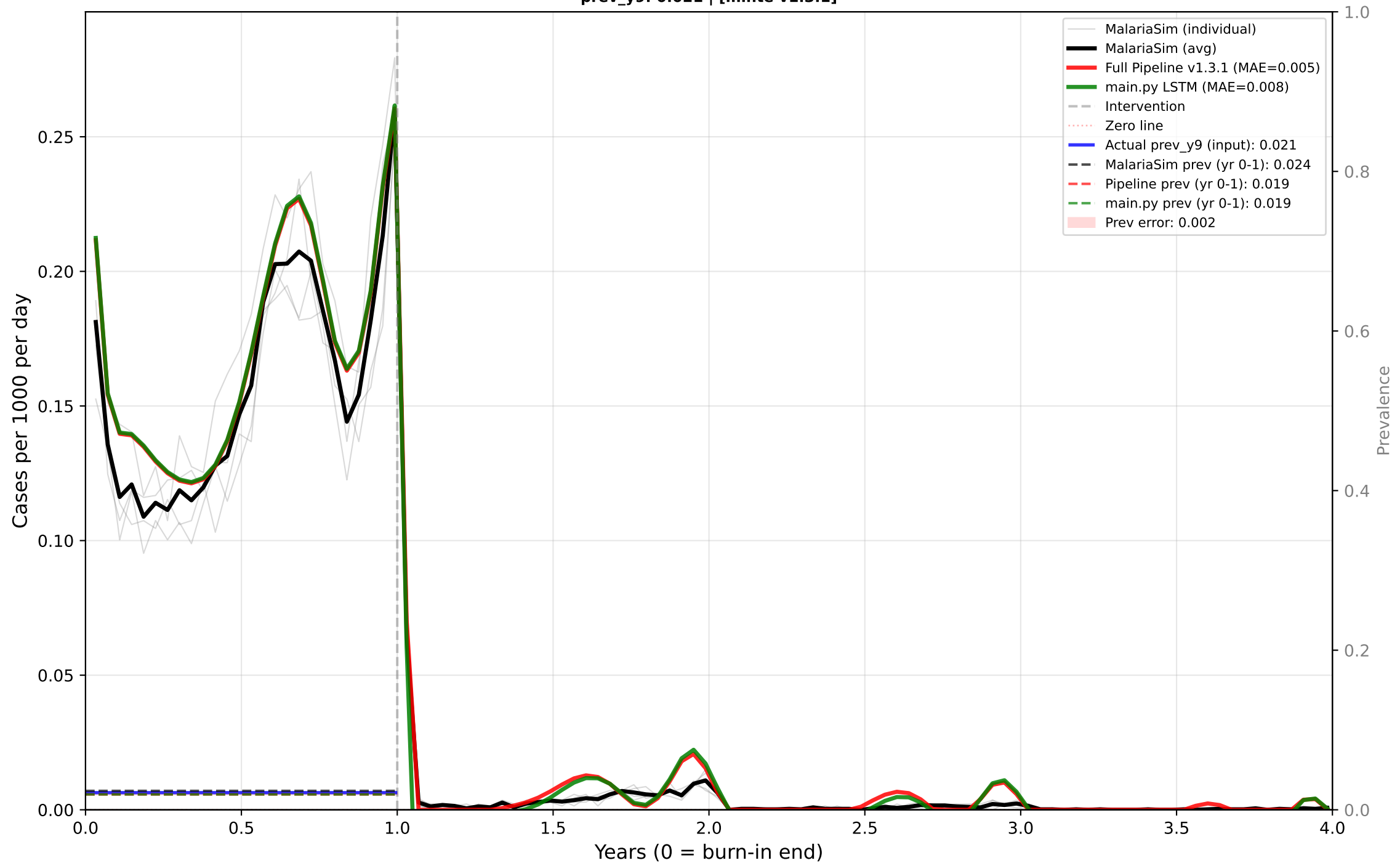
Case 35: Perennial - IRS+LSM - Low EIR Predictor: CASES | True EIR: 2.0 | Est EIR: 2.0 prev_y9: 0.021 | [minte v1.3.1]
