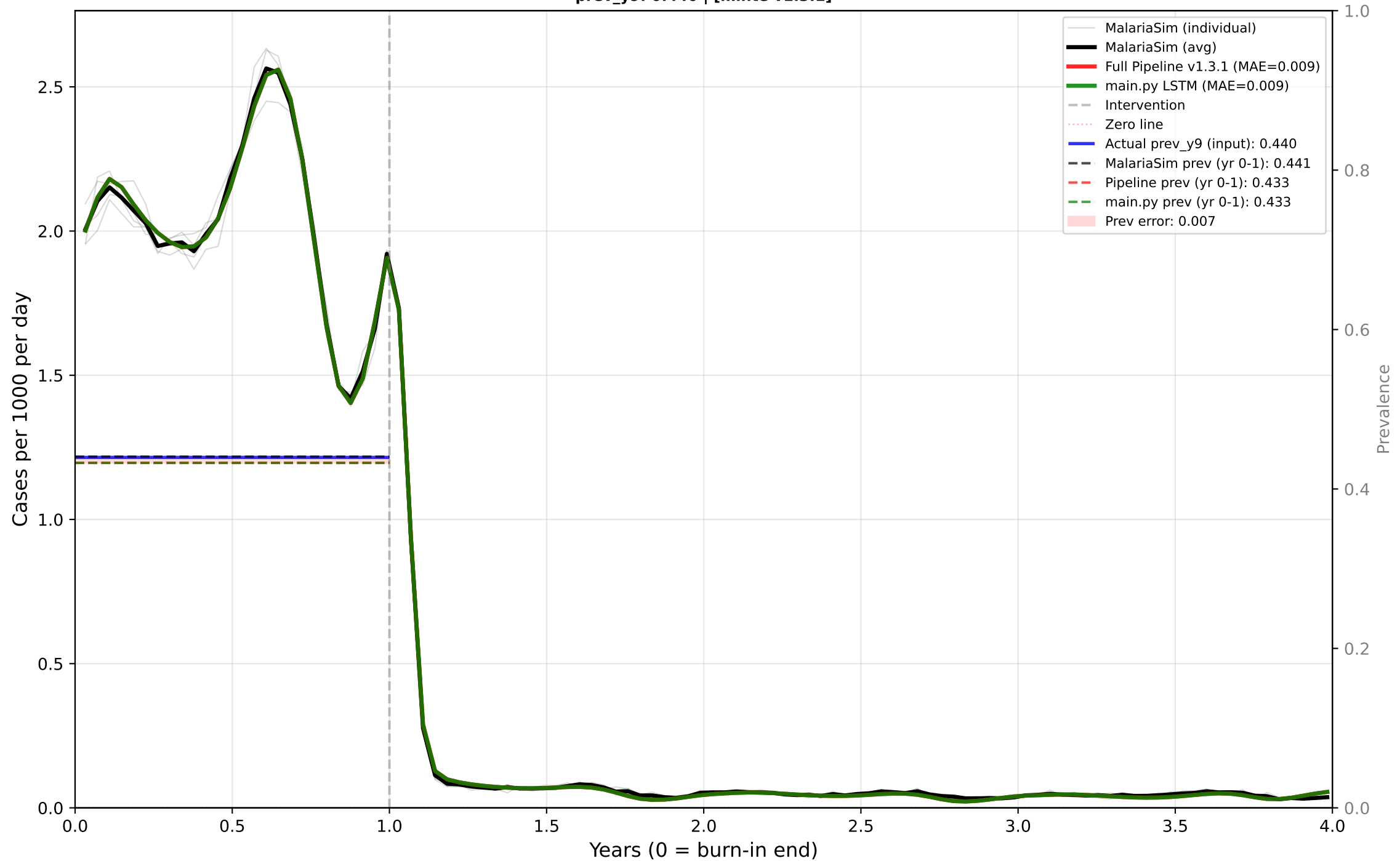
Case 33: Perennial - ITN+LSM - High EIR - High dn0 Predictor: CASES | True EIR: 24.1 | Est EIR: 24.1 prev_y9: 0.440 | [minte v1.3.1]
