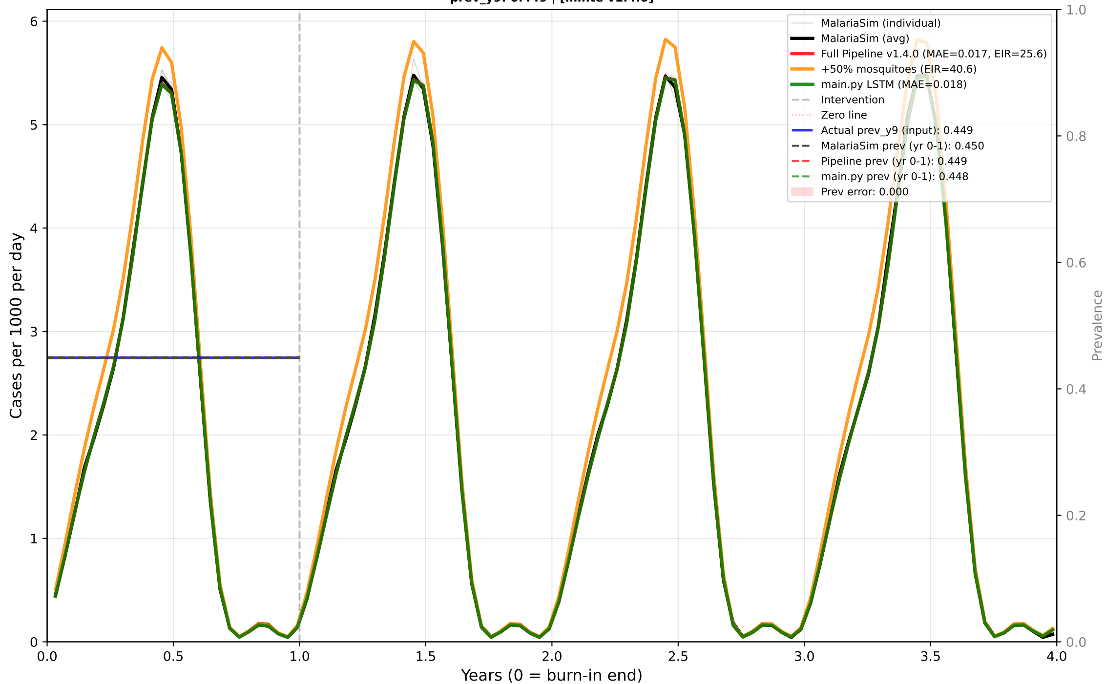
Case 6: Seasonal - No Intervention - High EIR Predictor: CASES | True EIR: 25.4 | Est EIR: 25.6 prev_y9: 0.449 | [minte v1.4.0]
