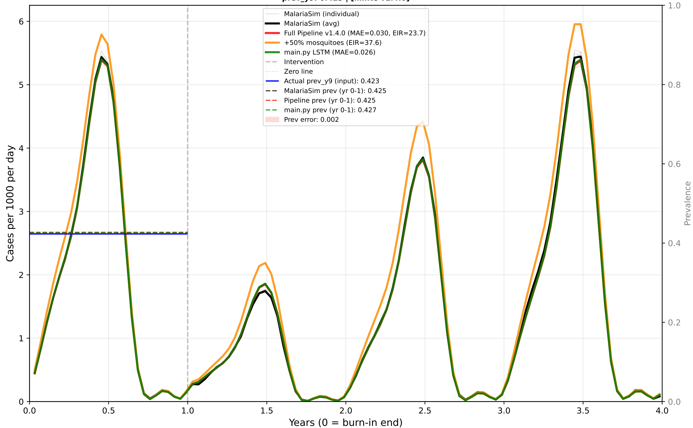
Case 18: Seasonal - ITN Only - High EIR - High dn0 Predictor: CASES | True EIR: 24.1 | Est EIR: 23.7 prev_y9: 0.423 | [minte v1.4.0]
