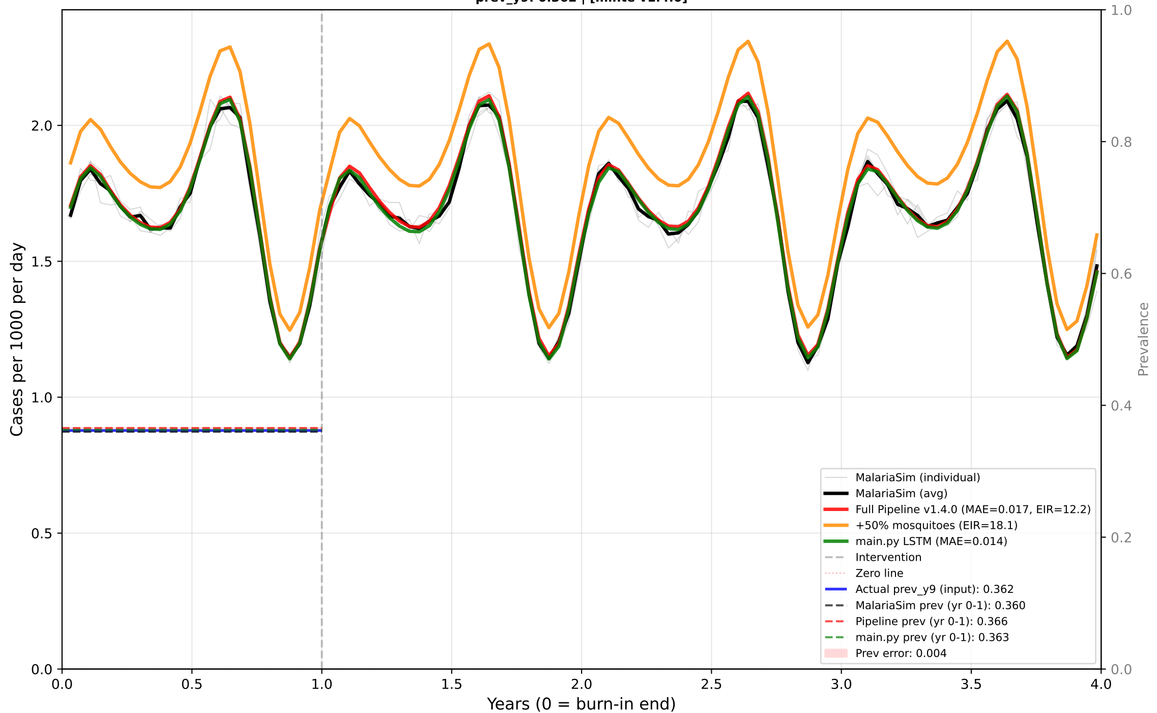
Case 2: Perennial - No Intervention - Mid EIR Predictor: CASES | True EIR: 12.0 | Est EIR: 12.2 prev_y9: 0.362 | [minte v1.4.0]
