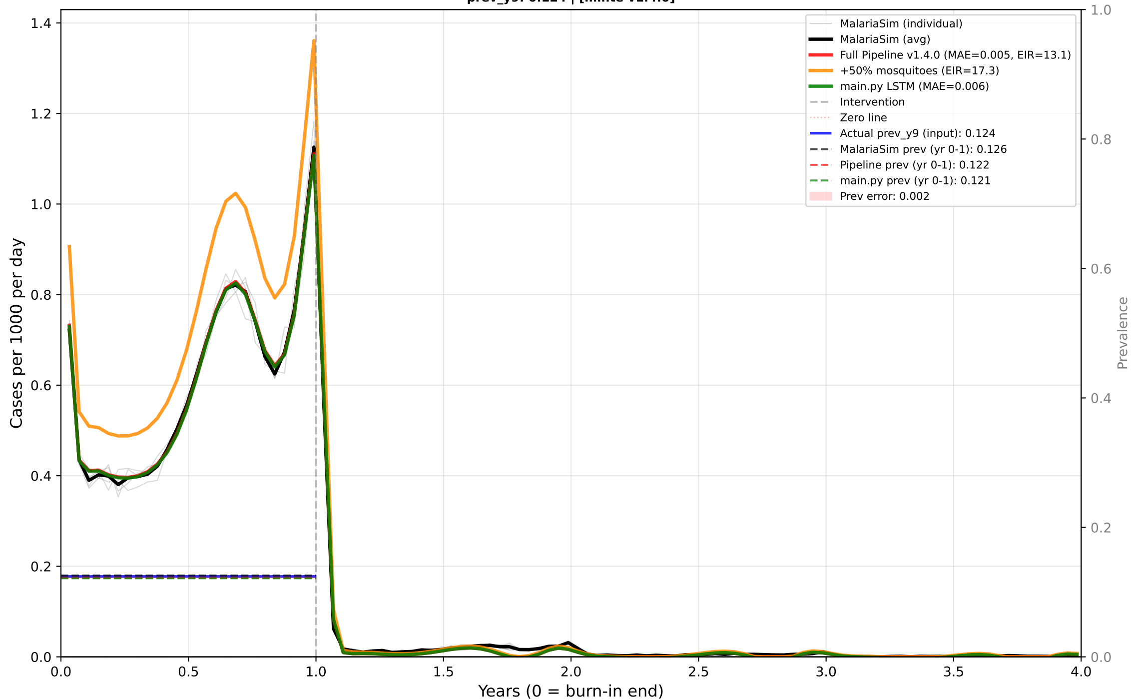
Case 40: Perennial - All Three - Mid EIR - Mid dn0 Predictor: CASES | True EIR: 13.0 | Est EIR: 13.1 prev_y9: 0.124 | [minte v1.4.0]
