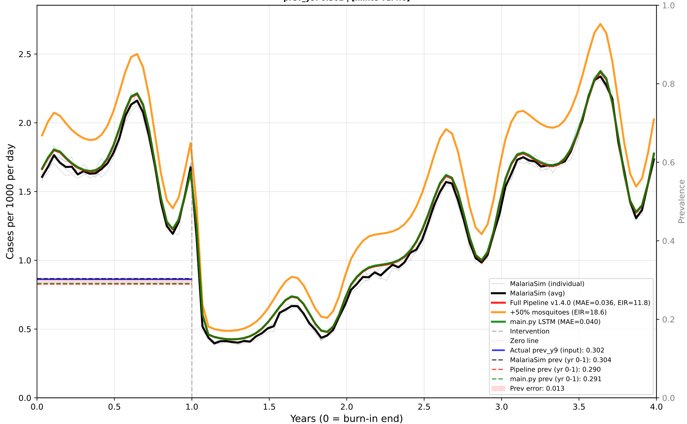
Case 14: Perennial - ITN Only - Mid EIR - High dn0 Predictor: CASES | True EIR: 11.9 | Est EIR: 11.8 prev_y9: 0.302 | [minte v1.4.0]
