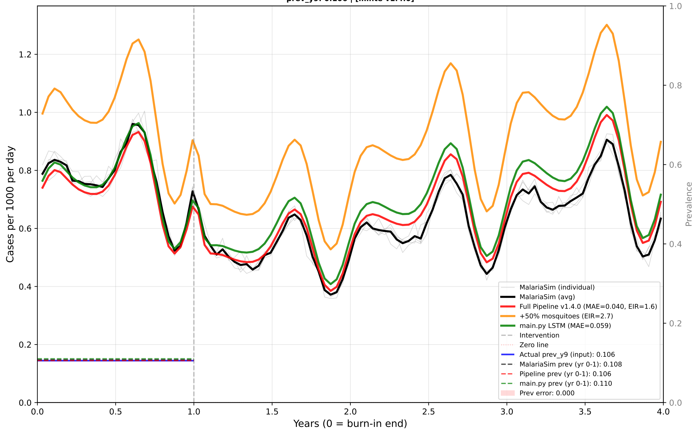
Case 7: Perennial - ITN Only - Low EIR - Low dn0 Predictor: CASES | True EIR: 1.7 | Est EIR: 1.6 prev_y9: 0.106 | [minte v1.4.0]
