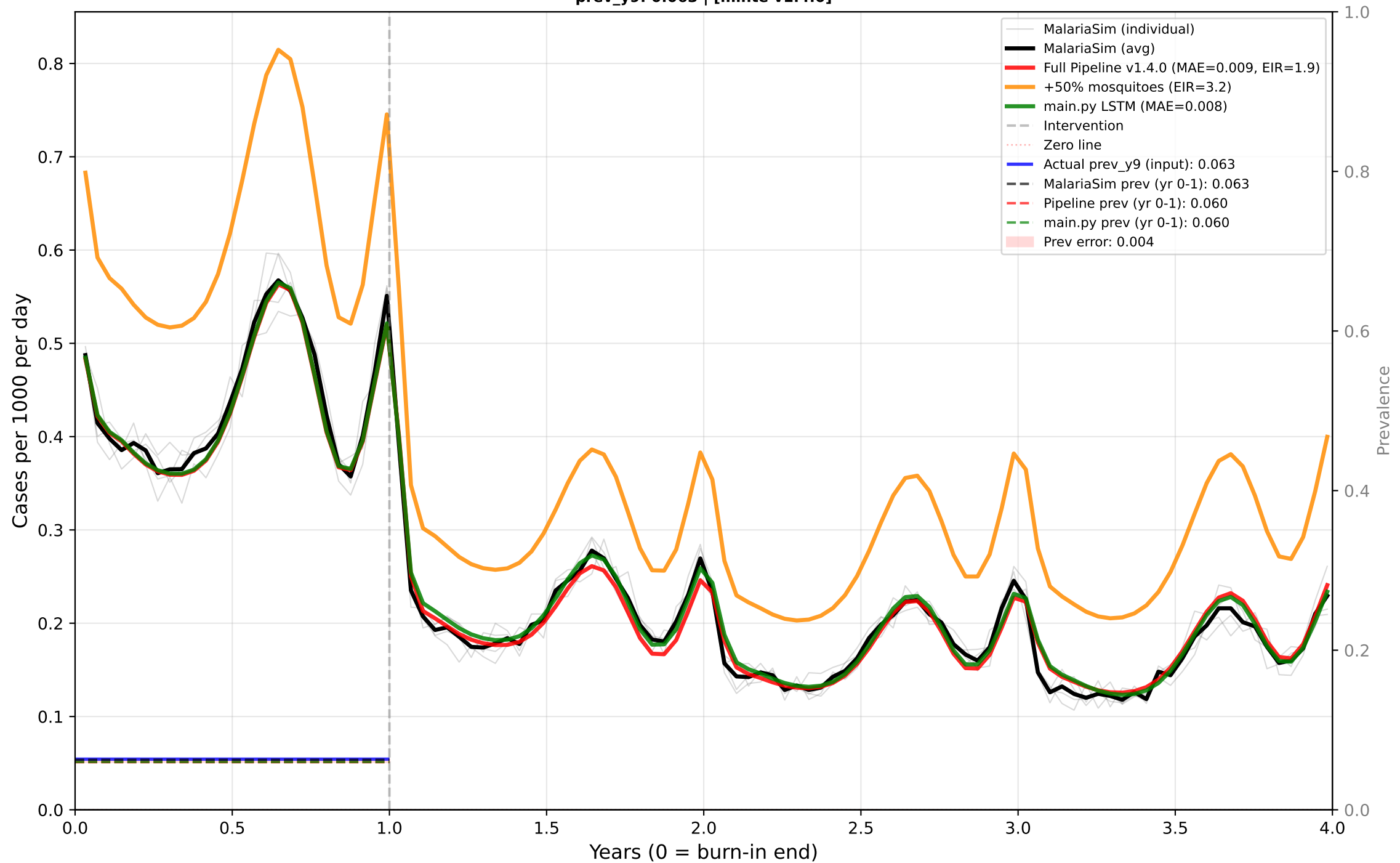
Case 27: Perennial - ITN+IRS - Low EIR - Low dn0 Predictor: CASES | True EIR: 2.0 | Est EIR: 1.9 prev_y9: 0.063 | [minte v1.4.0]
