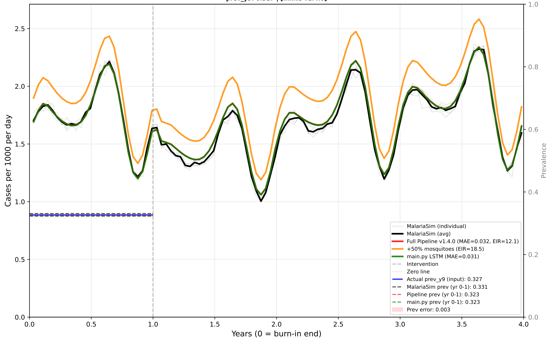
Case 8: Perennial - ITN Only - Mid EIR - Low dn0 Predictor: CASES | True EIR: 12.1 | Est EIR: 12.1 prev_y9: 0.327 | [minte v1.4.0]
