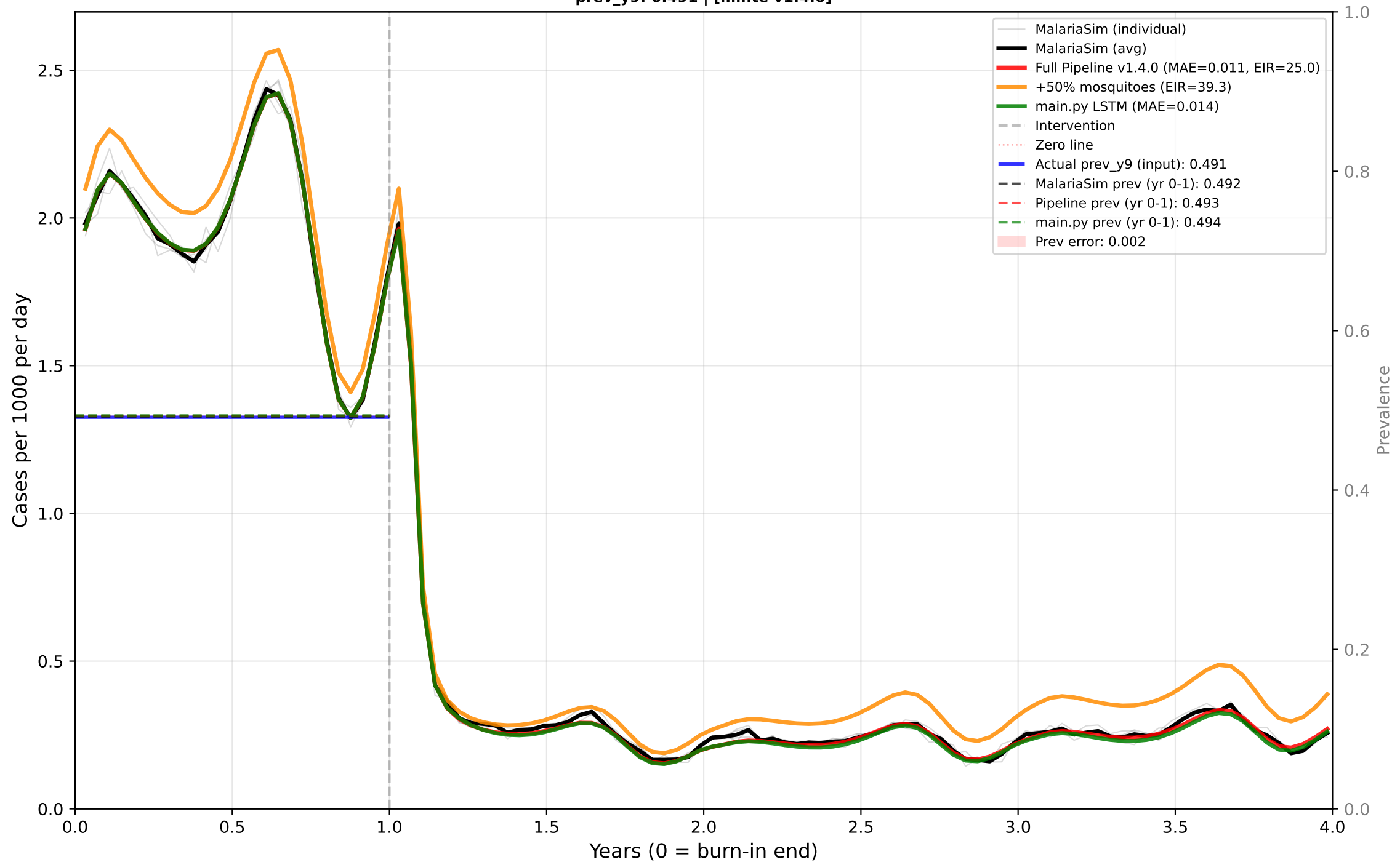
Case 25: Perennial - LSM Only - High EIR Predictor: CASES | True EIR: 25.0 | Est EIR: 25.0 prev_y9: 0.491 | [minte v1.4.0]
