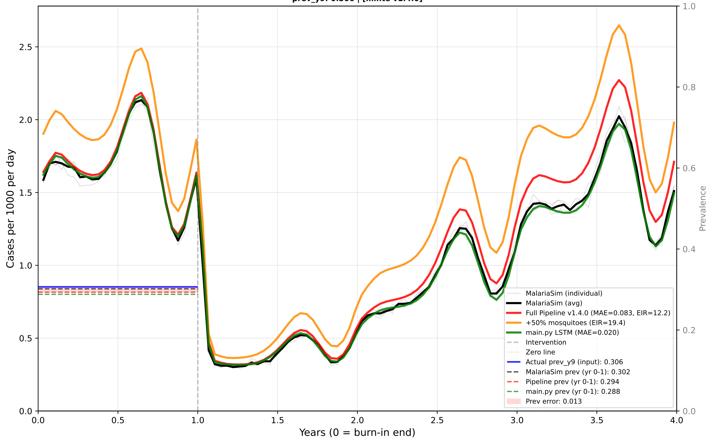
Case 11: Perennial - ITN Only - Mid EIR - Mid dn0 Predictor: CASES | True EIR: 11.8 | Est EIR: 12.2 prev_y9: 0.306 | [minte v1.4.0]
