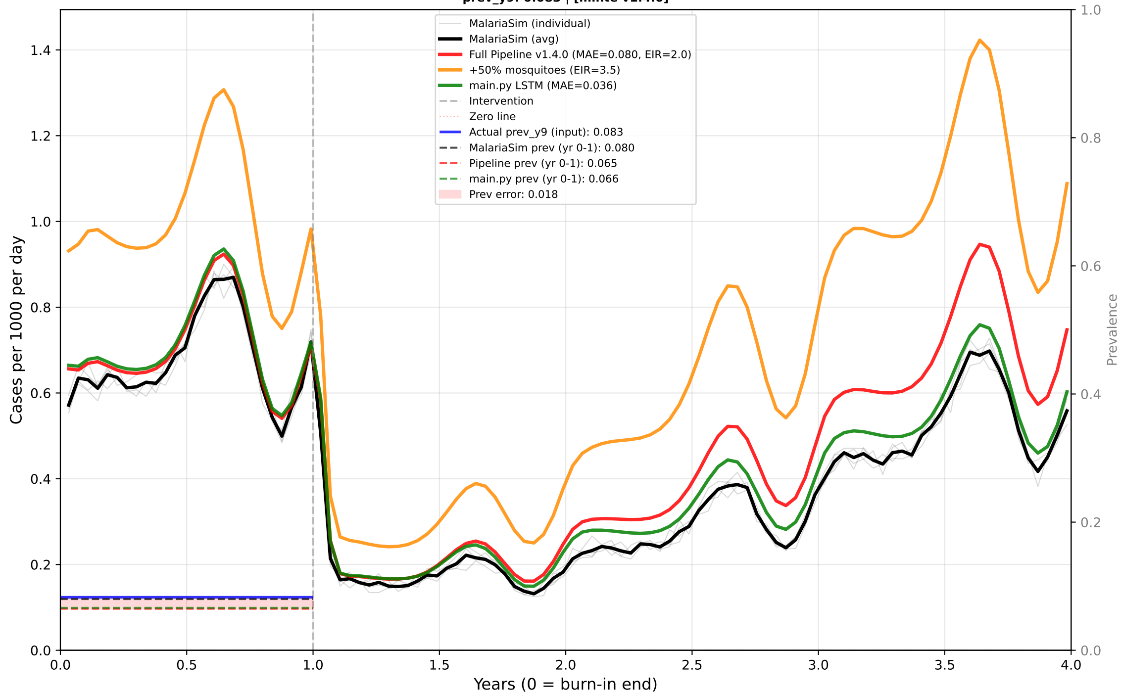
Case 10: Perennial - ITN Only - Low EIR - Mid dn0 Predictor: CASES | True EIR: 2.1 | Est EIR: 2.0 prev_y9: 0.083 | [minte v1.4.0]
