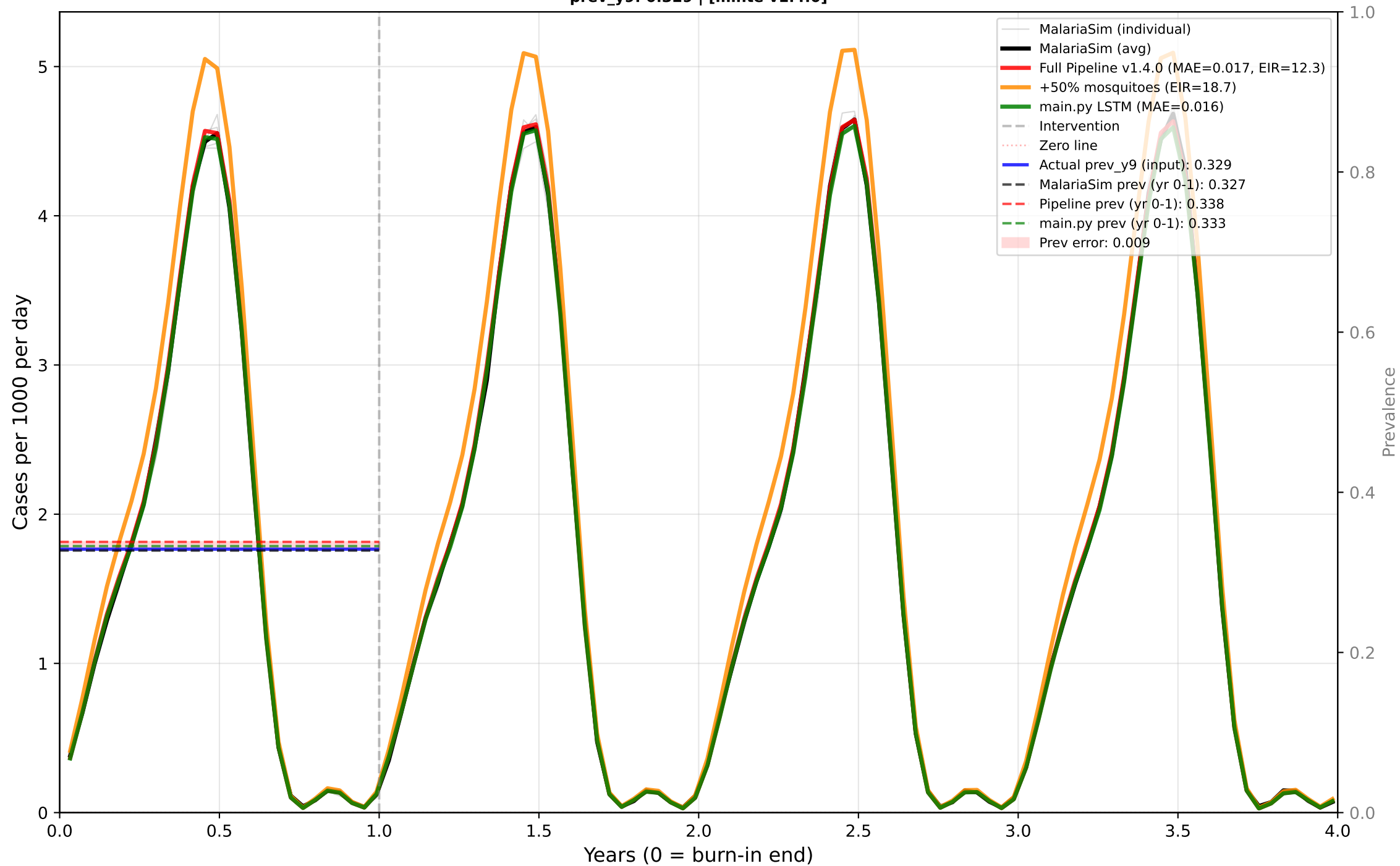
Case 5: Seasonal - No Intervention - Mid EIR Predictor: CASES | True EIR: 11.9 | Est EIR: 12.3 prev_y9: 0.329 | [minte v1.4.0]
