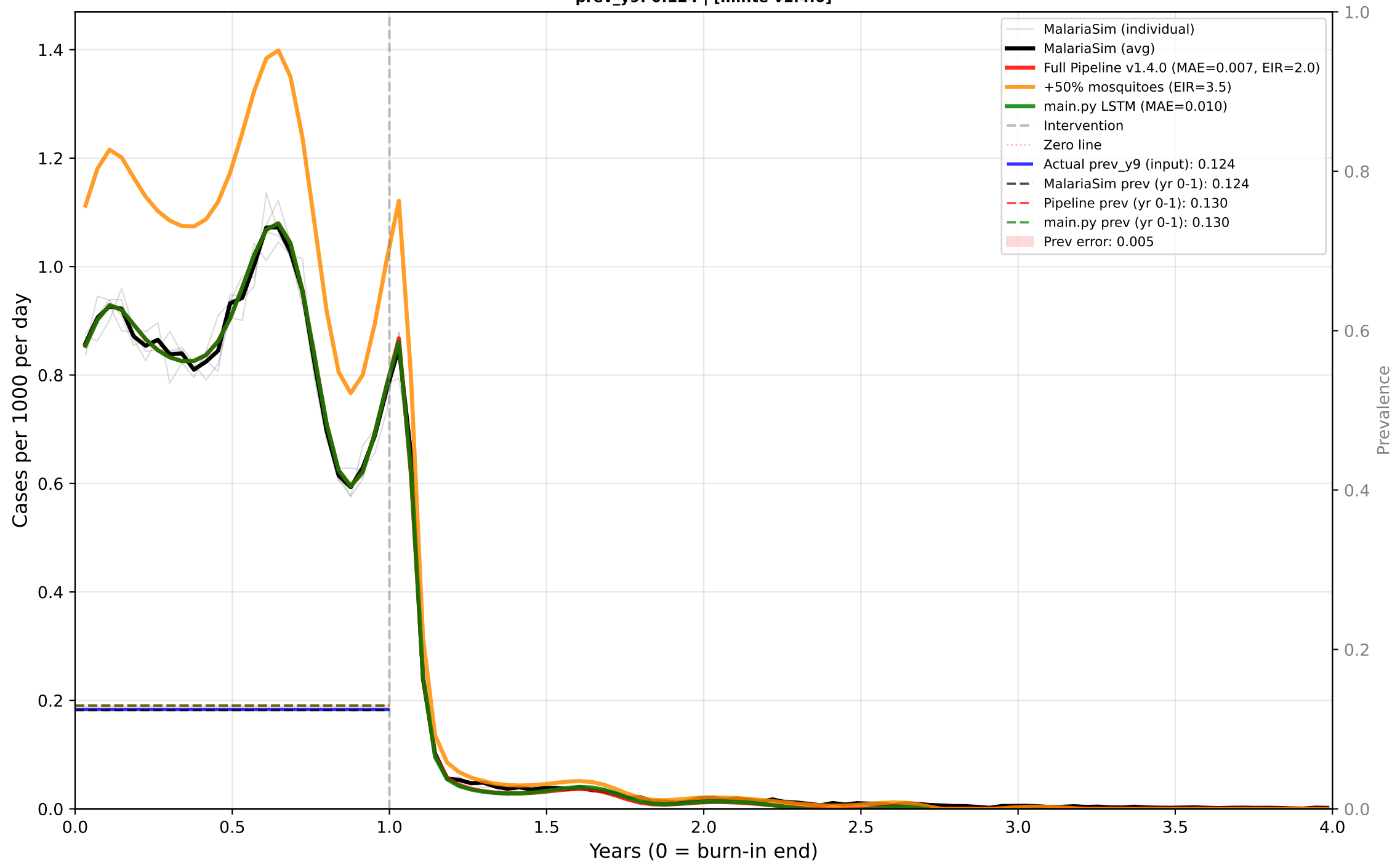
Case 23: Perennial - LSM Only - Low EIR Predictor: CASES | True EIR: 2.0 | Est EIR: 2.0 prev_y9: 0.124 | [minte v1.4.0]
