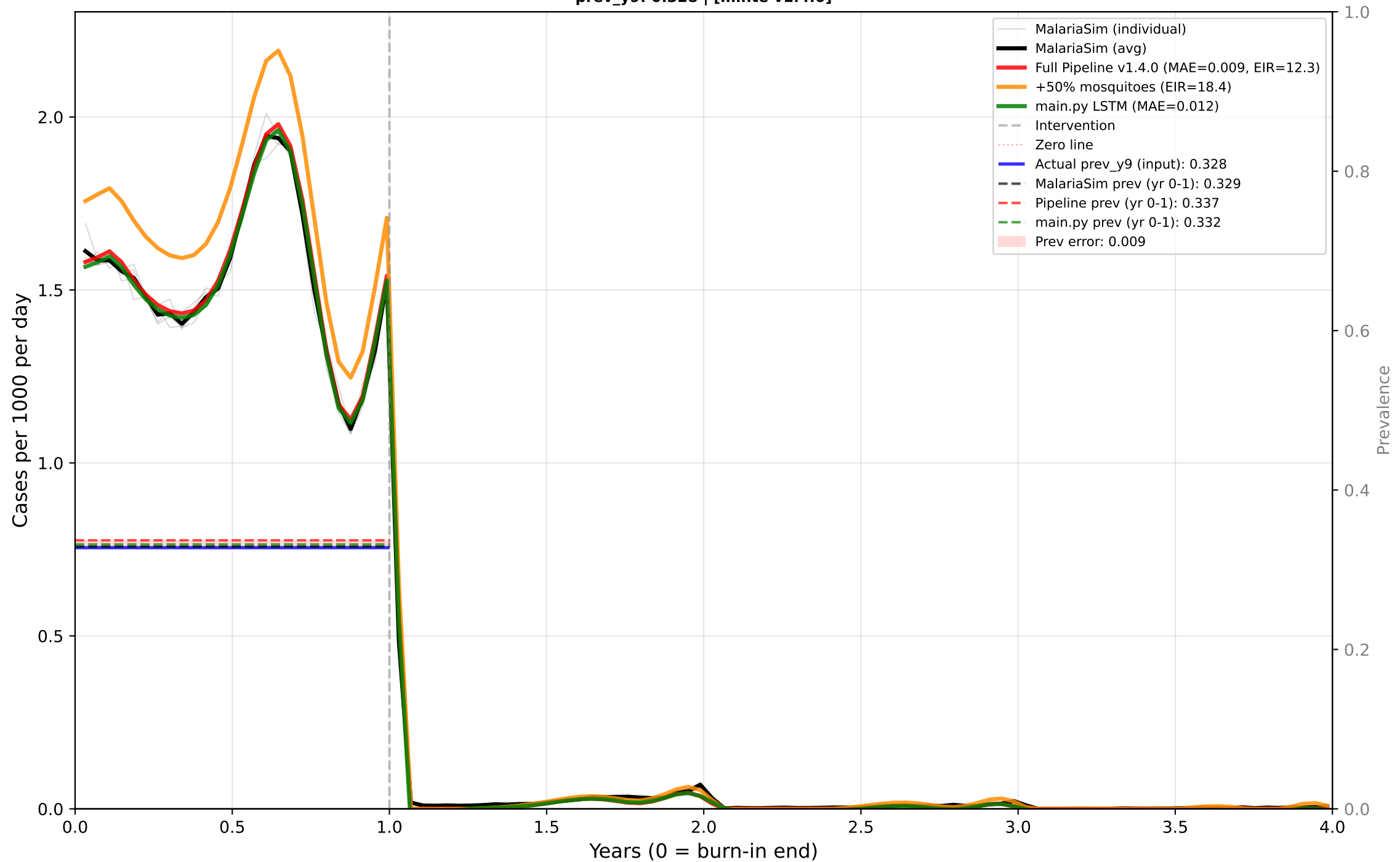
Case 36: Perennial - IRS+LSM - Mid EIR Predictor: CASES | True EIR: 11.9 | Est EIR: 12.3 prev_y9: 0.328 | [minte v1.4.0]
