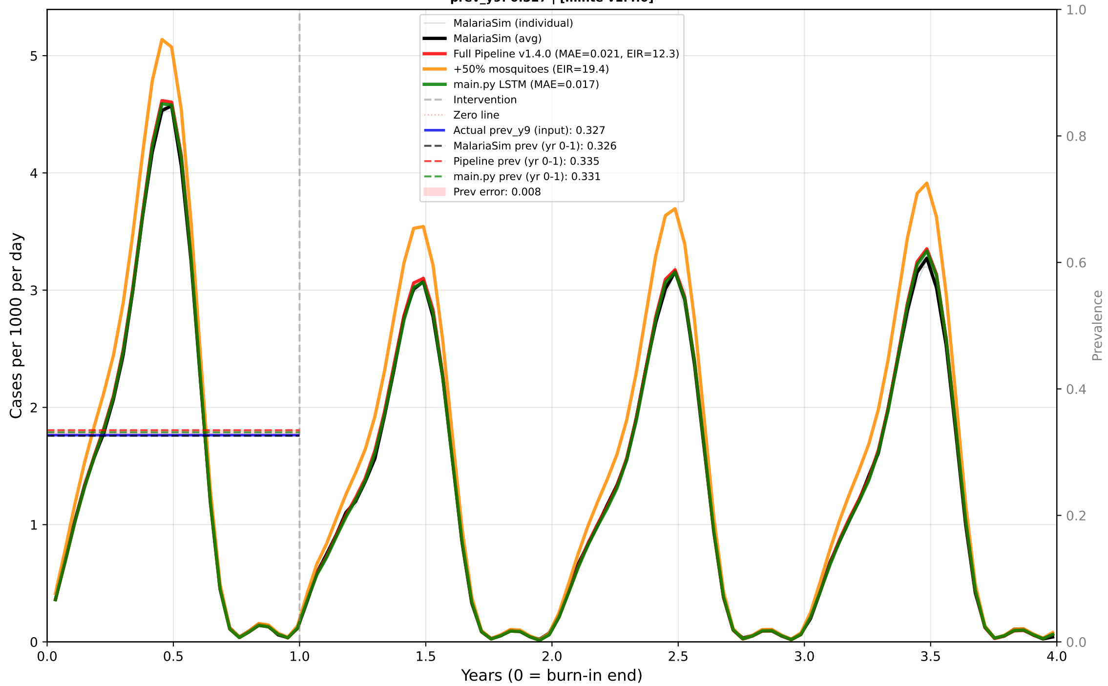
Case 26: Seasonal - LSM Only - Mid EIR Predictor: CASES | True EIR: 12.1 | Est EIR: 12.3 prev_y9: 0.327 | [minte v1.4.0]
