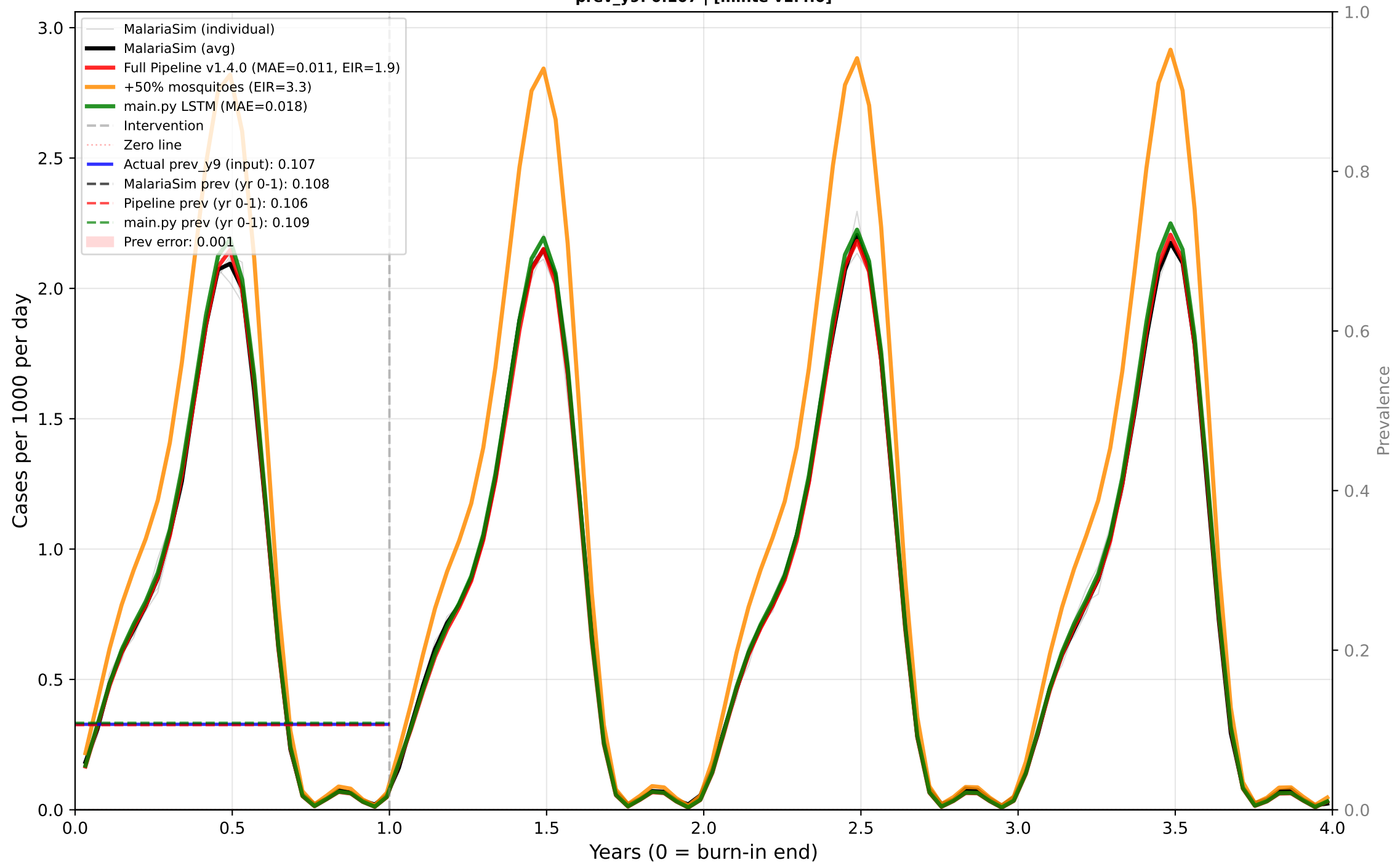
Case 4: Seasonal - No Intervention - Low EIR Predictor: CASES | True EIR: 2.0 | Est EIR: 1.9 prev_y9: 0.107 | [minte v1.4.0]
