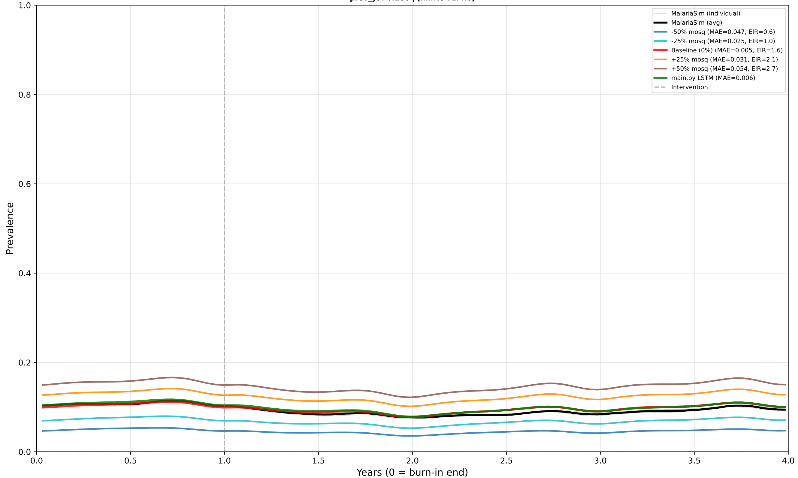
Case 7: Perennial - ITN Only - Low EIR - Low dn0 Predictor: PREVALENCE | True EIR: 1.7 | Est EIR (0%): 1.6 prev_y9: 0.106 | [minte v1.4.0]
