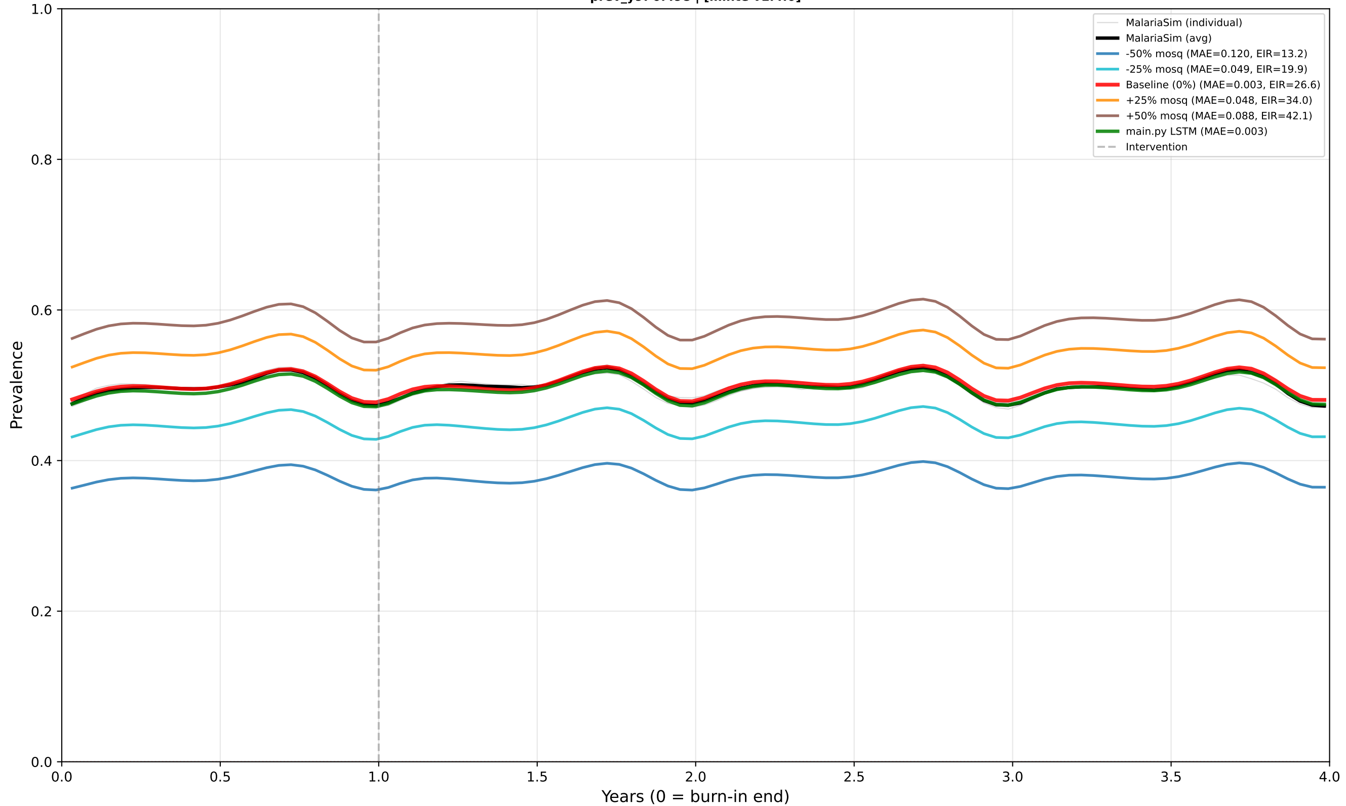
Case 3: Perennial - No Intervention - High EIR Predictor: PREVALENCE | True EIR: 25.7 | Est EIR (0%): 26.6 prev_y9: 0.498 | [minte v1.4.0]
