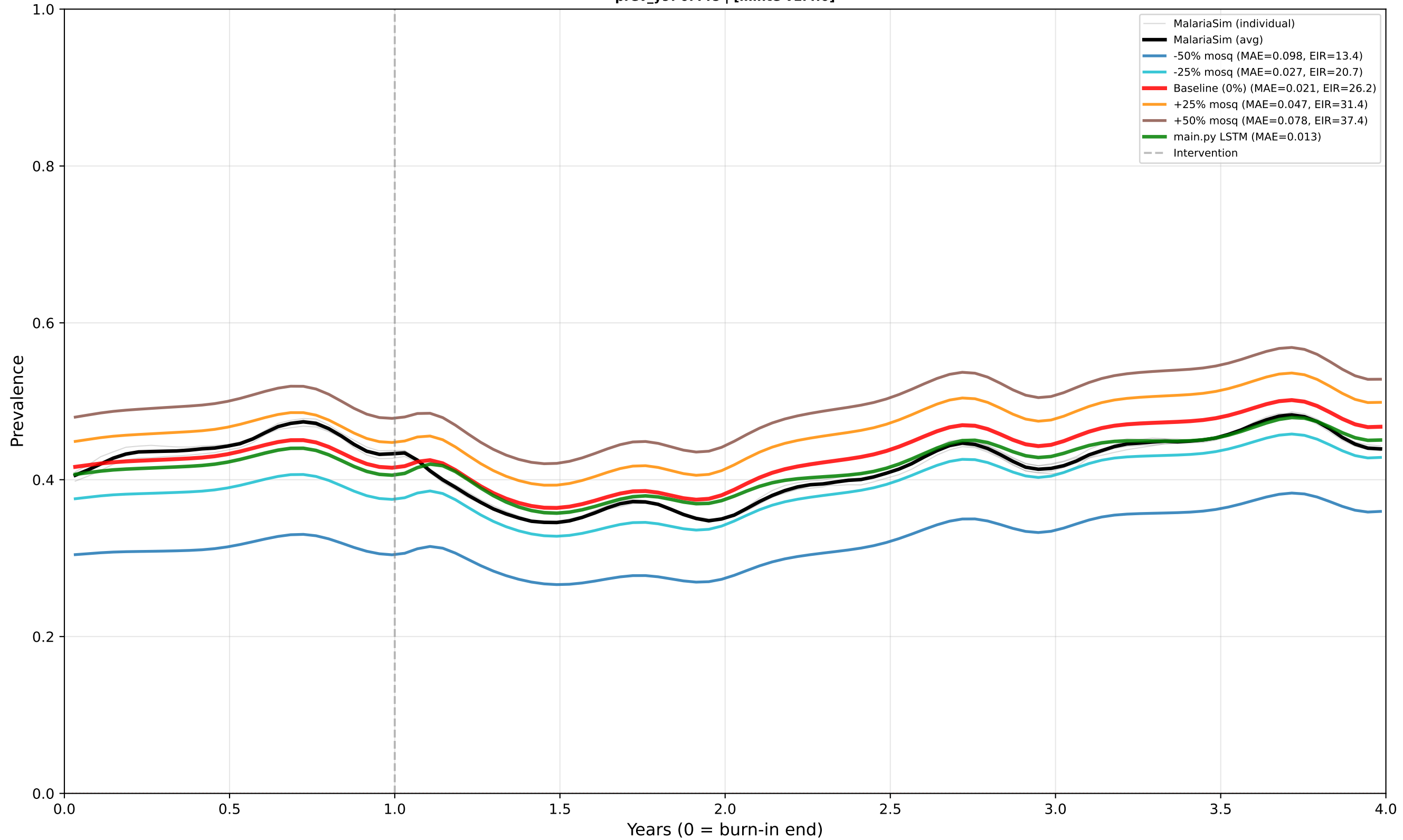
Case 9: Perennial - ITN Only - High EIR - Low dn0 Predictor: PREVALENCE | True EIR: 24.8 | Est EIR (0%): 26.2 prev_y9: 0.448 | [minte v1.4.0]
