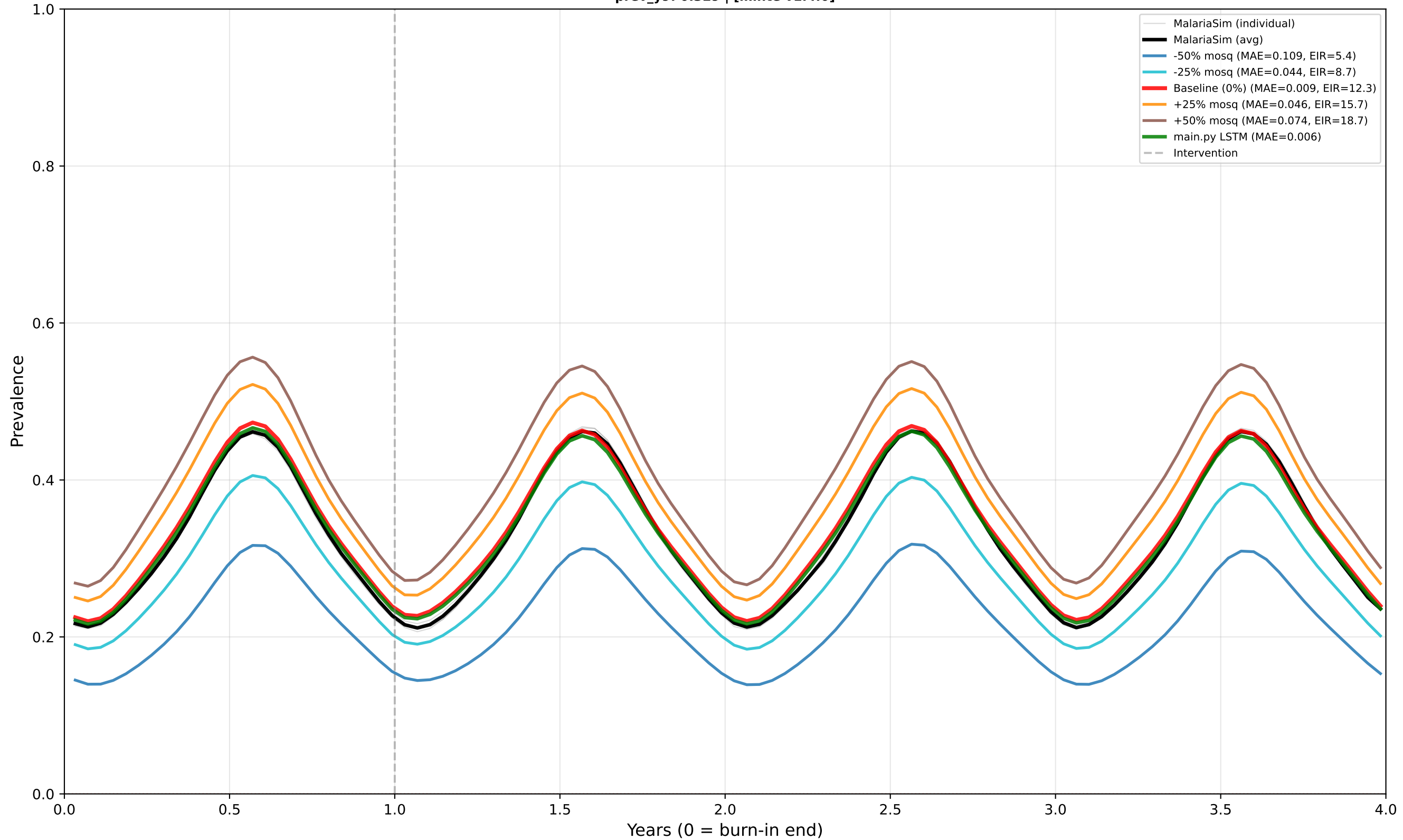
Case 5: Seasonal - No Intervention - Mid EIR Predictor: PREVALENCE | True EIR: 11.9 | Est EIR (0%): 12.3 prev_y9: 0.329 | [minte v1.4.0]
