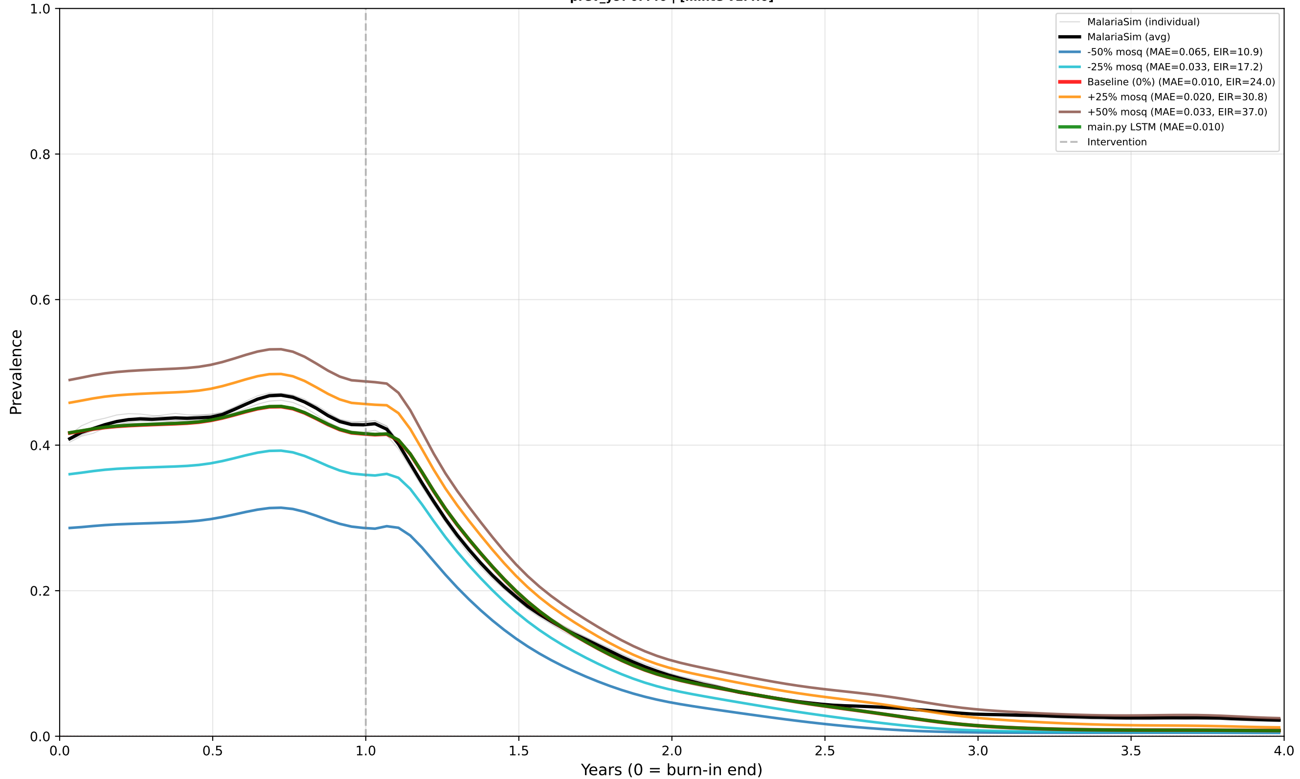
Case 33: Perennial - ITN+LSM - High EIR - High dn0 Predictor: PREVALENCE | True EIR: 24.1 | Est EIR (0%): 24.0 prev_y9: 0.440 | [minte v1.4.0]
