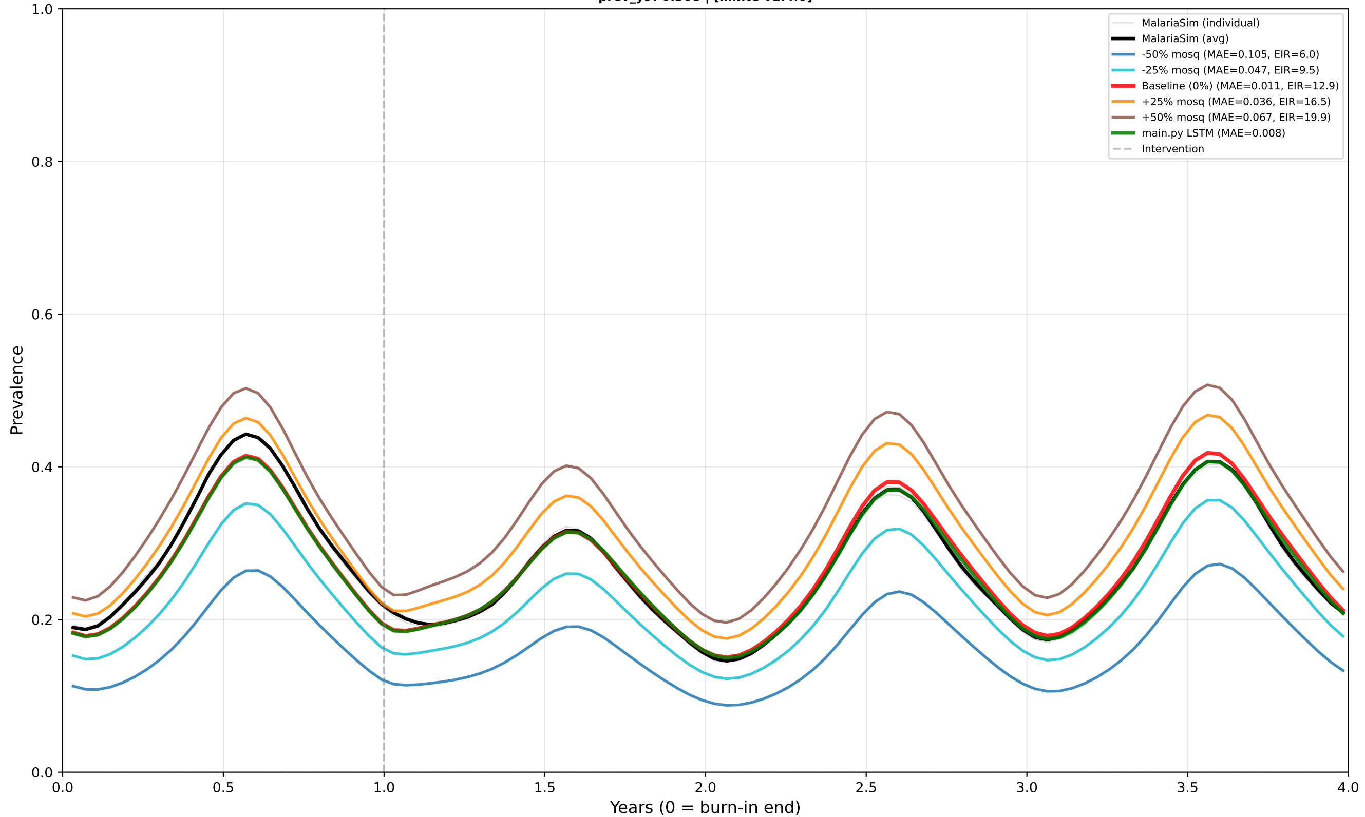
Case 34: Seasonal - ITN+LSM - Mid EIR - Mid dn0 Predictor: PREVALENCE | True EIR: 12.8 | Est EIR (0%): 12.9 prev_y9: 0.308 | [minte v1.4.0]
