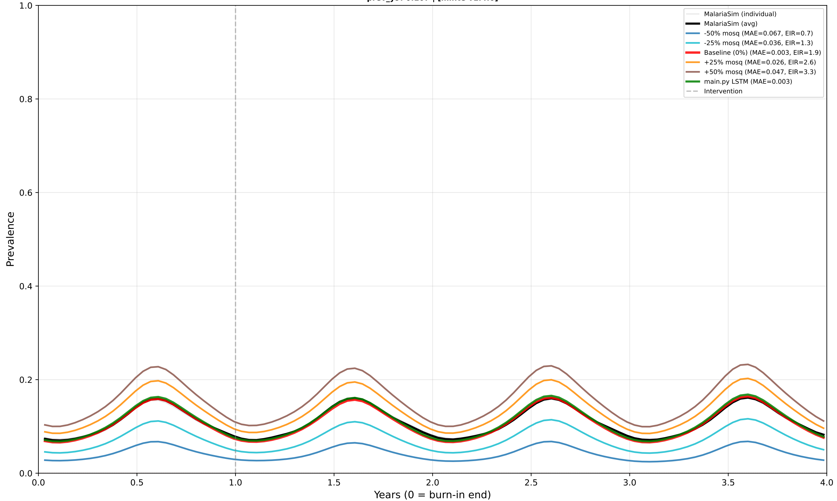
Case 4: Seasonal - No Intervention - Low EIR Predictor: PREVALENCE | True EIR: 2.0 | Est EIR (0%): 1.9 prev_y9: 0.107 | [minte v1.4.0]
