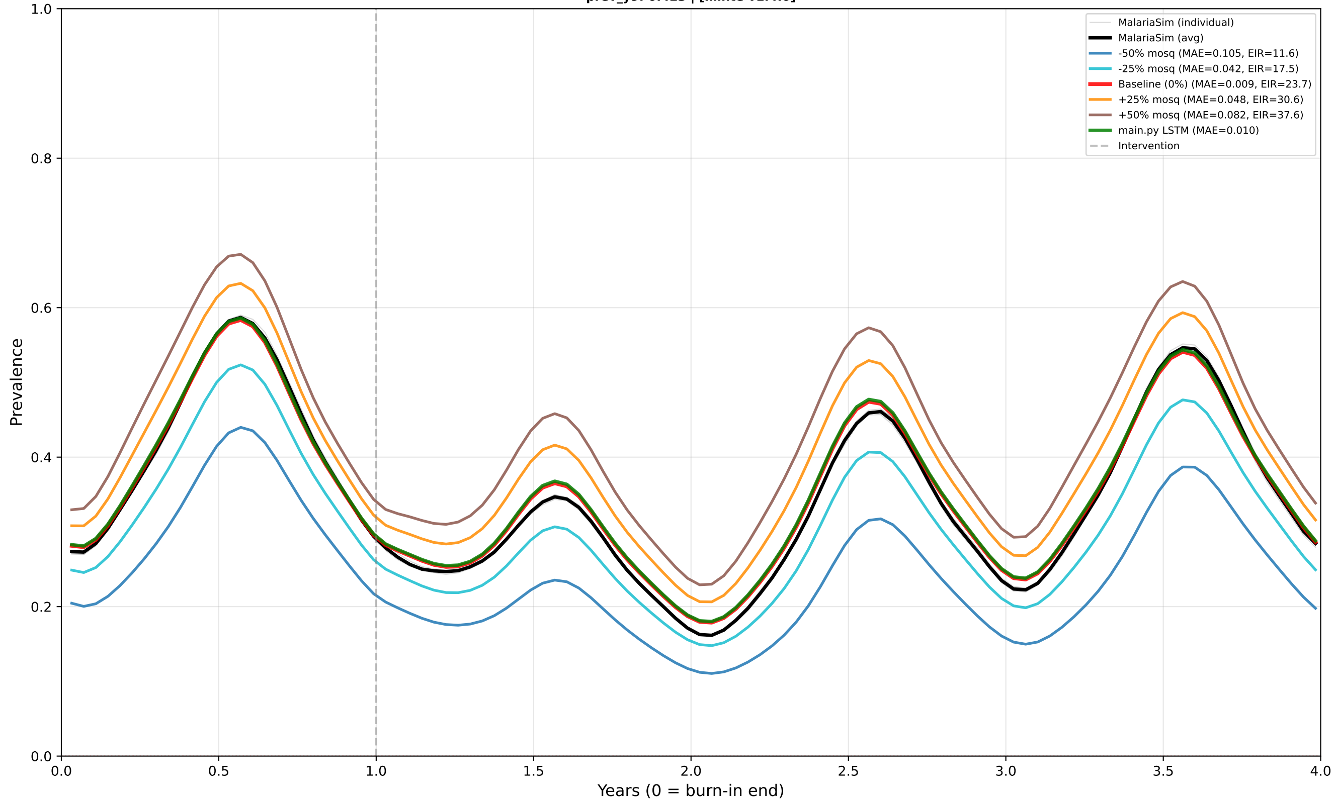
Case 18: Seasonal - ITN Only - High EIR - High dn0 Predictor: PREVALENCE | True EIR: 24.1 | Est EIR (0%): 23.7 prev_y9: 0.423 | [minte v1.4.0]
