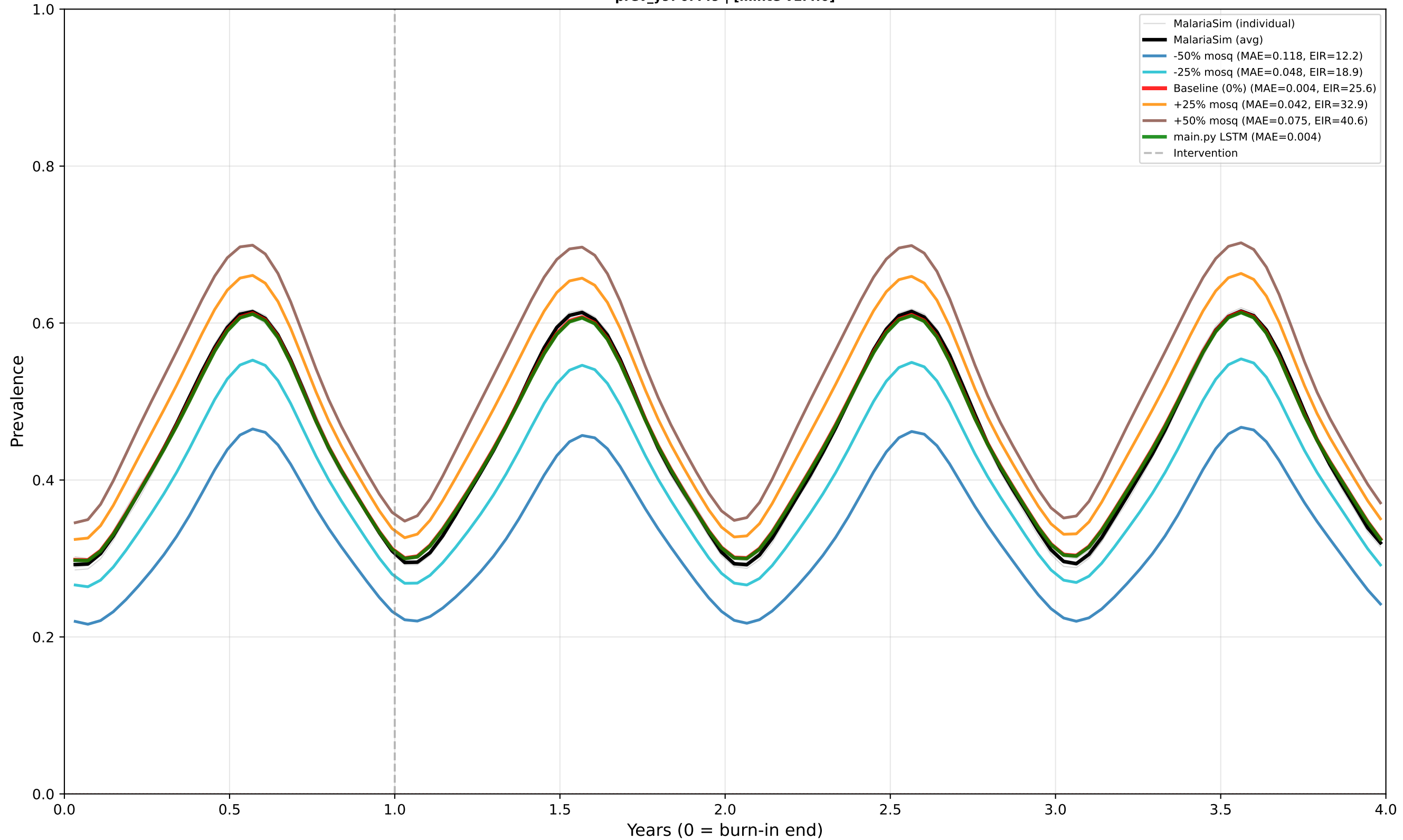
Case 6: Seasonal - No Intervention - High EIR Predictor: PREVALENCE | True EIR: 25.4 | Est EIR (0%): 25.6 prev_y9: 0.449 | [minte v1.4.0]
