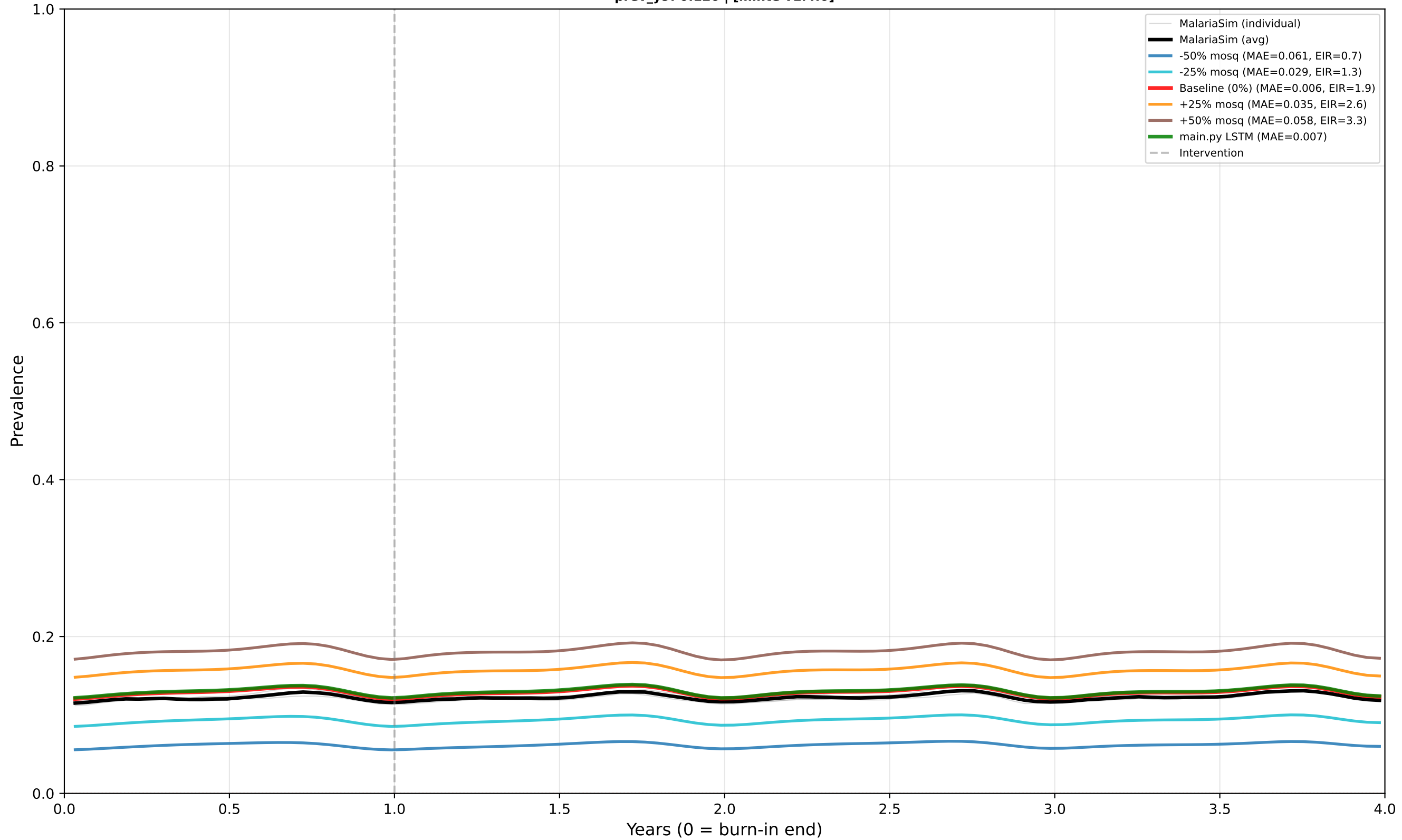
Case 1: Perennial - No Intervention - Low EIR Predictor: PREVALENCE | True EIR: 2.0 | Est EIR (0%): 1.9 prev_y9: 0.120 | [minte v1.4.0]
