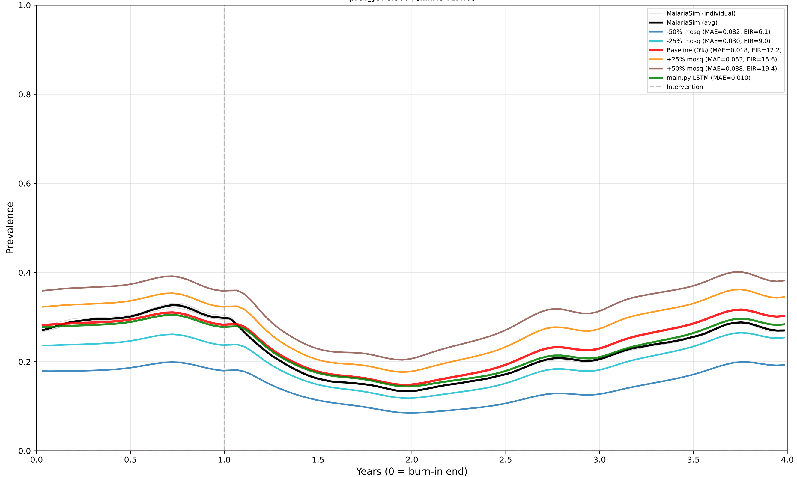
Case 11: Perennial - ITN Only - Mid EIR - Mid dn0 Predictor: PREVALENCE | True EIR: 11.8 | Est EIR (0%): 12.2 prev_y9: 0.306 | [minte v1.4.0]
