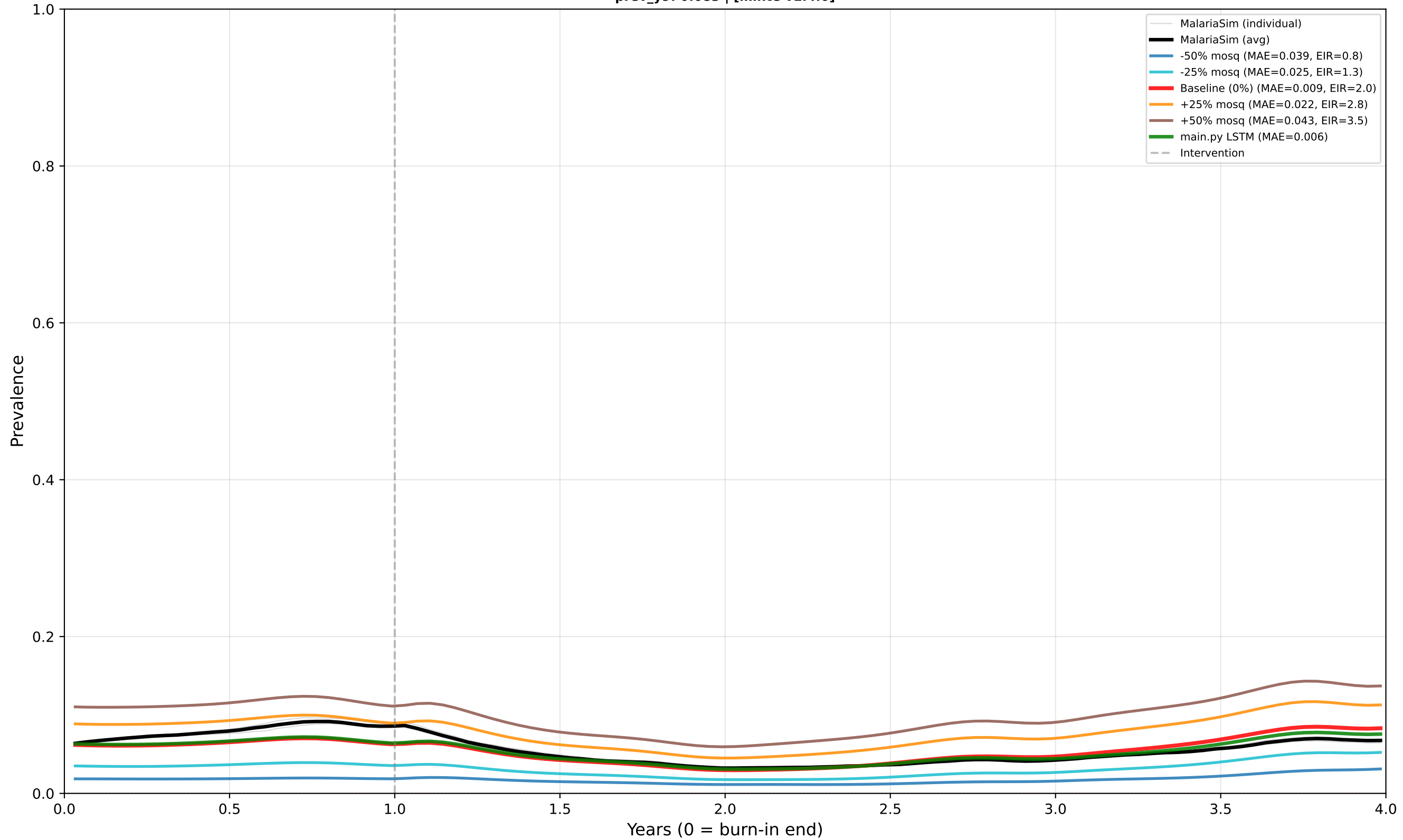
Case 10: Perennial - ITN Only - Low EIR - Mid dn0 Predictor: PREVALENCE | True EIR: 2.1 | Est EIR (0%): 2.0 prev_y9: 0.083 | [minte v1.4.0]
