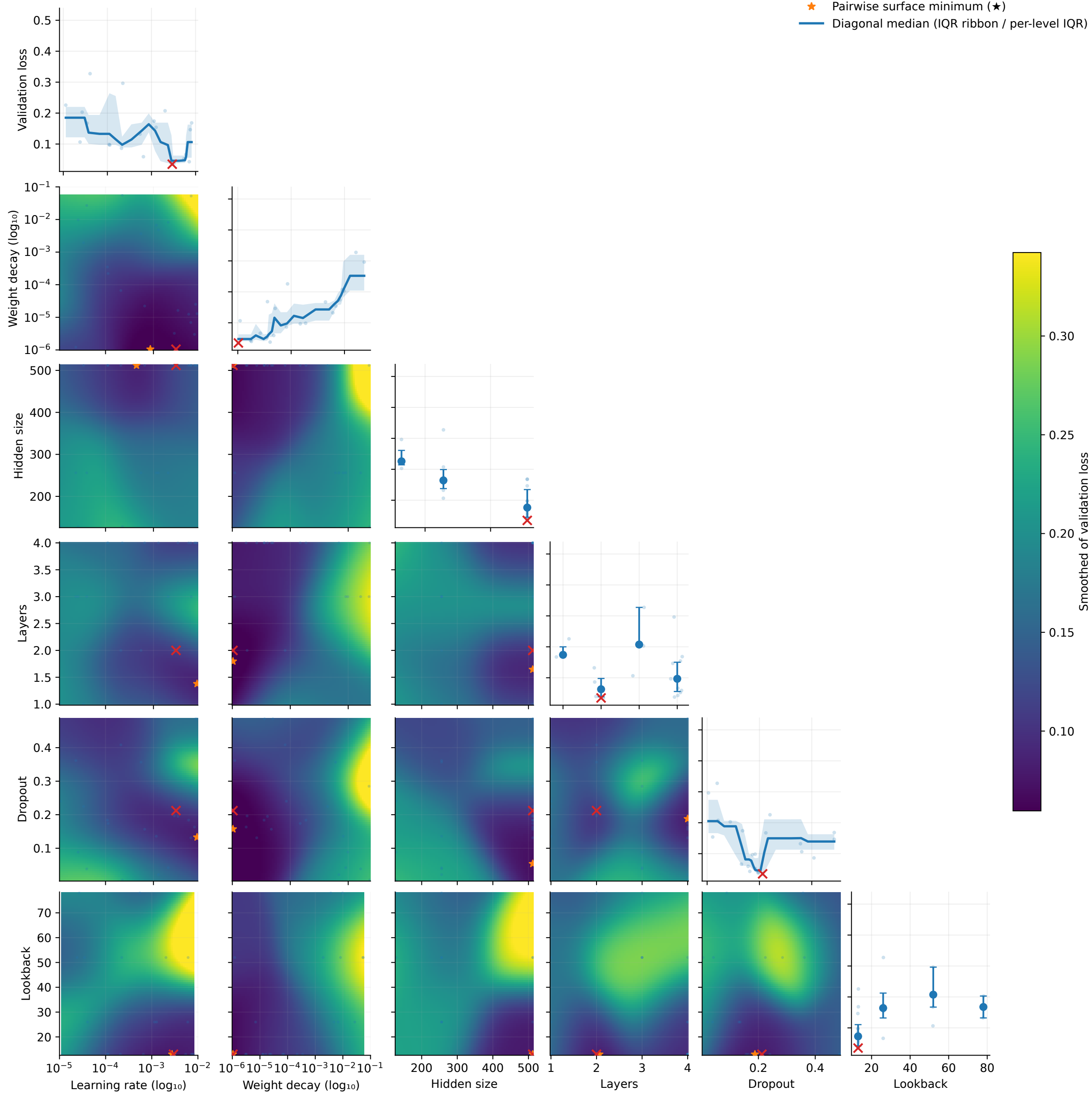
Cases — GRU • Hyperparameter sensitivity matrix (kernel-smoothed validation loss)
