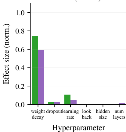
Hyperparameter effects (GRU vs LSTM) PDP (norm.)
