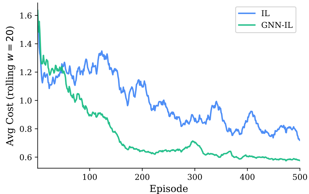
M = 10 : Moderate Coordination Regime
