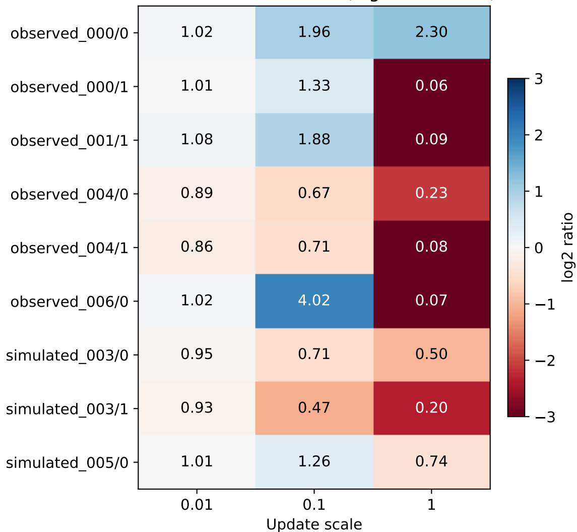
ESS fraction / reference (higher is better)
