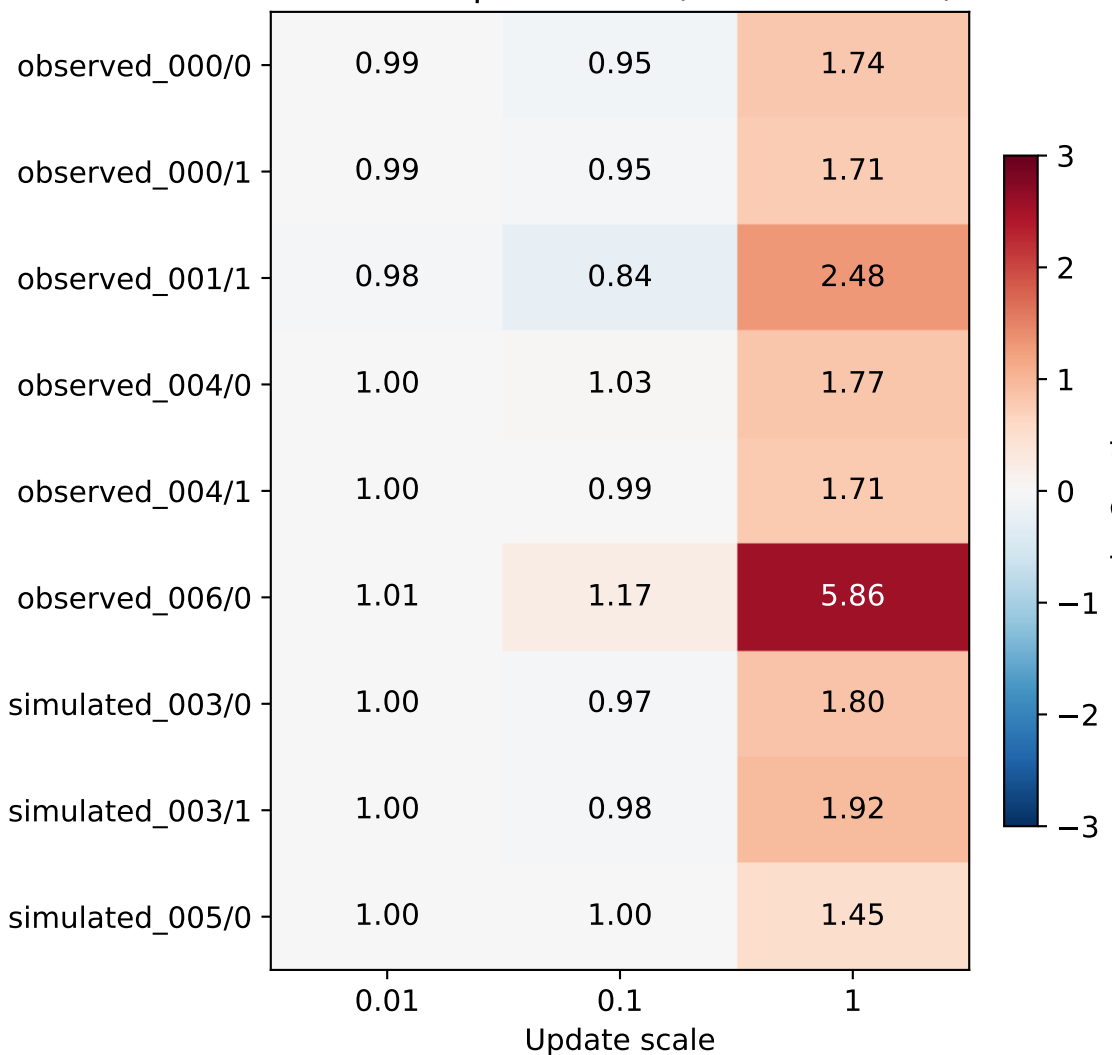
RMS / no-update RMS (lower is better)
