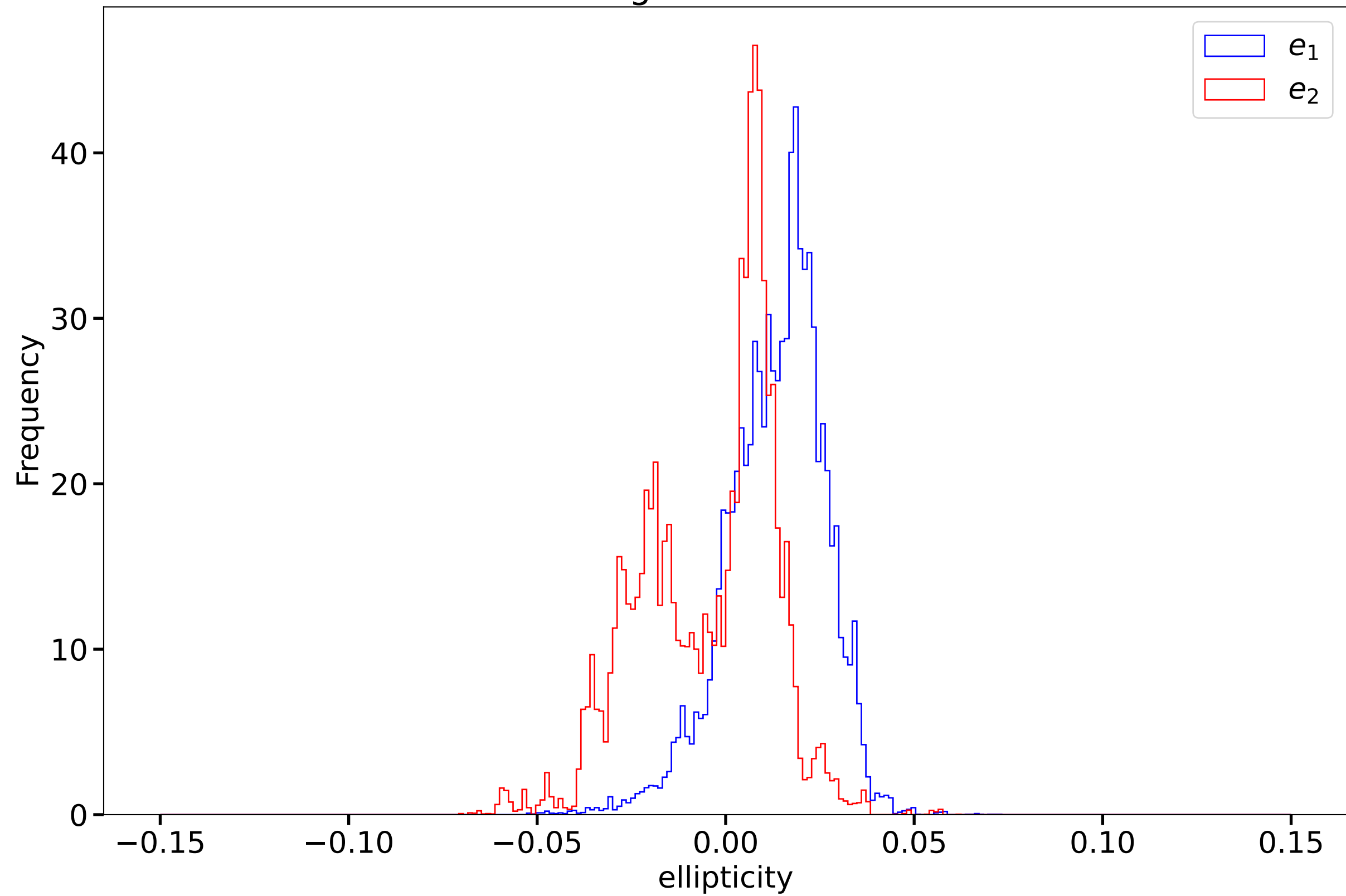
galsim PSF
