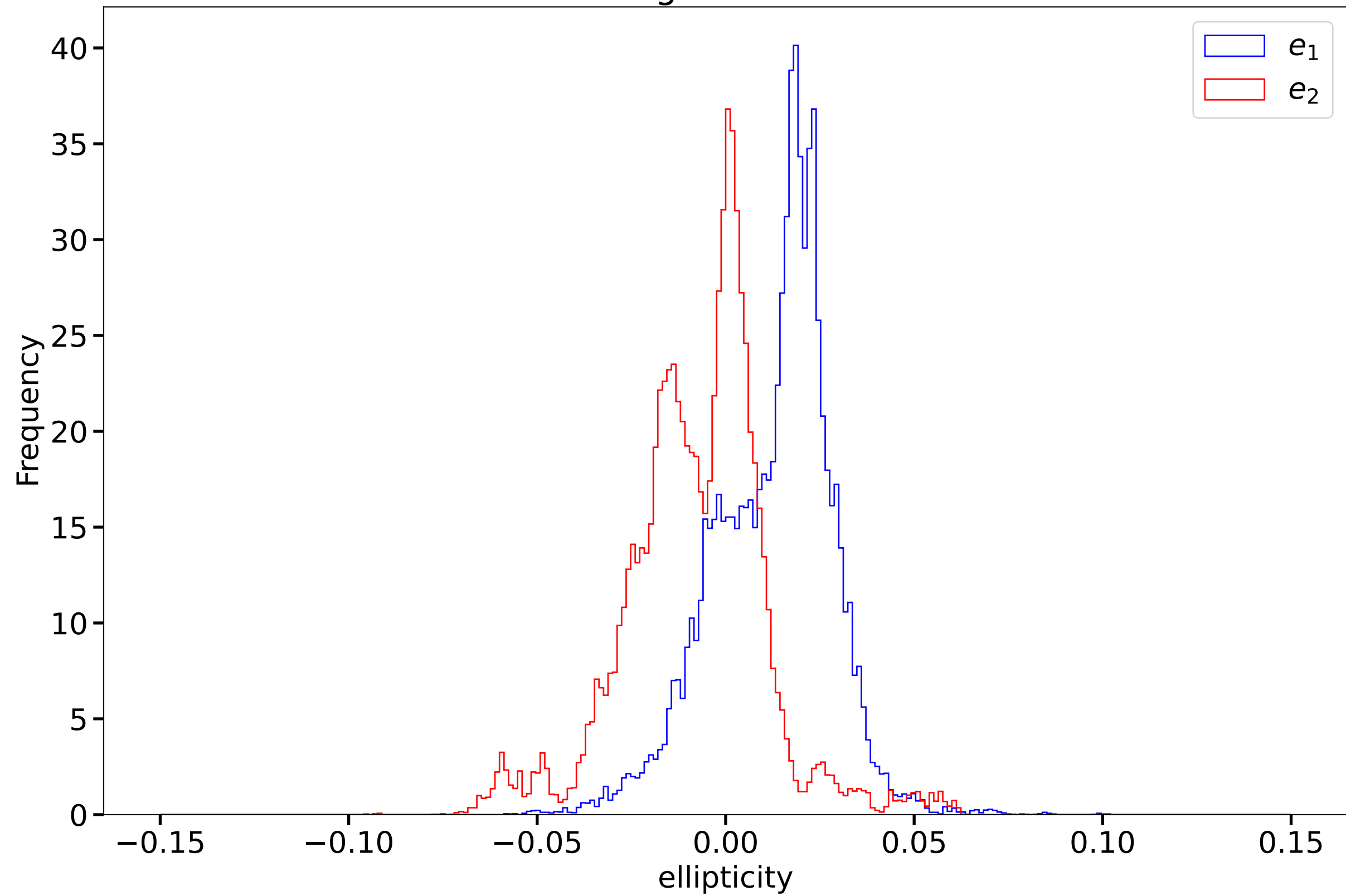
ngmix PSF
