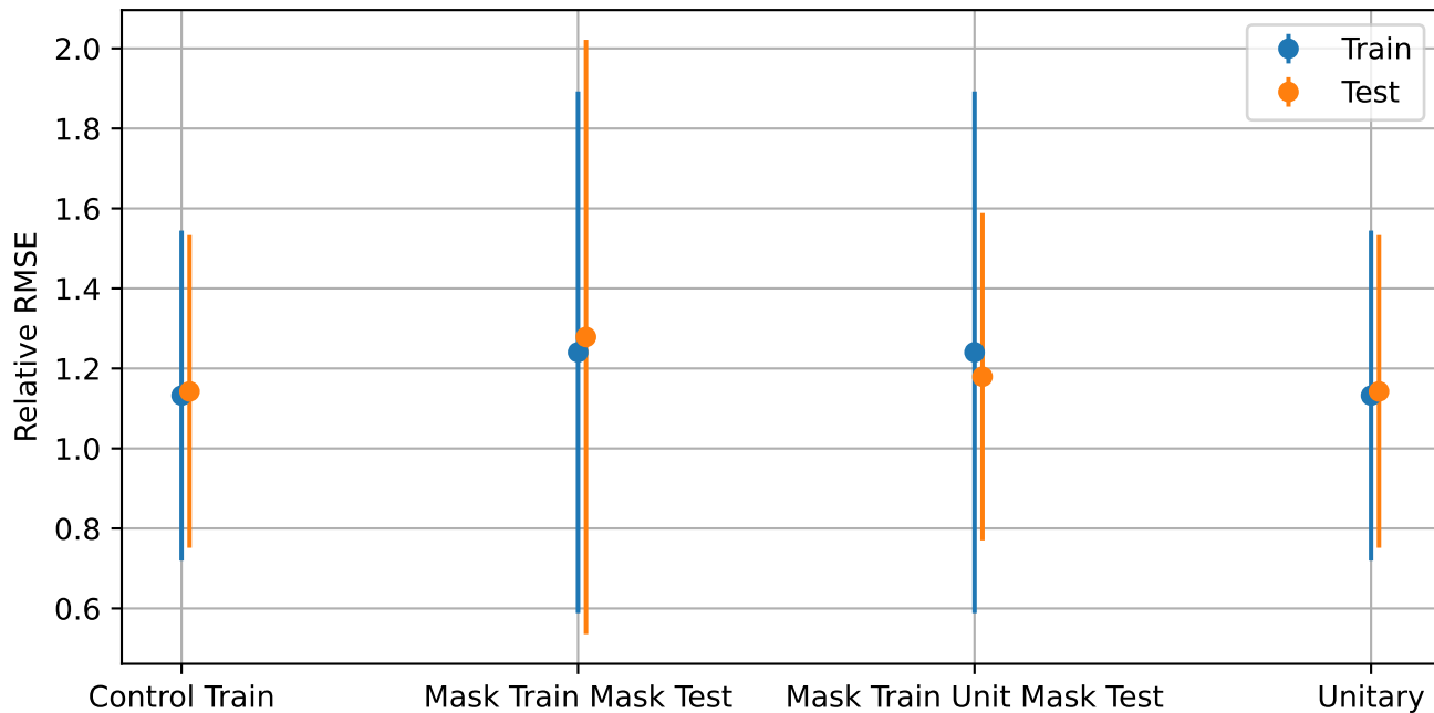
Relative RMSE 1x - Train and Test dataset
