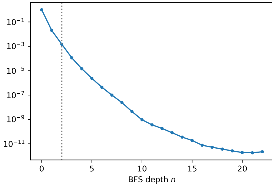
\sigma_{\text{pair}}(n) (B-frequency count), q = 101
