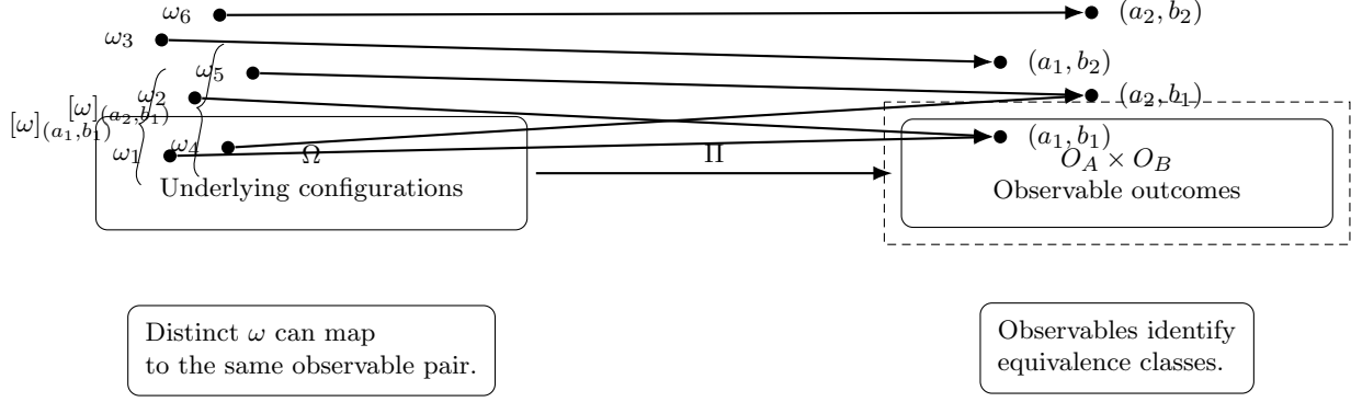
Fig. 1 Schematic non-injective projection from the underlying configuration space \Omega to the observable outcome space O_A \times O_B . Multiple underlying configurations correspond to the same observable pair (a, b) , defining equivalence classes. This many-to-one identification induces a generic failure of probabilistic factorization at the observable level without requiring nonlocal dynamics.
