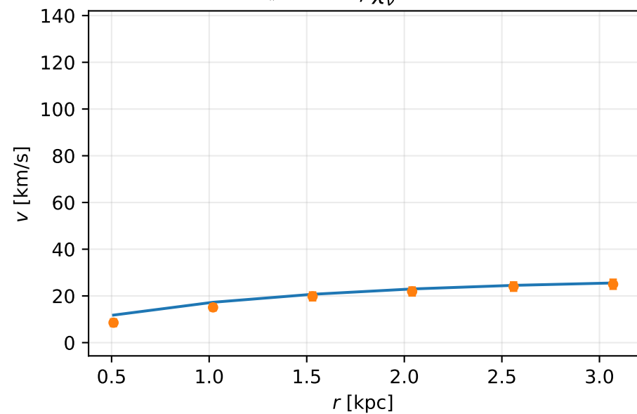
D564-8 Y_* = 0.05, \chi^2_\nu = 1.54
