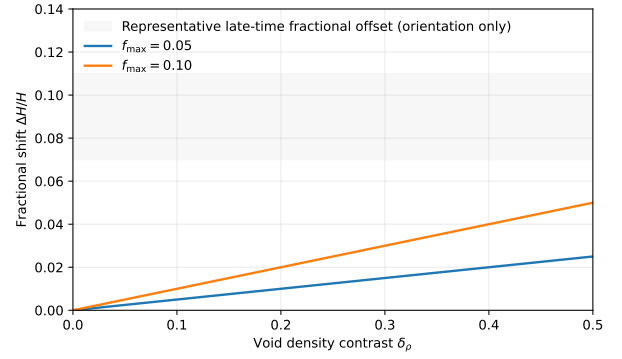
Figure 3. Quantitative visualization of the void inference bias implied by Eq. (8) in the deep-saturation regime ( g_{\text{void}} \ll a_\star ), where f(g_{\text{void}}/a_\star) \rightarrow f_{\text{max}} and \Delta H/H \simeq \delta_\rho f_{\text{max}} (Eq. (11)). Curves show representative values f_{\text{max}} = 0.05 and f_{\text{max}} = 0.10 , consistent with the independent bound discussed in the text. The shaded horizontal band indicates a representative range of late-time fractional offsets reported in the literature, shown for orientation only and not used for calibration.
