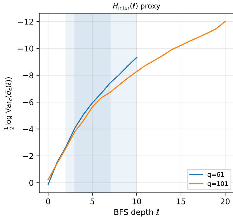
[O-2] numerical test — H(\sigma(\ell) \mid c) monotonicity
