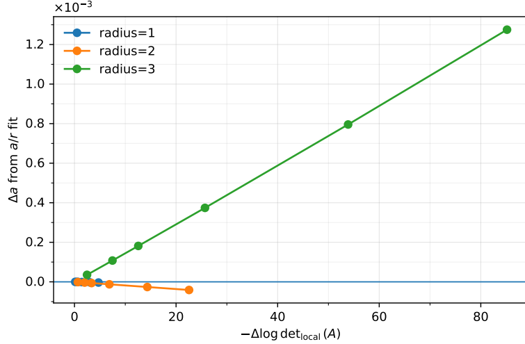
Fig. 1 Shift of the fitted Newtonian amplitude \Delta a as a function of -\Delta \log \det\{A\} for perturbations of increasing spatial radius R . Only sufficiently extended perturbations produce a macroscopic long-range response.
