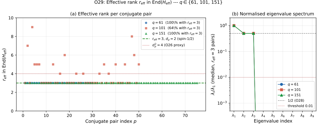
Figure 1: (a) Effective rank r_{\text{eff}}^{(A)} in \text{End}(H_{\text{eff}}) = \text{End}(\mathbb{C}^3) per conjugate pair (c, q-c) , for q \in \{61, 101, 151\} (reproduced from the o29_rank_computation.py pipeline). The dashed green line marks r_{\text{eff}} = 3 , the symmetric rank formula prediction for d_\rho = 2 (spin- \frac{1}{2} ). At q = 61 (30/30 pairs) and q = 151 (75/75 pairs), r_{\text{eff}} = 3 holds universally with zero inter-pair variance. At q = 101 , r_{\text{eff}} = 3 is the modal result (64% of pairs); anomalous pairs are confirmed as single-sample Monte Carlo artefacts by a multi-sample analysis (Remark 6.1). (b) Median normalised eigenvalue spectrum \lambda_i/\lambda_1 in \text{End}(H_{\text{eff}}) , computed over all r_{\text{eff}}^{(A)} = 3 pairs at each prime. The two subleading eigenvalues satisfy \lambda_2/\lambda_1 \approx \lambda_3/\lambda_1 \approx \frac{1}{2} , confirming the invariant structure [\lambda_1 : \lambda_2 : \lambda_3] = [1 : \frac{1}{2} : \frac{1}{2}] of O28 [7]. Eigenvalues \lambda_4, \dots, \lambda_9 lie below the 1% threshold (dotted red line) by more than two orders of magnitude.
