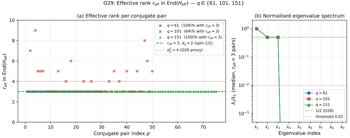
Figure 1: (a) Effective rank r_{\text{eff}}^{(A)} in \text{End}(H_{\text{eff}}) = \text{End}(\mathbb{C}^3) per conjugate pair (c, q-c) , for q \in \{61, 101, 151\} (reproduced from the o29_rank_computation.py pipeline). The dashed green line marks r_{\text{eff}} = 3 , the symmetric rank formula prediction for d_\rho = 2 (spin- \frac{1}{2} ). At q = 61 (30/30 pairs) and q = 151 (75/75 pairs), r_{\text{eff}} = 3 holds universally with zero inter-pair variance. At q = 101 , r_{\text{eff}} = 3 is the modal result (64% of pairs); anomalous pairs are attributed to atypical single-sample BFS trajectories (Remark 6.1). (b) Median normalised eigenvalue spectrum \lambda_i/\lambda_1 in \text{End}(H_{\text{eff}}) , computed over all r_{\text{eff}}^{(A)} = 3 pairs at each prime. The two subleading eigenvalues satisfy \lambda_2/\lambda_1 \approx \lambda_3/\lambda_1 \approx \frac{1}{2} , confirming the invariant structure [\lambda_1 : \lambda_2 : \lambda_3] = [1 : \frac{1}{2} : \frac{1}{2}] of O28 [7]. Eigenvalues \lambda_4, \dots, \lambda_9 lie below the 1% threshold (dotted red line) by more than two orders of magnitude.
