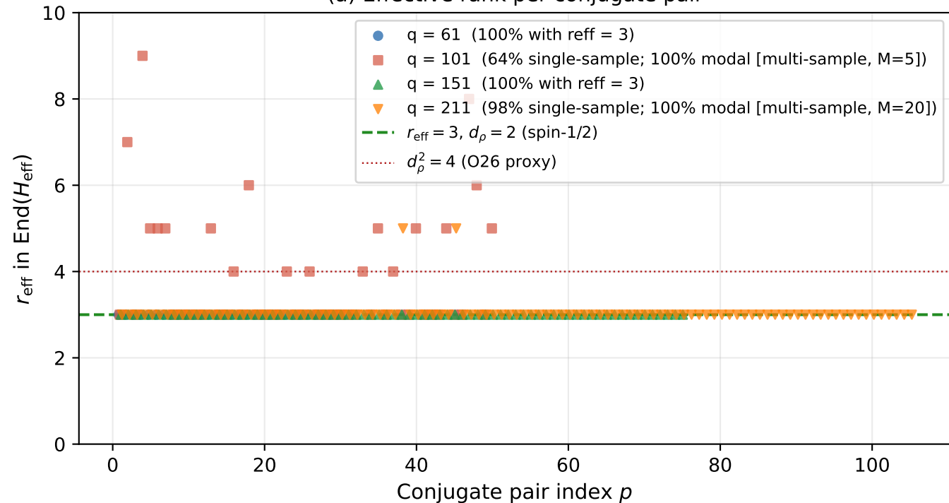
(a) Effective rank per conjugate pair
