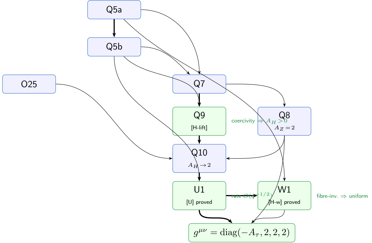
Figure 2: Geometric emergence sub-programme: logical chain from the continuum-limit hypotheses Q5a–Q5b to the effective Lorentzian co-metric. Q9 (proved) : [H-lift] is a theorem under Q5a; coercivity gives A_H > 0 independently of the bridge. Q8 (structural) : A_Z = C_{\mathfrak{su}(2)} = 2 by Casimir rigidity; normalisation fixed by horizontal sector. Q10 (structural) : universality [U] \Rightarrow \mathfrak{su}(2)\text{-isotropy} \Rightarrow A_H \rightarrow 2 , conditional on [U] . U1 (proved) : [U] proved with rate O(q^{-1/2}) from Weil-generator Lipschitz bound and BFS–Carnot–Carathéodory convergence (Q5b). W1 (proved) : [H-w] proved as a structural consequence of fibre-invariance ( \mathcal{O} = \text{Im } \Pi ), quantitative control from U1. The effective metric g^{\mu\nu} = \text{diag}(-A_\tau, 2, 2, 2) is established under the Q5a hypotheses.
