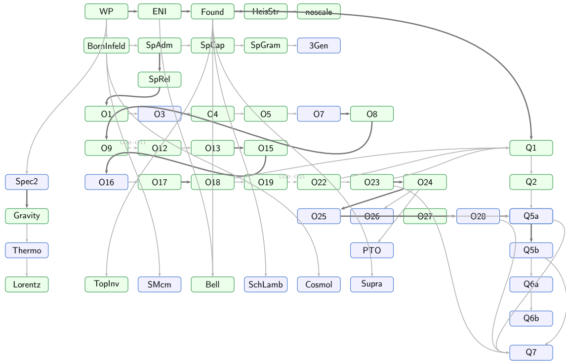
Figure 1: Logical dependency DAG of the Cosmochrony programme. Colour coding: ■ proved , ■ structural , ■ heuristic , ■ open . Thick arrows indicate the main logical spine; thin arrows indicate supporting dependencies. Dashed arrows with labels abbreviate linear sub-chains. The interactive version with clickable nodes is provided as a companion HTML file.
