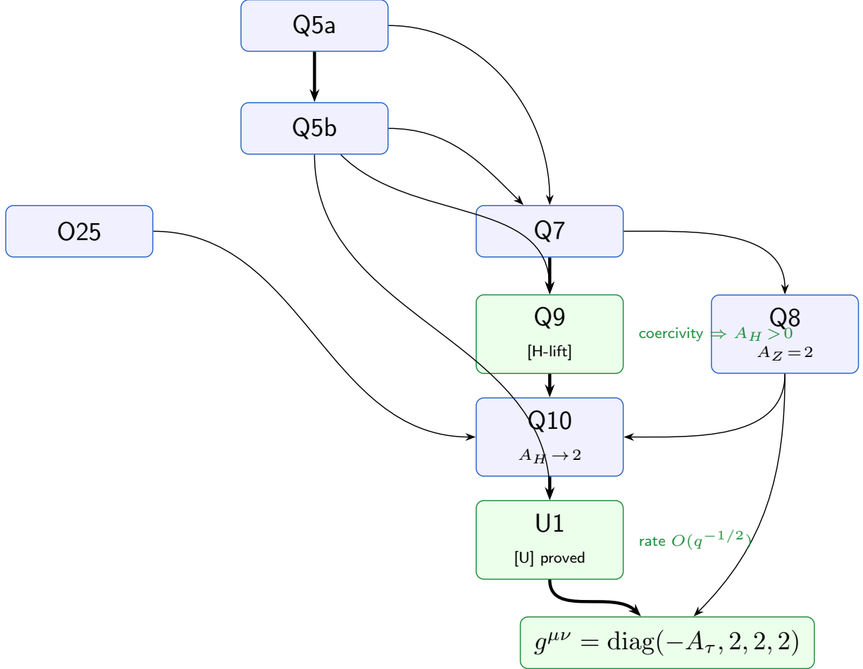
Figure 2: Geometric emergence sub-programme: logical chain from the continuum-limit hypotheses Q5a–Q5b to the effective Lorentzian co-metric. Q9 (proved) : [H-lift] is a theorem under Q5a; coercivity gives A_H > 0 independently of the bridge. Q8 (structural) : A_Z = C_{\mathfrak{su}(2)} = 2 by Casimir rigidity; normalisation fixed by horizontal sector. Q10 (structural) : universality [U] \Rightarrow \mathfrak{su}(2) -isotropy \Rightarrow A_H \rightarrow 2 , conditional on [U]. U1 (proved) : [U] proved with rate O(q^{-1/2}) from Weil-generator Lipschitz bound and BFS–Carnot–Carathéodory convergence (Q5b). The effective metric g^{\mu\nu} = \text{diag}(-A_\tau, 2, 2, 2) is established under the Q5a hypotheses.
