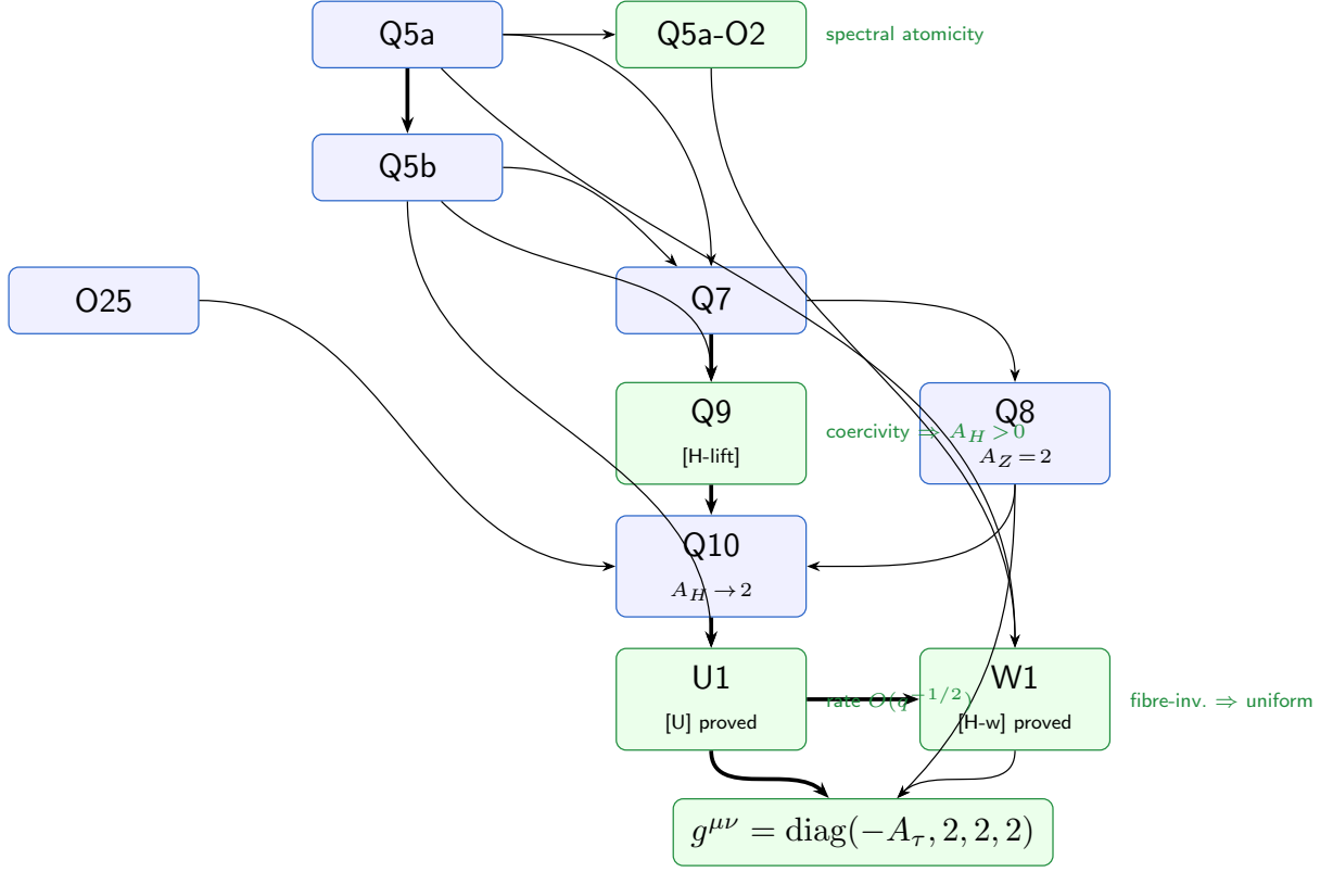
Figure 2: Geometric emergence sub-programme: logical chain from Q5a to the effective Lorentzian co-metric. Q5a-O2 [62] ( proved ): spectral atomicity of \text{ran}(\Pi_q) ; proves [H- \mathcal{E}1 ] and [C]; closes all Q5a hypotheses except [H2]. Q9 ( proved ): [H-lift] is a theorem under Q5a; coercivity gives A_H > 0 independently of the bridge. Q8 ( structural ): A_Z = C_{\mathfrak{su}(2)} = 2 by Casimir rigidity; normalisation fixed by horizontal sector. Q10 ( structural ): universality [U] \Rightarrow \mathfrak{su}(2) -isotropy \Rightarrow A_H \rightarrow 2 , conditional on [U]. U1 ( proved ): [U] proved with rate O(q^{-1/2}) from Weil-generator Lipschitz bound and BFS–Carnot–Carathéodory convergence (Q5b). W1 ( proved ): [H-w] proved as a structural consequence of fibre-invariance ( \mathcal{O} = \text{Im } \Pi ), quantitative control from U1. The effective metric g^{\mu\nu} = \text{diag}(-A_\tau, 2, 2, 2) is established under the Q5a hypotheses; [H2] is the sole remaining open hypothesis.
