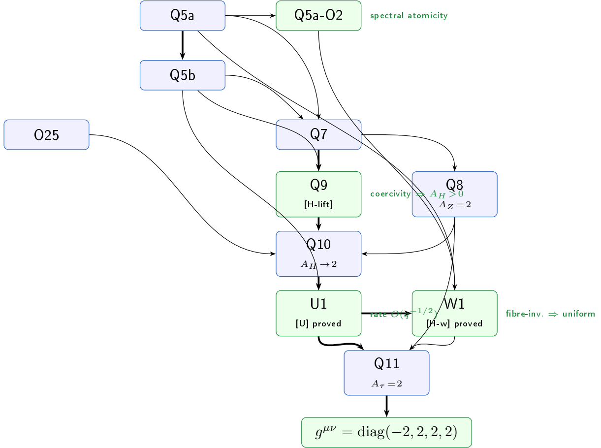
Figure 2: Geometric emergence sub-programme: logical chain from Q5a to the effective Lorentzian co-metric. Q5a-O2 [89] ( proved ): spectral atomicity of \text{ran}(\Pi_q) ; proves [H- \mathcal{E} 1] and [C]; closes all Q5a hypotheses except [H2]. Q9 ( proved ): [H-lift] is a theorem under Q5a; coercivity gives A_H > 0 independently of the bridge. Q8 ( structural ): A_Z = C_{\mathfrak{su}(2)} = 2 by Casimir rigidity; normalisation fixed by horizontal sector. Q10 ( structural ): universality [U] \Rightarrow \mathfrak{su}(2) -isotropy \Rightarrow A_H \rightarrow 2 , conditional on [U]. U1 ( proved ): [U] proved with rate O(q^{-1/2}) from Weil-generator Lipschitz bound and BFS–Carnot–Carathéodory convergence (Q5b). W1 ( proved ): [H-w] proved as a structural consequence of fibre-invariance ( \mathcal{O} = \text{Im } \Pi ), quantitative control from U1. The effective metric g^{\mu\nu} = \text{diag}(-A_\tau, 2, 2, 2) is established under the Q5a hypotheses; [H2] is the sole remaining open hypothesis.
