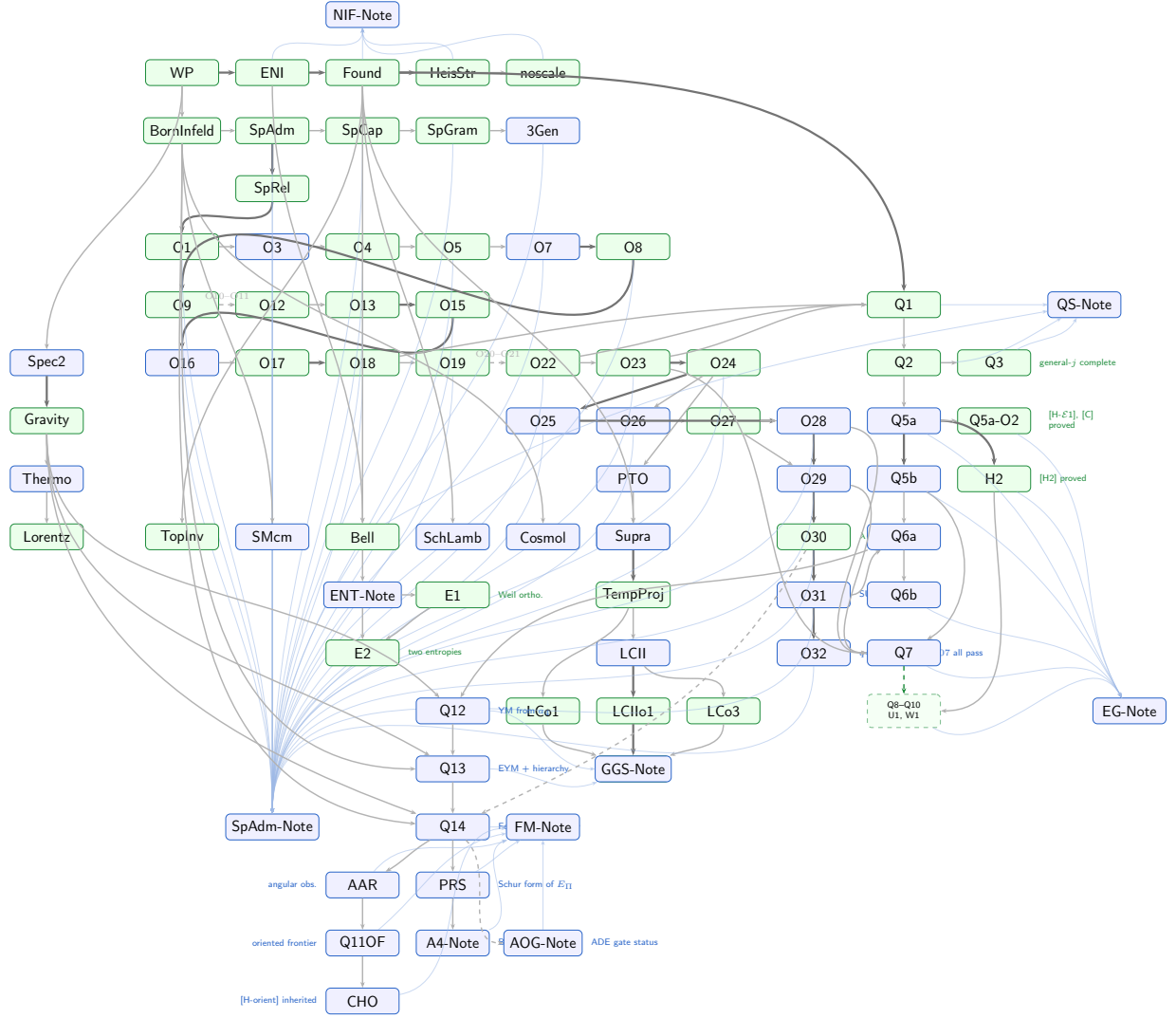
Figure 1: Logical dependency DAG of the Cosmochrony programme. Colour coding: ■ proved , ■ structural , ■ heuristic , ■ open . Thick arrows indicate the main logical spine; thin arrows indicate supporting dependencies. Dashed arrows with labels abbreviate linear sub-chains. The faint converging edges gather the constituent papers of each thematic sub-programme into its synthesis node: the Branch I foundational papers (ENI, Found, HeisStr, noscale) into NIF-Note , the spectral admissibility papers into SpAdm-Note , the Lorentz-capacity papers into LC-Synth , the geometric emergence papers into EG-Note , Q1/Q2/Q3 and the Bell paper into the quantum-structure QS-Note , Q12 and Q13 into the gauge-gravity stratification GGS-Note , and Q14 with the companion notes PRS, AAR, Q11OF, CHO, A4-Note and AOG-Note into the fermionic-matter FM-Note . The dashed green arrow from Q7 leads to the geometric emergence closure block Q8–Q10 and U1, W1, detailed in Figure 2. The interactive version with clickable nodes is provided as a companion HTML file.
