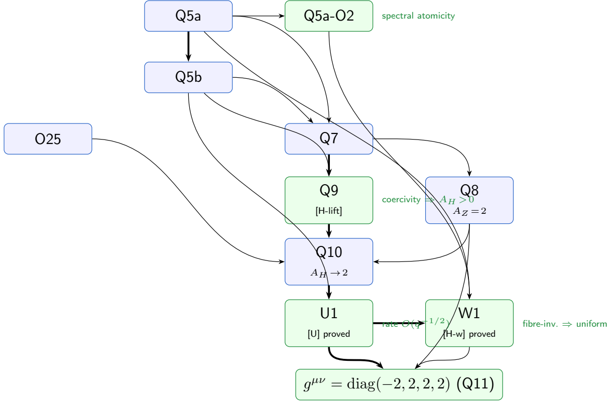
Figure 2: Geometric emergence sub-programme: logical chain from Q5a to the effective Lorentzian co-metric. Q5a-O2 [63] ( proved ): spectral atomicity of \text{ran}(\Pi_q) ; proves [H- \mathcal{E}1 ] and [C]; closes all Q5a hypotheses except [H2]. Q9 ( proved ): [H-lift] is a theorem under Q5a; coercivity gives A_H > 0 independently of the bridge. Q8 ( structural ): A_Z = C_{\mathfrak{su}(2)} = 2 by Casimir rigidity; normalisation fixed by horizontal sector. Q10 ( structural ): universality [U] \Rightarrow \mathfrak{su}(2) -isotropy \Rightarrow A_H \rightarrow 2 , conditional on [U]. U1 ( proved ): [U] proved with rate O(q^{-1/2}) from Weil-generator Lipschitz bound and BFS–Carnot–Carathéodory convergence (Q5b). W1 ( proved ): [H-w] proved as a structural consequence of fibre-invariance ( \mathcal{O} = \text{Im } \Pi ), quantitative control from U1. The effective metric g^{\mu\nu} = \text{diag}(-A_\tau, 2, 2, 2) is established under the Q5a hypotheses; [H2] is the sole remaining open hypothesis.
