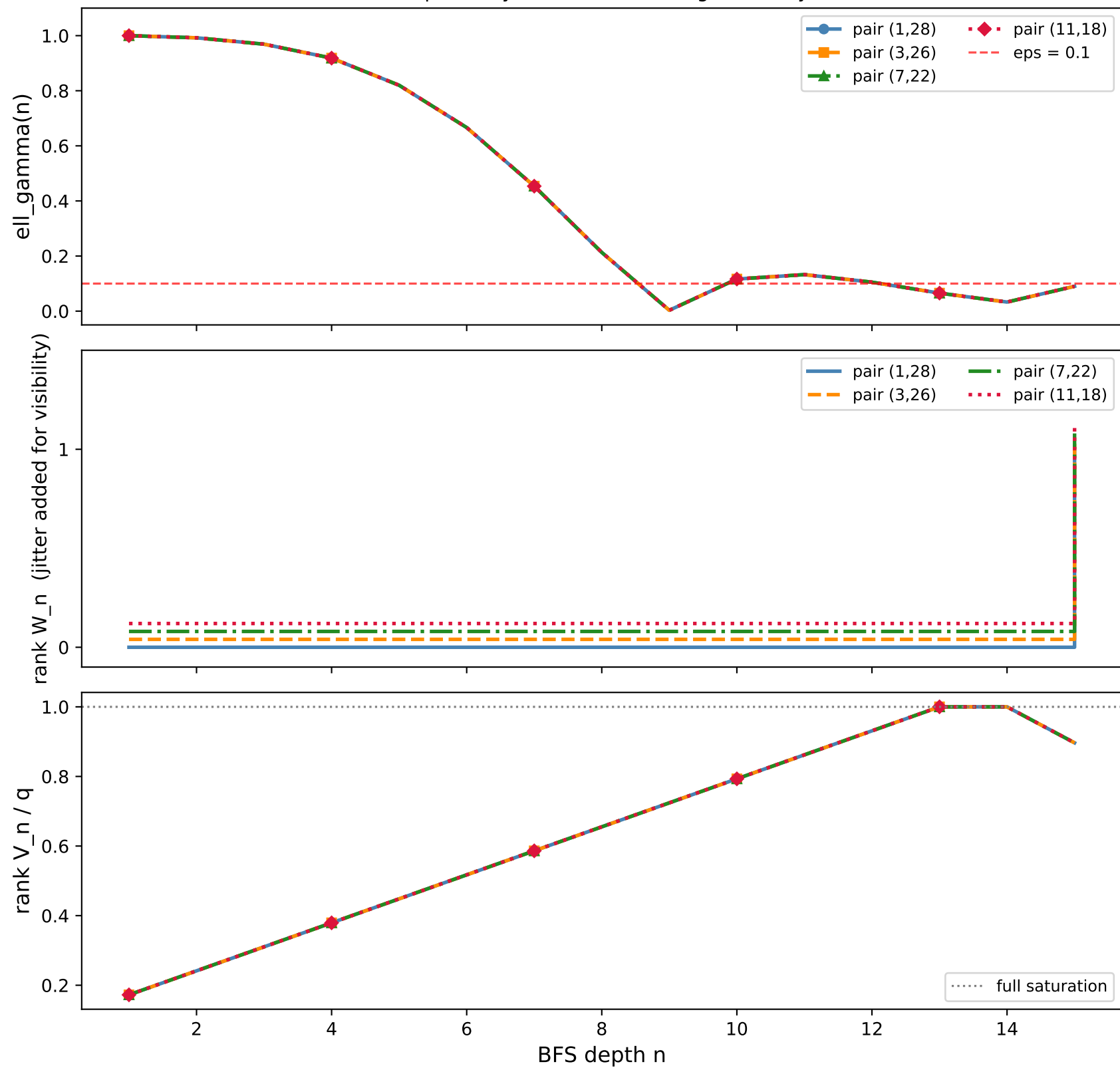
Fibre separator R_n vs coherence -- q=29 , 4 conjugate pairs Curves overlap exactly: structural indistinguishability confirmed
