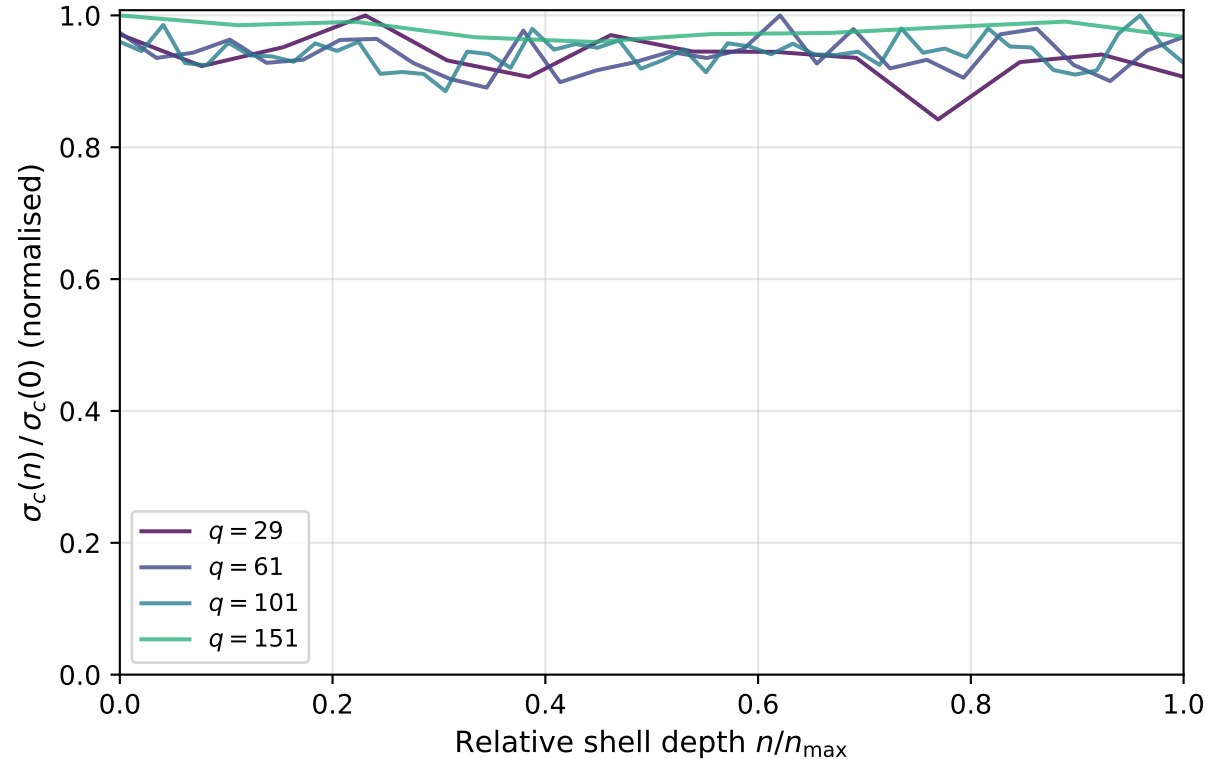
Secondary: per-shell admissibility energy \sigma_c(n)
