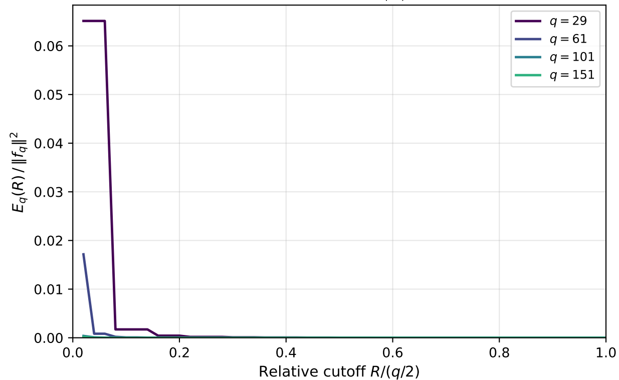
Conjecture C: spectral tail of \Pi_q g_q (Gaussian test)
