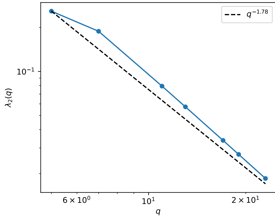
Global gap closure
