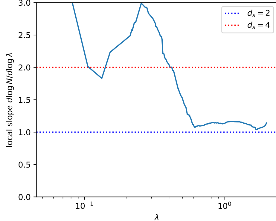
Sliding spectral dimension ( q=19 )
