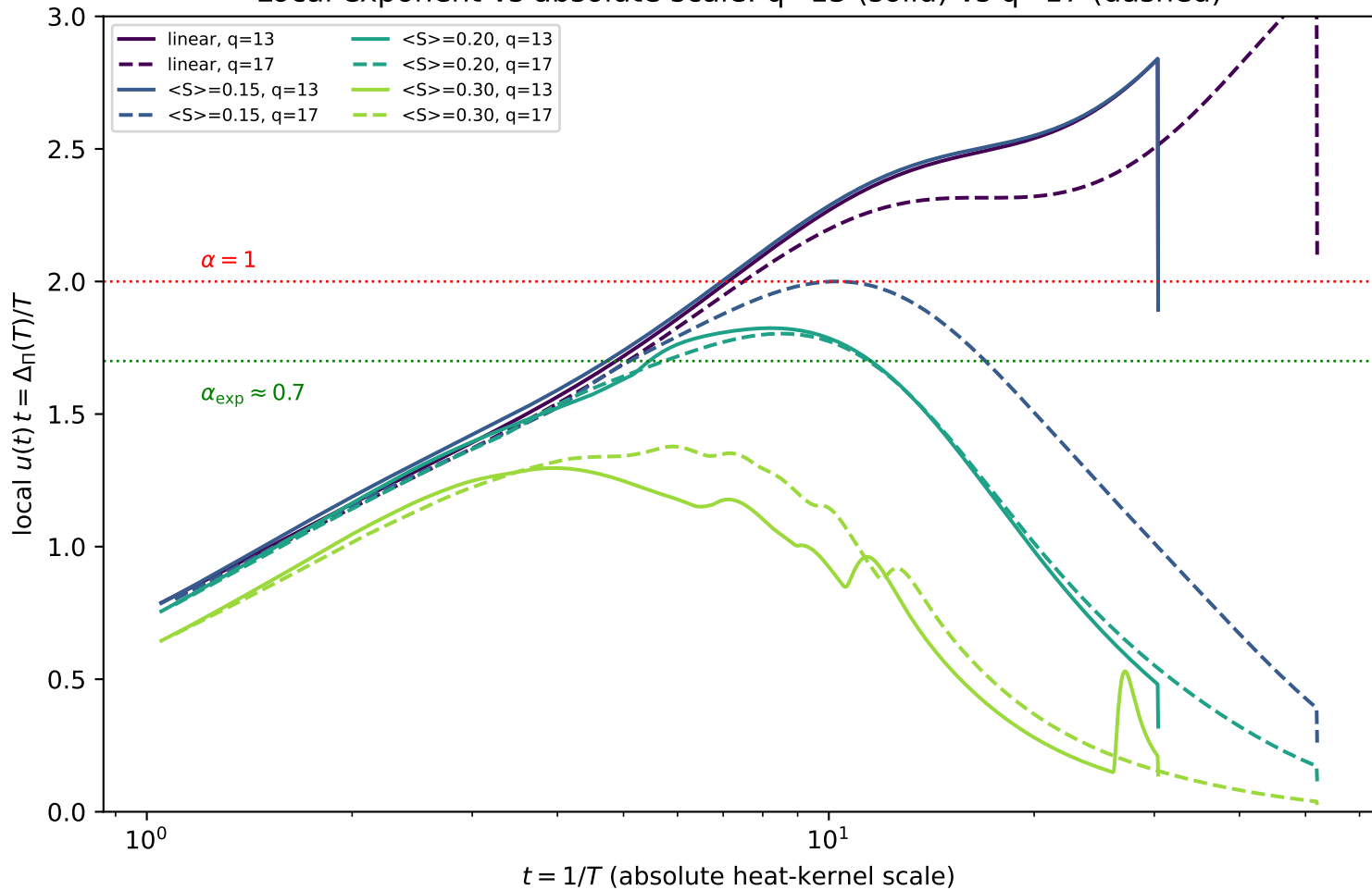
Local exponent vs absolute scale: q=13 (solid) vs q=17 (dashed)
