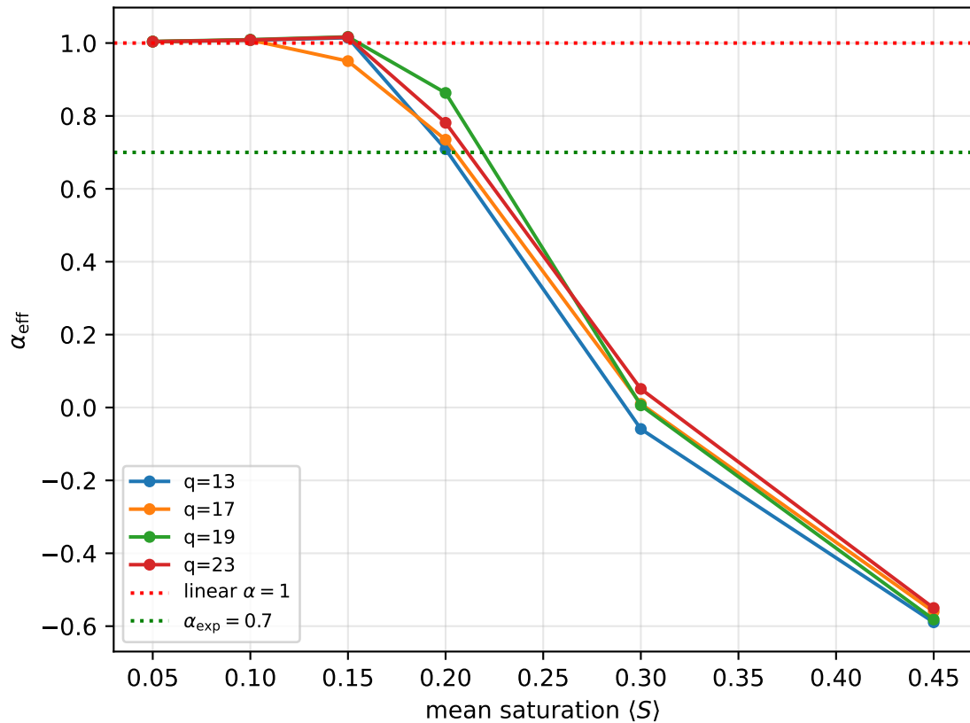
BI exponent vs saturation (window t=(6.0, 12.0) )
