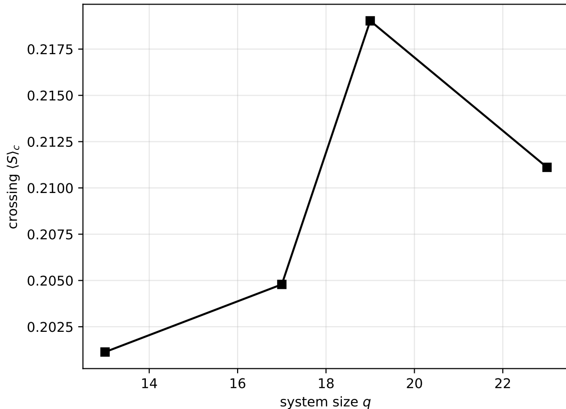
q-stability of the \alpha = 0.7 crossing
